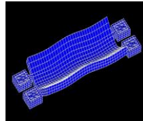
MEMS resonator
