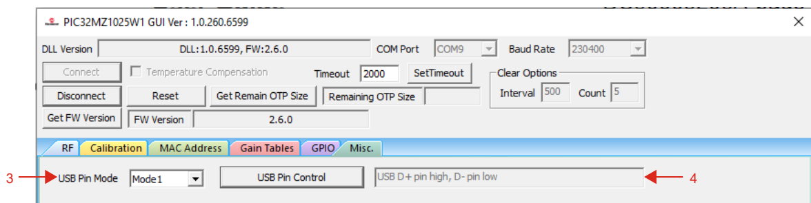
Figure 3-26. Mode1 USB Pin Control
