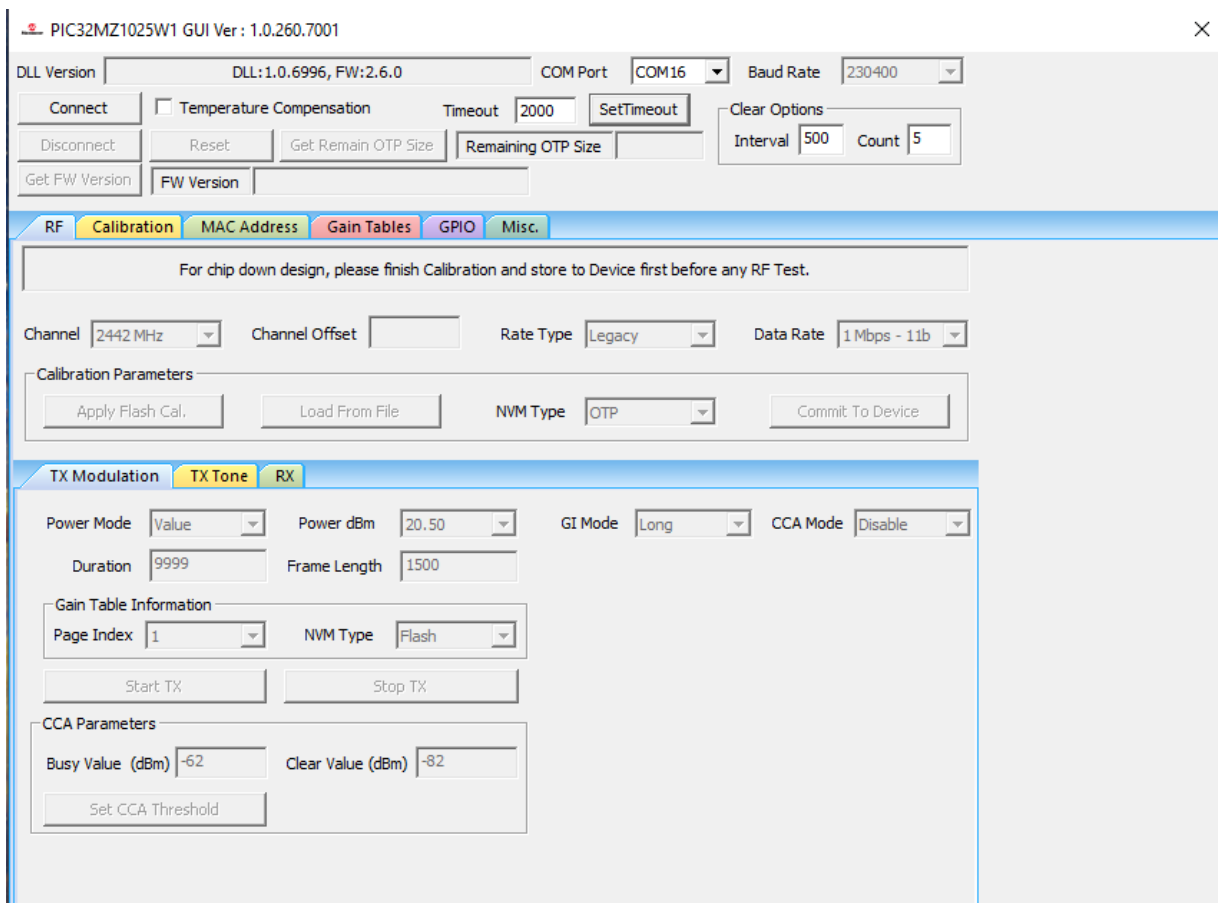
Figure 3-6. Start-Up Window of the PIC32MZ1025W1 GUI Tool
