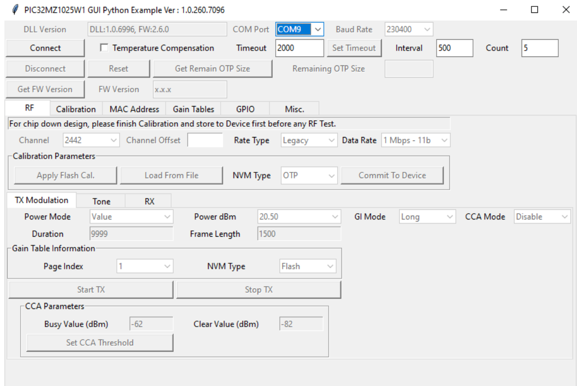
Figure 3-39. PIC32MZ1025W1 GUI Python Example
