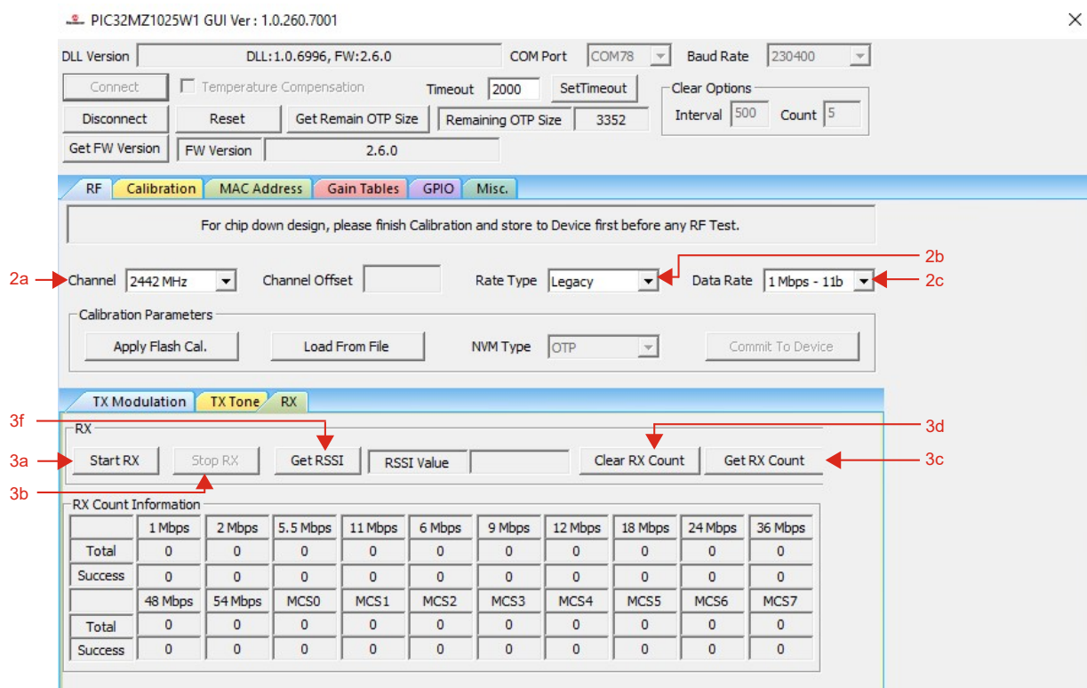
Figure 3-17. MCHPRT3 PIC32MZ1025W1 GUI for RF RX Test Demonstration
