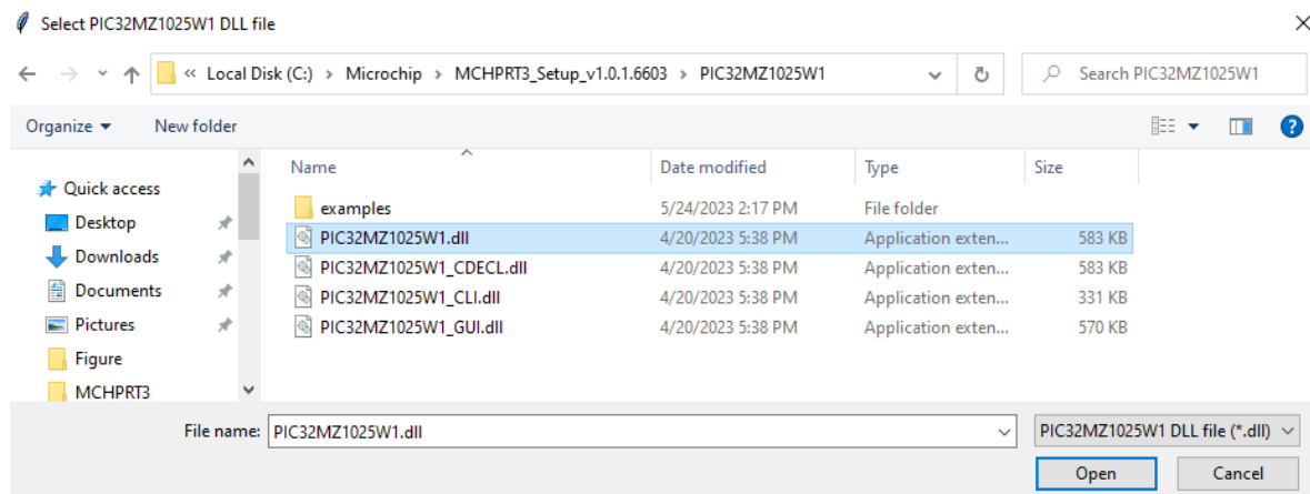
Figure 3-37. Opening PIC32MZ1025W1.dll
