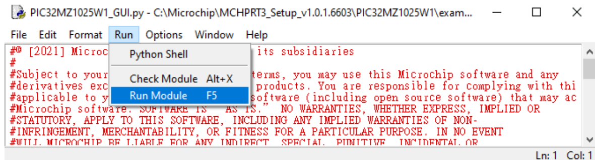
Figure 3-35. Run Module
