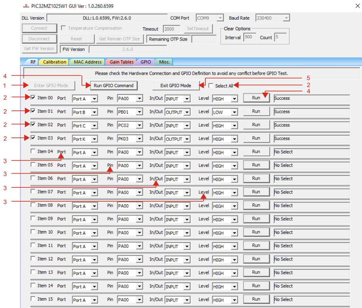
Figure 3-24. MCHPRT3 PIC32MZ1025W1 GUI GPIO Demonstration
