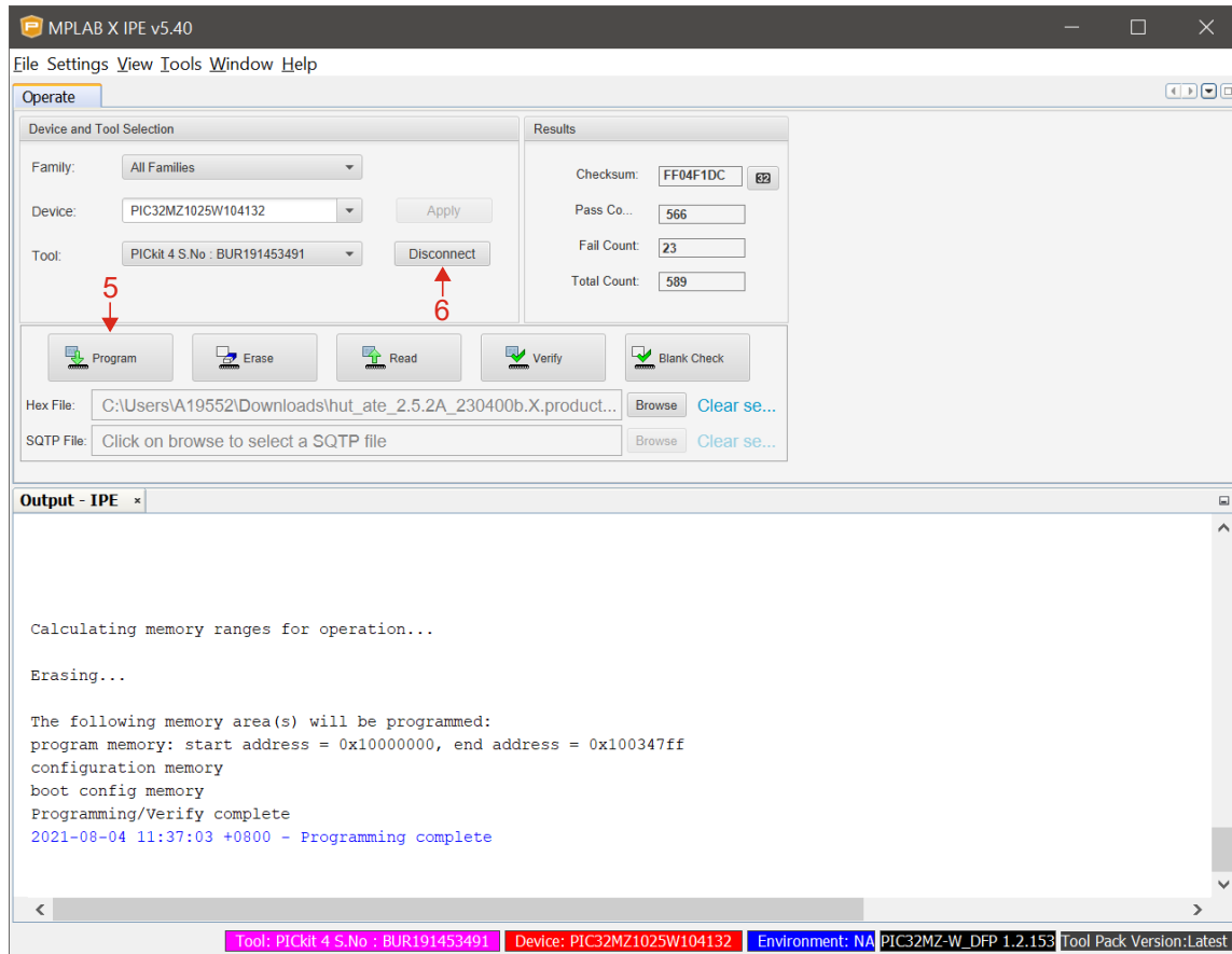
Figure 3-3. MPLAB X IPE – Programming Complete
