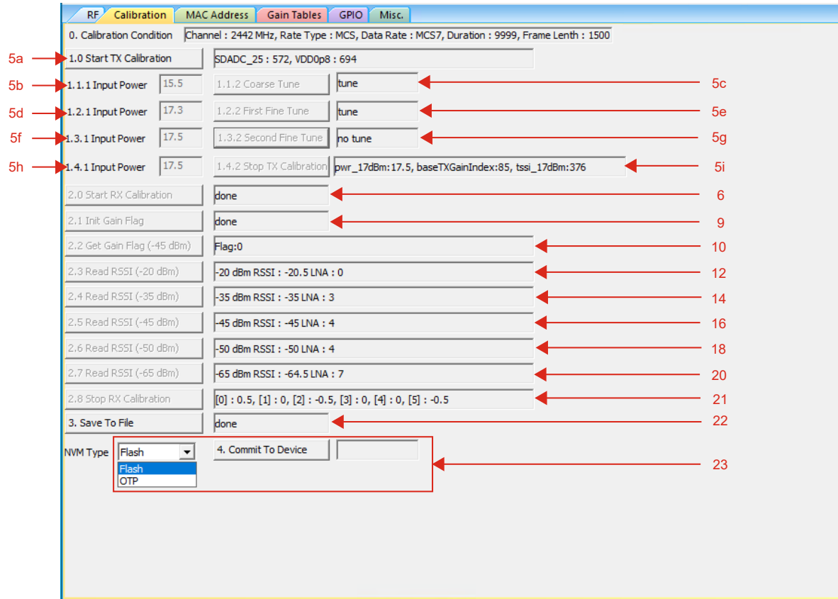
Figure 3-19. MCHPRT3 PIC32MZ1025W1 GUI for Calibration Flow Demonstration
