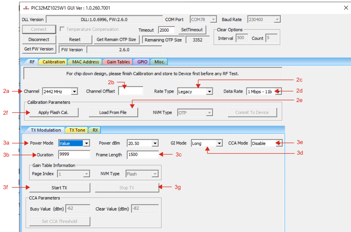
Figure 3-14. MCHPRT3 PIC32MZ1025W1 GUI for RF TX Modulation Test Demonstration
