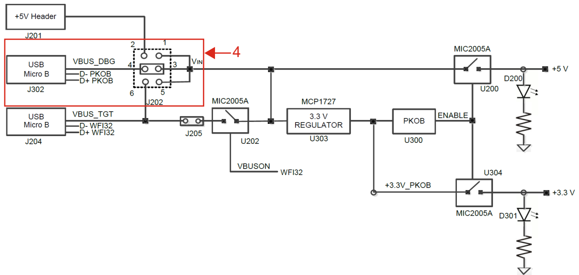
Figure 3-8. Power Tree Diagram
