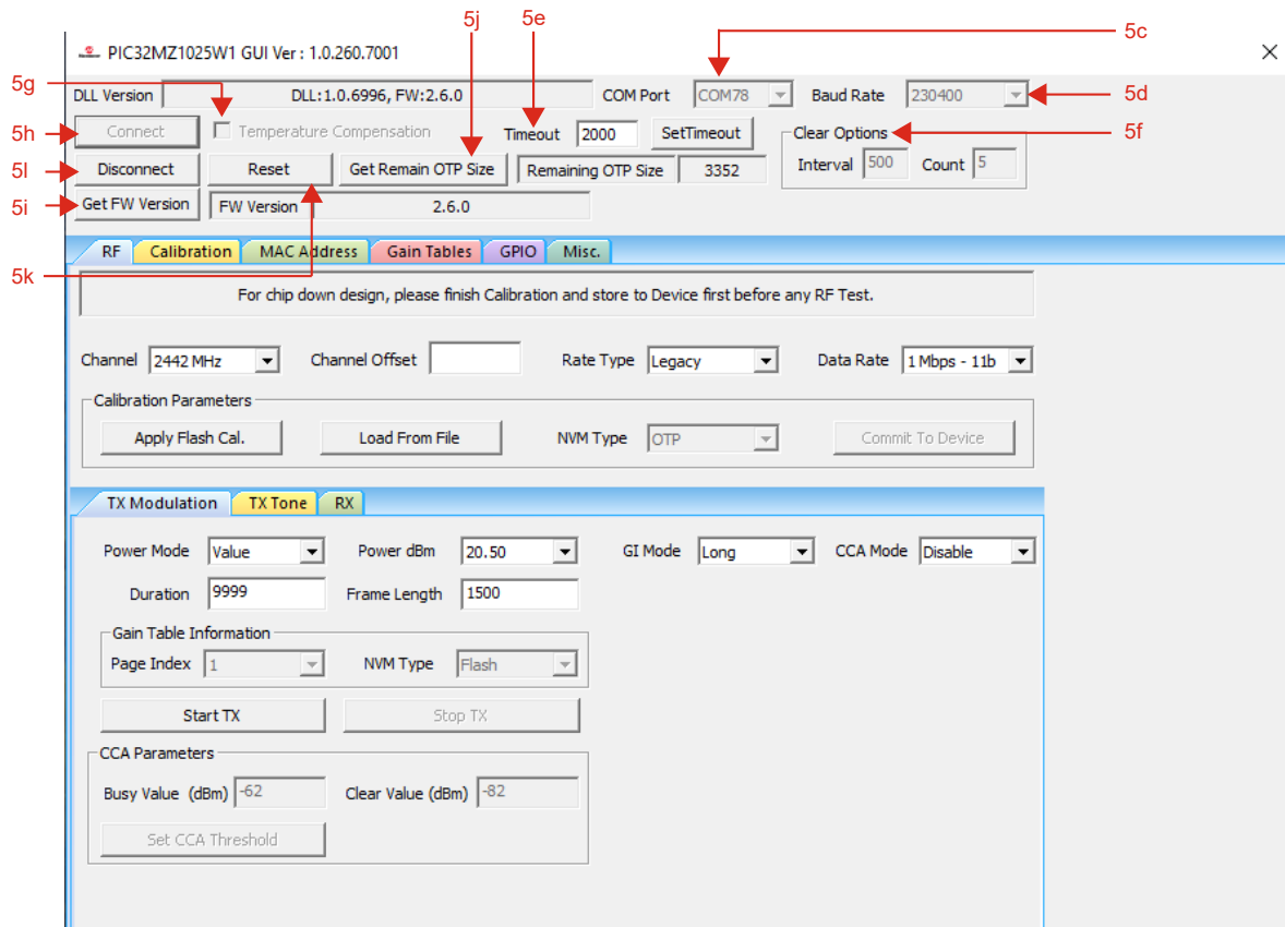
Figure 3-12. RF Test on PIC32 WFI32E Curiosity Board with MCHPRT3 Tool
