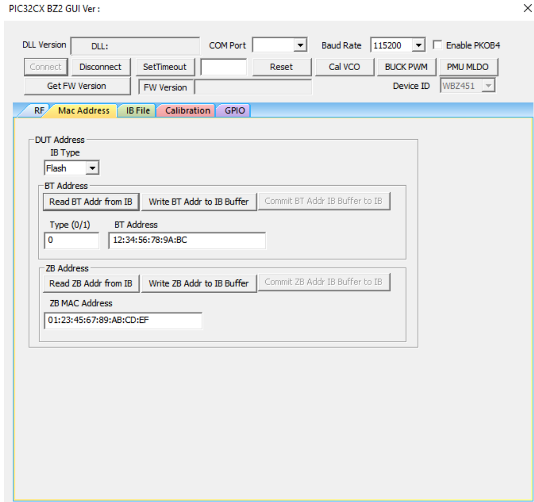
Figure 4-18. MCHPRT3 PIC32CX-BZ2 GUI for MAC Address Programming
