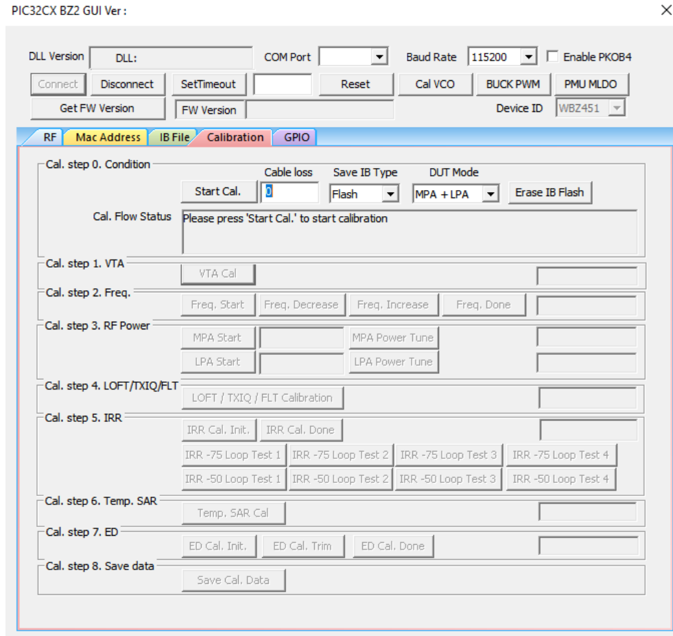
Figure 4-16. Calibration Setup
