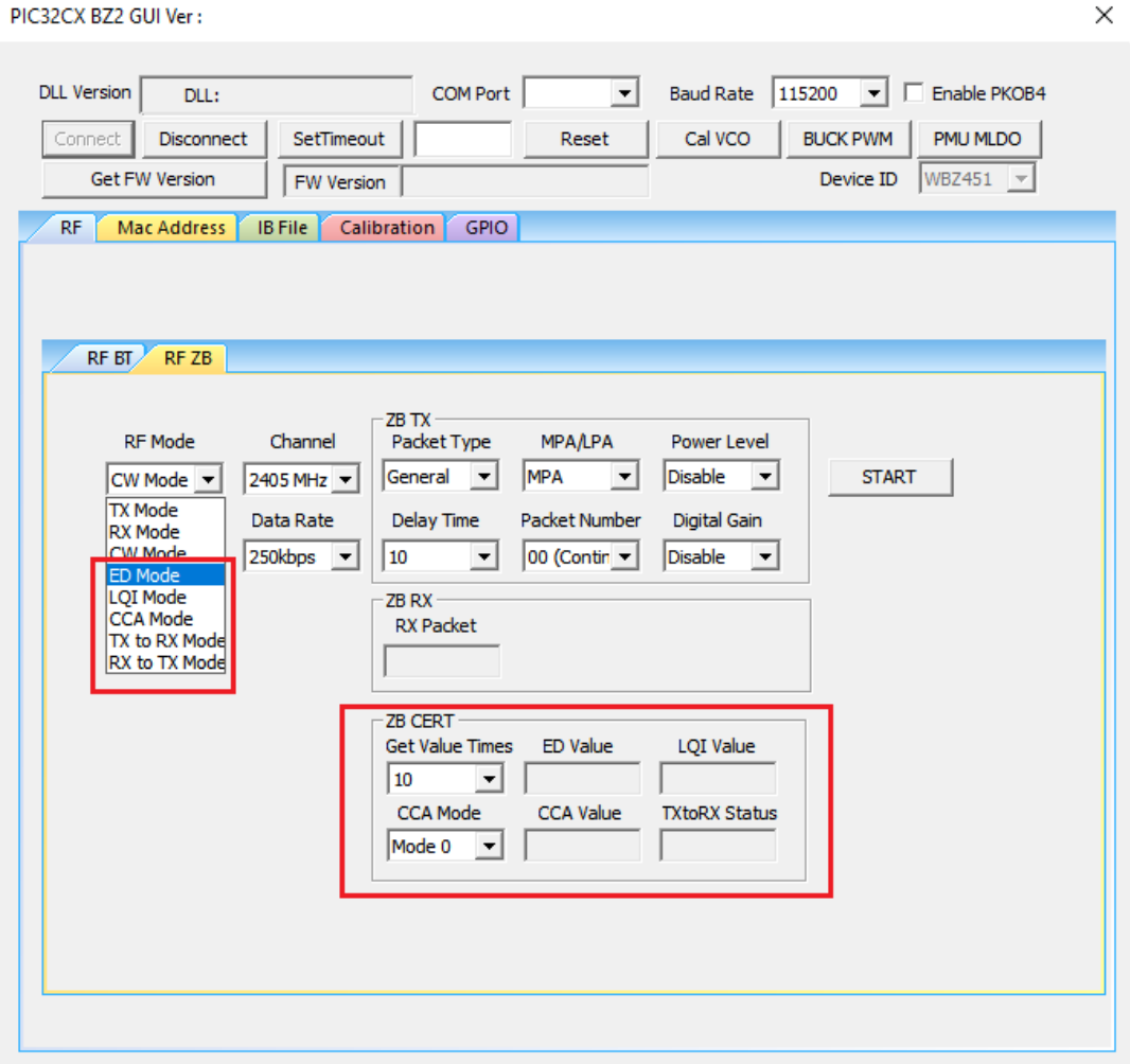
Figure 4-14. MCHPRT3 PIC32CX-BZ2 GUI for Zigbee PHY Test
