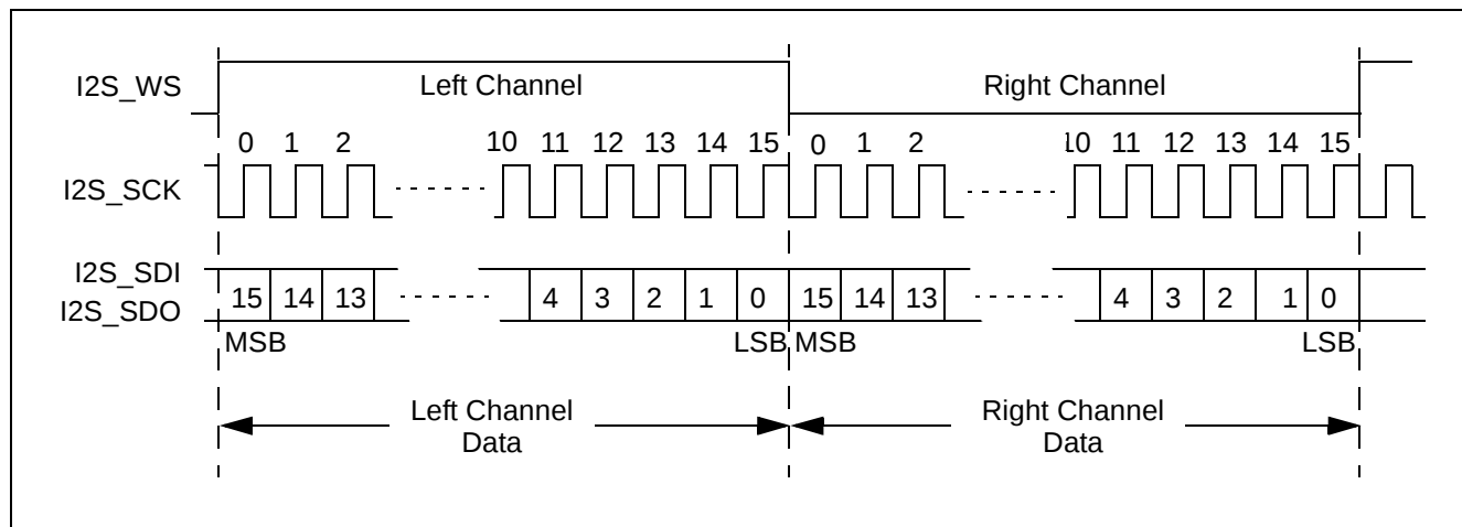
Figure 9 - Left Justified Mode
