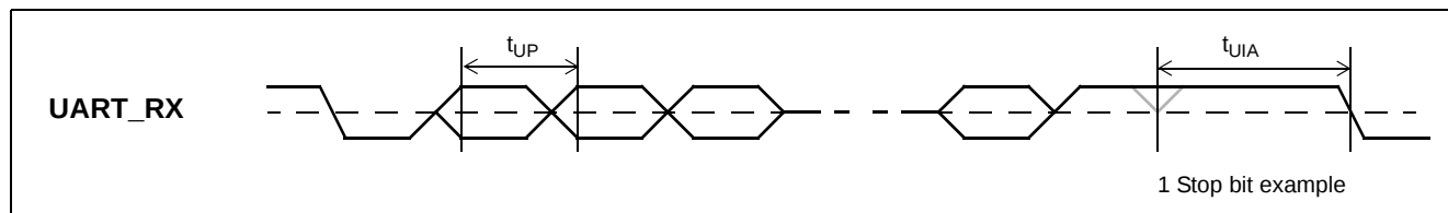
Figure 42 - UART_RX Timing
