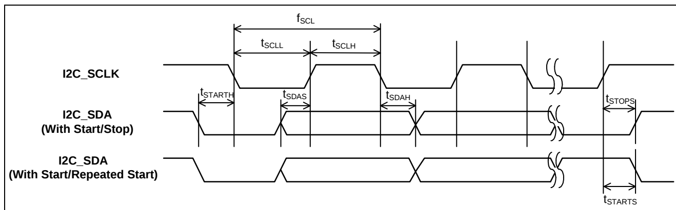
Figure 41 - I²C Timing Parameter Definitions
