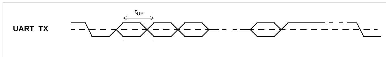
Figure 43 - UART_TX Timing
