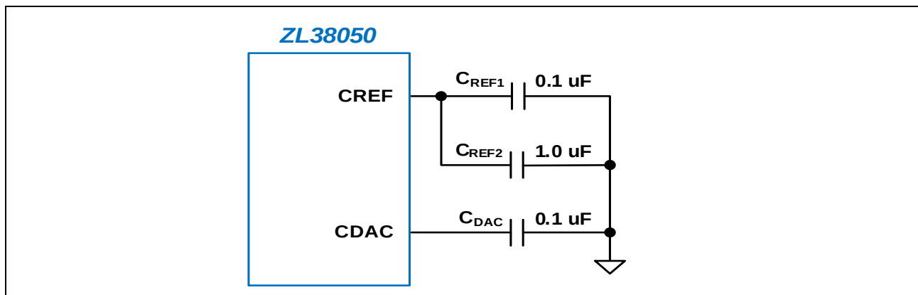
Figure 6 - ZL38050 Bias Circuit
