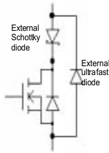
Fig. 21. Avoiding body-diode conduction with current-steering diodes.
