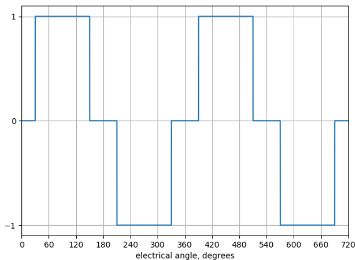
Figure 18: Typical six-step current waveform
