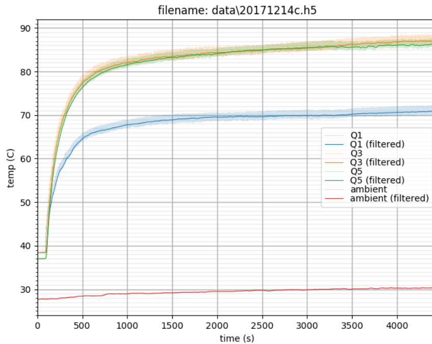
Figure 6: Graph of thermocouple readings during current rating test
