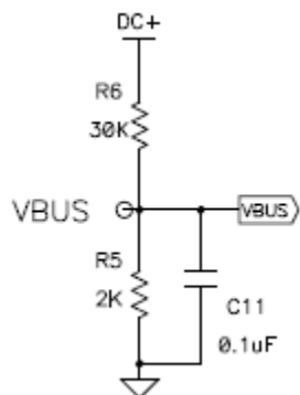
Figure 12: MCLV-2 DC link voltage sensing (excerpt from the dsPICDEM™ MCLV-2 Development Board User's Guide, DS52080A page 37)
