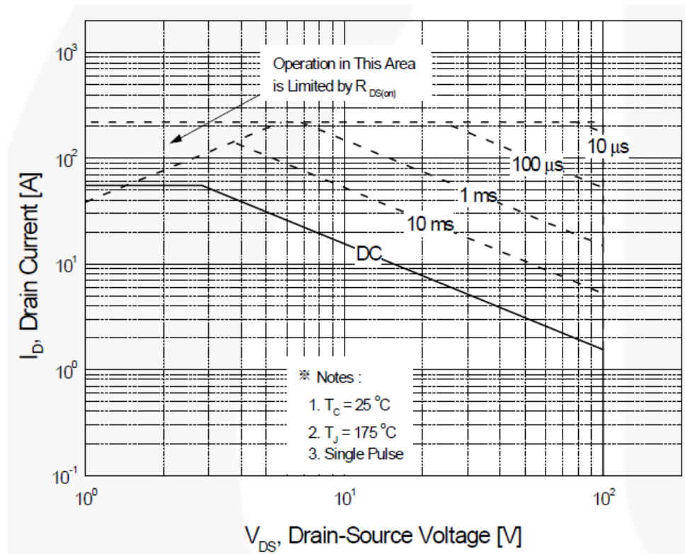
Figure 8: ON Semiconductor FQB55N10 single-pulse safe operating area graph (Figure 9 from datasheet)
