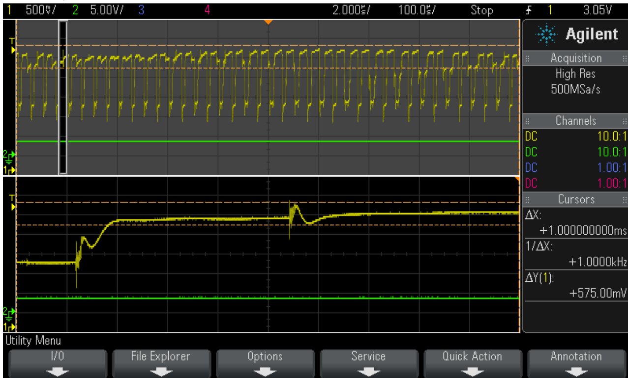
Figure 11: short switching transients in the DC link current ("IBUS") signal
