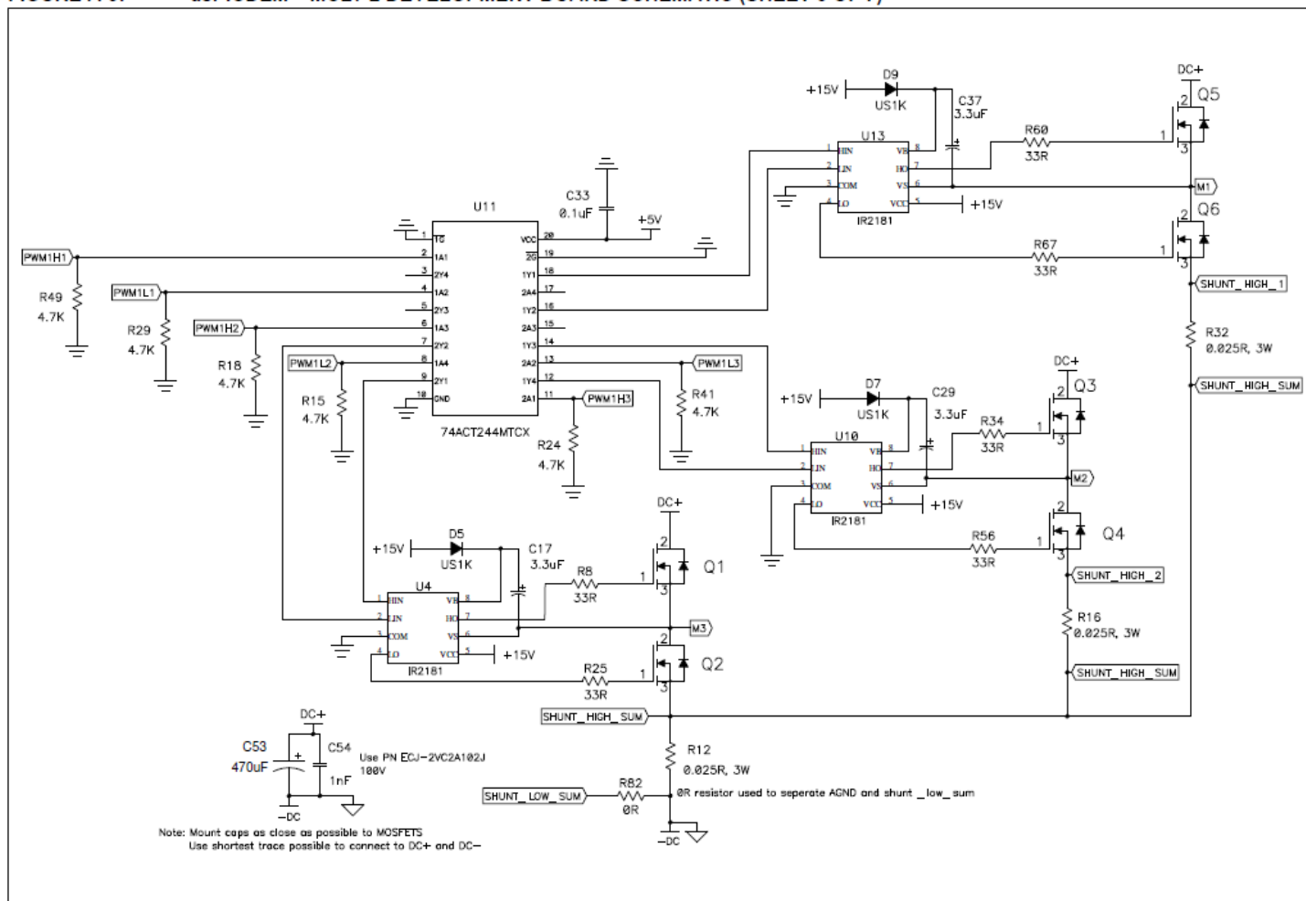
Figure 13: MCLV-2 components affected by Vdc (excerpt from the dsPICDEM™ MCLV-2 Development Board User's Guide, DS52080A page 34)
