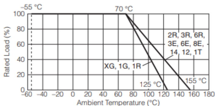
Figure 16: ERJ series chip resistor, power derating
