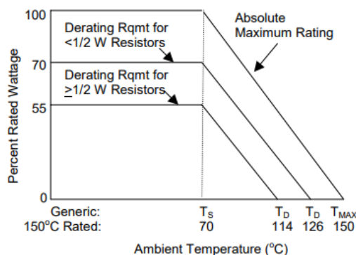
Figure 15: Resistor power derating criteria, for fixed-value film chip resistors, from US Navy SD-18
