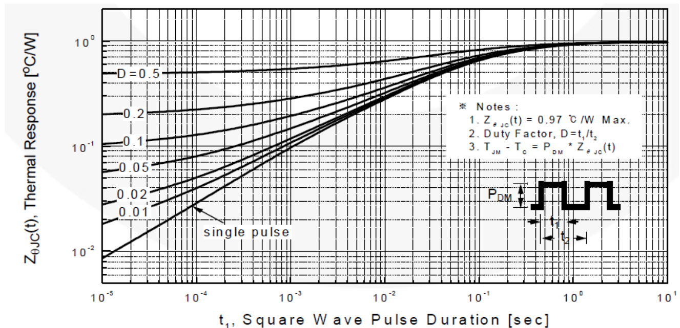
Figure 9: ON Semiconductor FQB55N10 transient thermal response curve graph (Figure 11 from datasheet)
