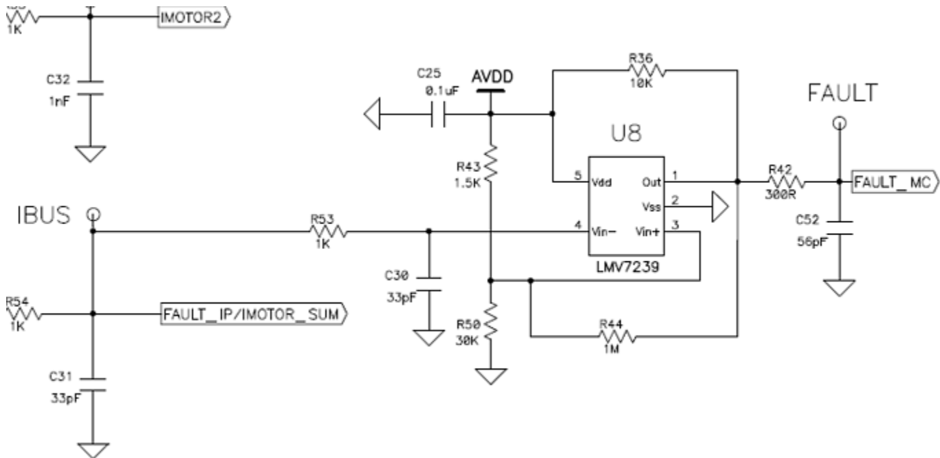
Figure 10: MCLV-2 overcurrent trip circuitry (excerpt from the dsPICDEM™ MCLV-2 Development Board User's Guide, DS52080A page 33)
