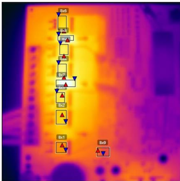
Figure 7: Thermal camera picture at end of current rating test
