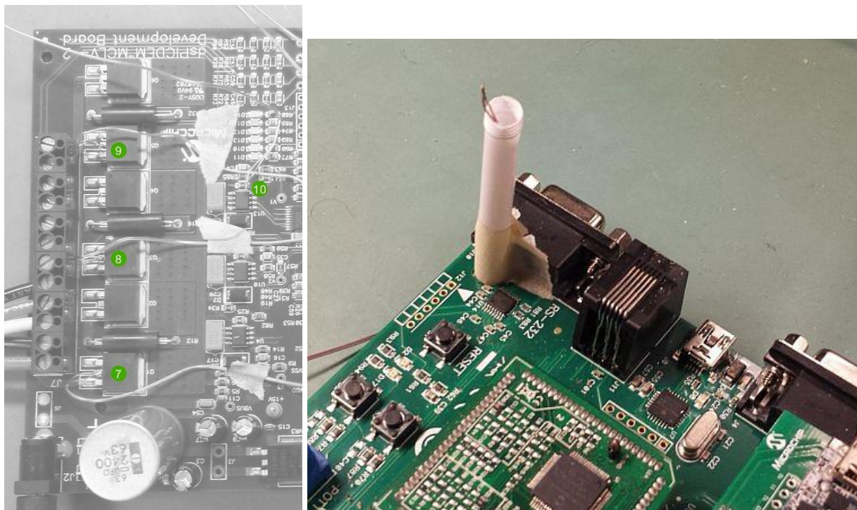
Figure 5: Thermocouple setup. Items shown in left picture are (7), (8), (9): type T thermocouples soldered to drain pins of Q1, Q3, Q5, and in right picture is a fourth type T thermocouple measuring ambient temperature near the MCLV-2 board.
