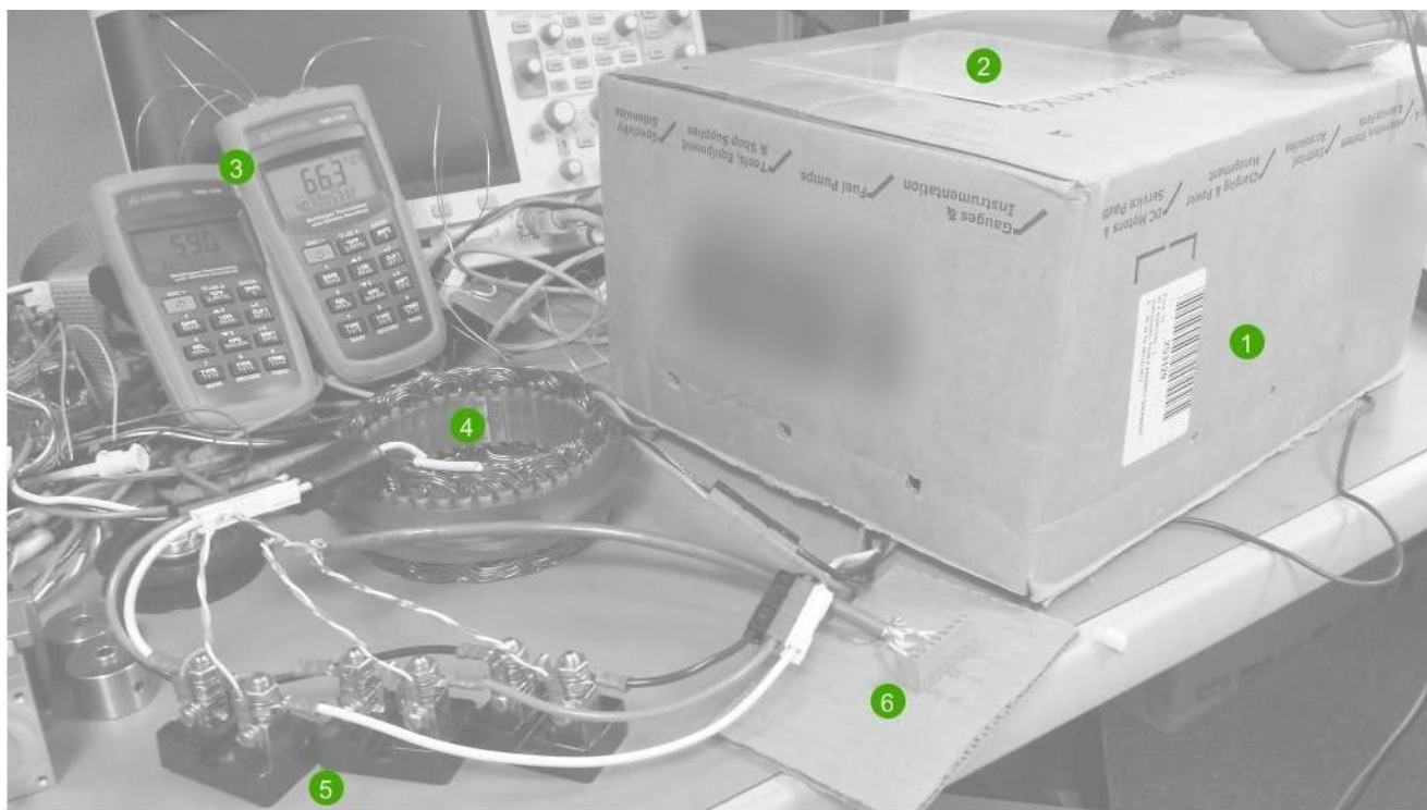
Figure 4: Test setup for determining thermal rating of MCLV-2 board. Numbered items shown are (1) cardboard box to act as a shield from unwanted convection currents, (2) IR-translucent window for thermal camera observation (this ended up not working well, and we moved the window halfway-open to allow observation using the thermal camera, but reduce the risk of unwanted convection currents), (3) TMD-55W thermocouple meters, (4) 24V alternator stator, (5) laboratory shunts, (6) terminal block for measuring Kelvin connections on shunts
