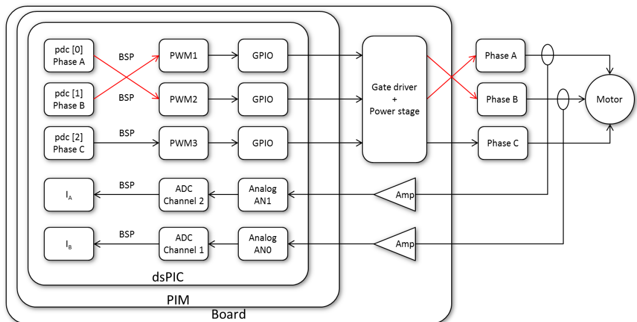
Figure 3: Custom board with crisscrossed PWM channel to motor phase mapping
