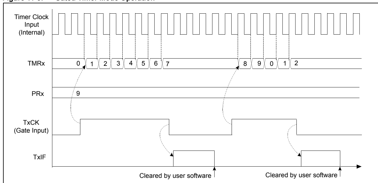
Figure 11-5: Gated Timer Mode Operation
