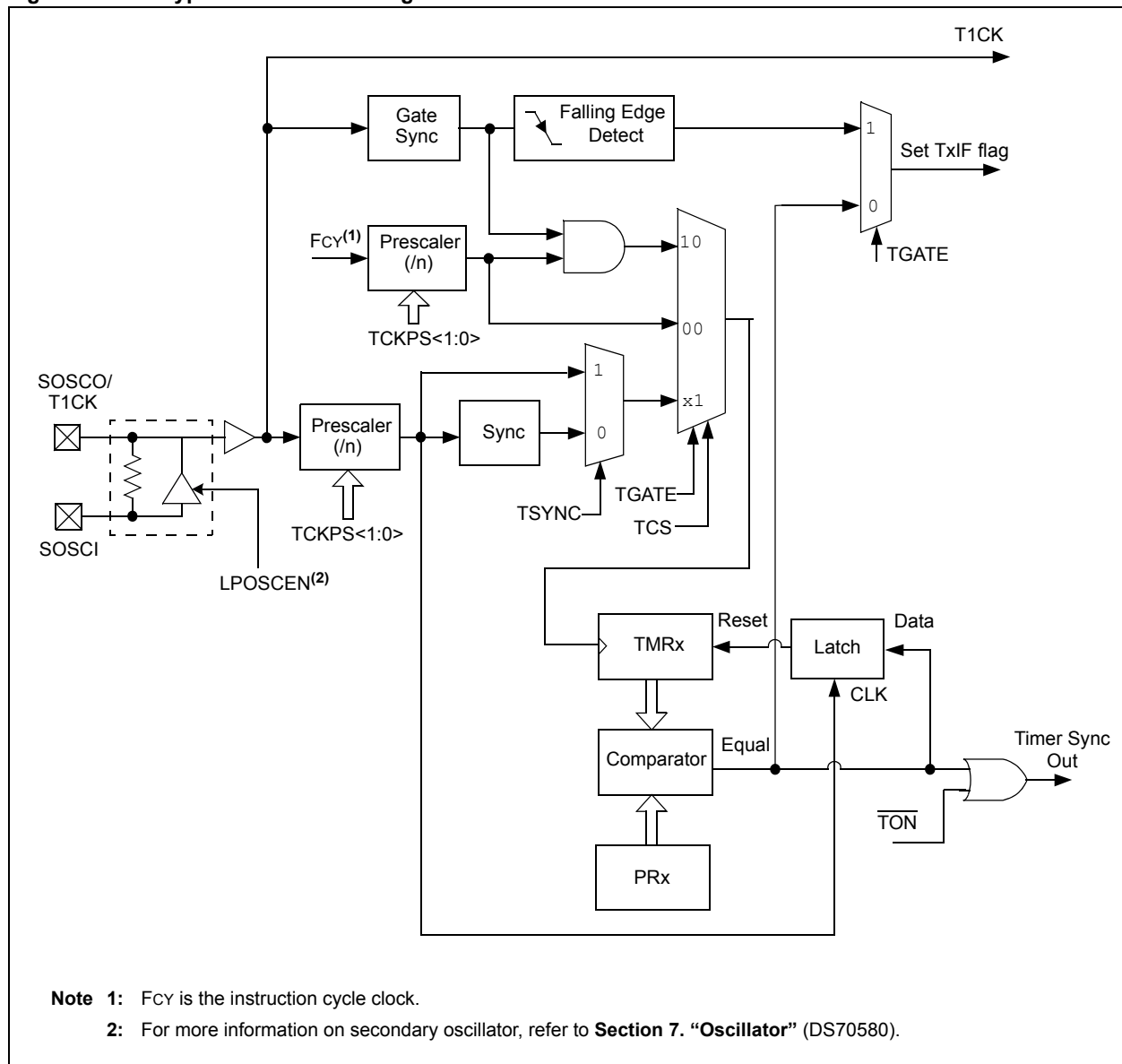
Figure 11-1: Type A Timer Block Diagram
