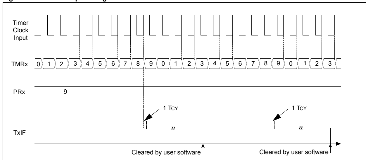
Figure 11-4: Interrupt Timing for Timer Period Match
