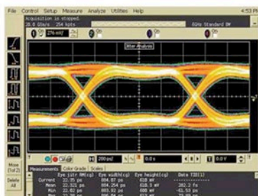
Symwave's 1394b Eye-Diagram
