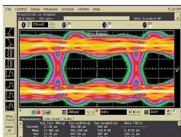
Competitor's 1394b Eye-Diagram
