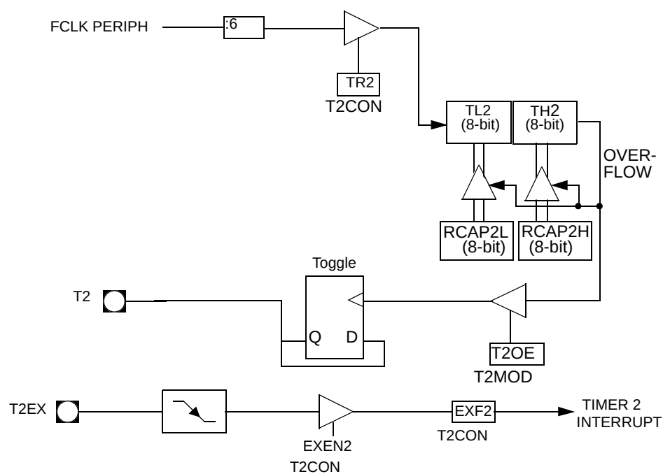
Figure 13. Clock-Out Mode C/\overline{T2} = 0
