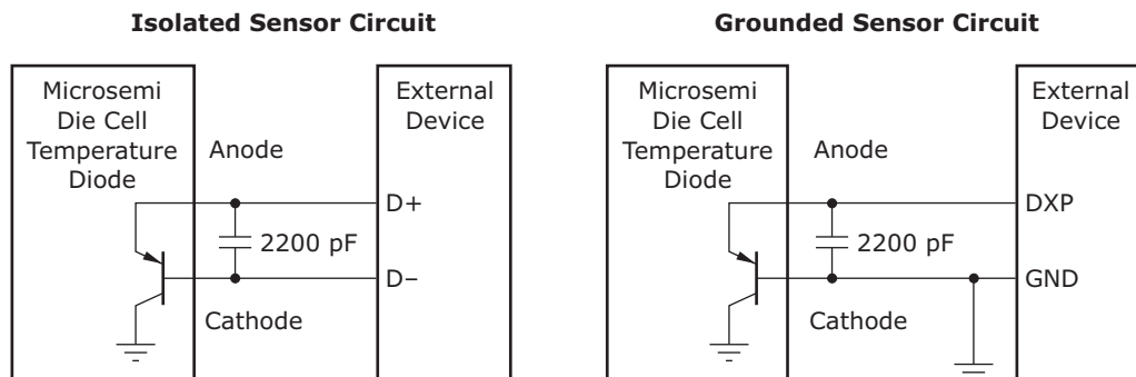
Figure 90 • Thermal Diode
