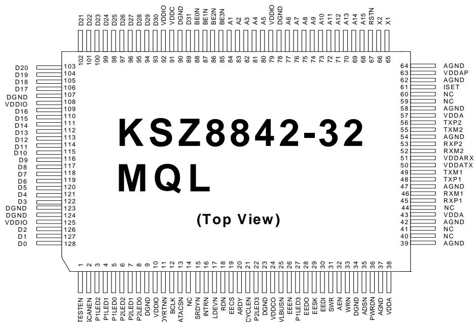
Figure 4. Standard – KSZ8842-32 MQL 128-Pin PQFP (Top View)
