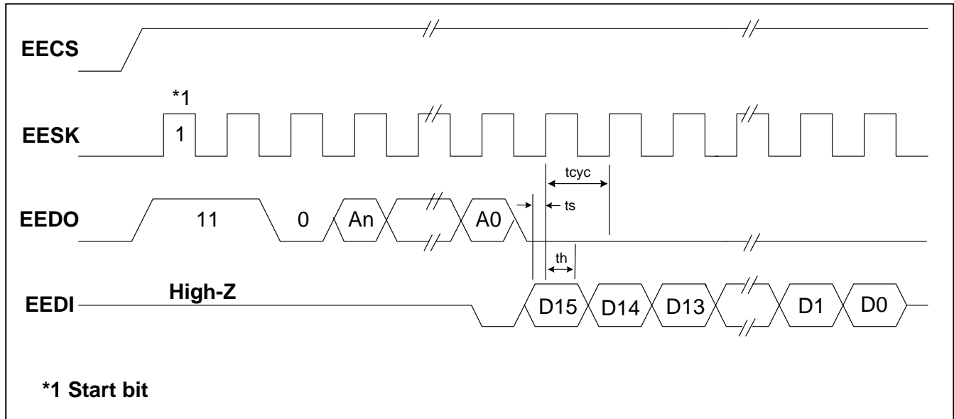
Figure 24. EEPROM Read Cycle Timing Diagram
