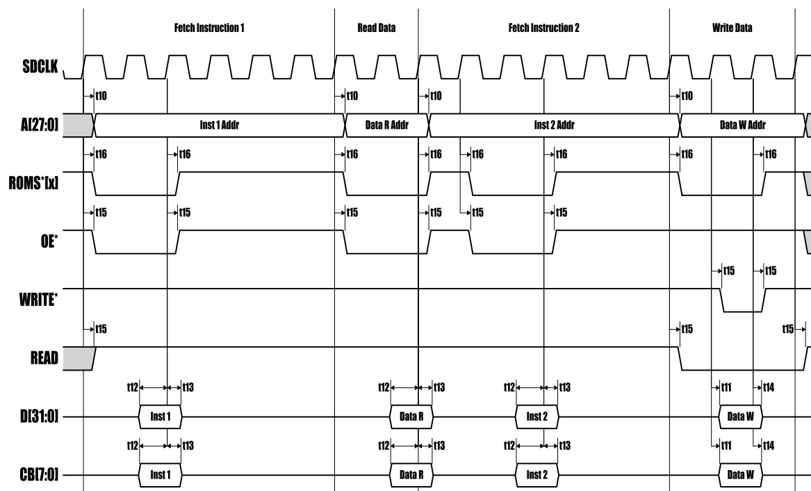
Figure 17-14. Fetch, Read and Write from 32-bit PROM 2n wait-states
