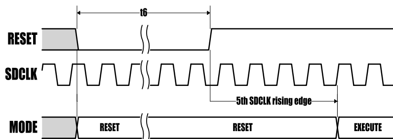
Figure 17-10. Reset Sequence
