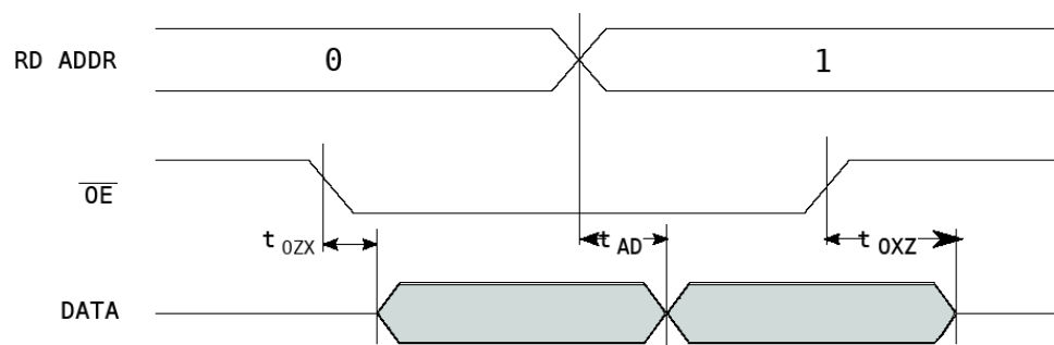
Figure 17-9. Dual-port Read
