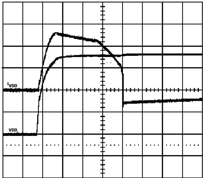
Figure 17-3. Inrush current
