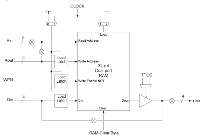
Figure 11-28. RAM logic - Detailed
