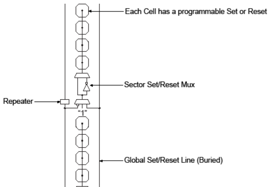
Figure 13-7. Set/Reset
