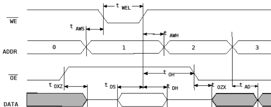
Figure 17-4. Single-port Write/Read
