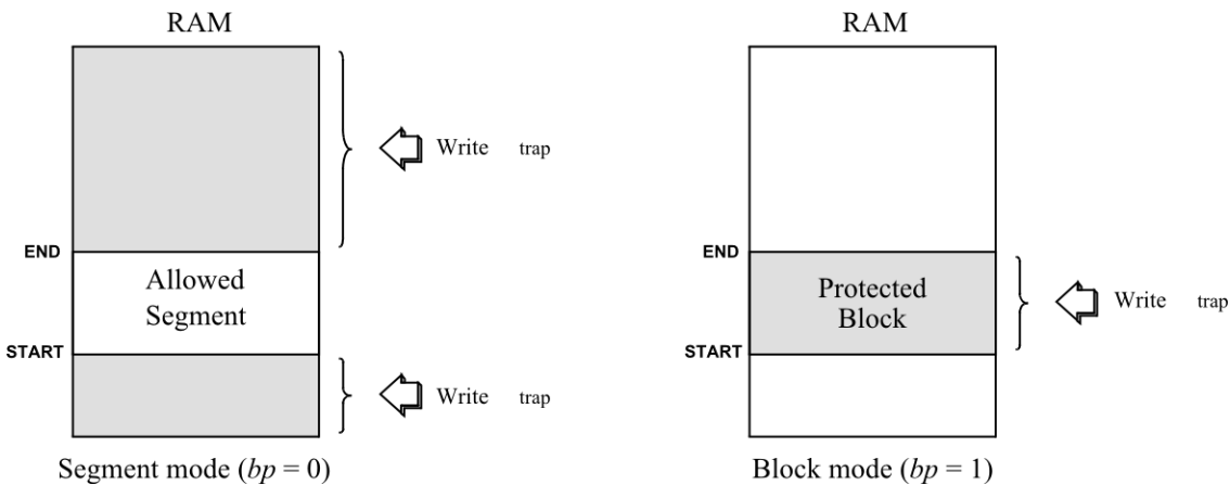
Figure 3-14. Start/End Address Scheme Protection Overview
