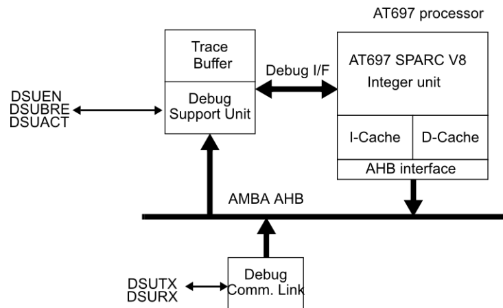
Figure 14-1. Debug Support Unit and Communication Link
