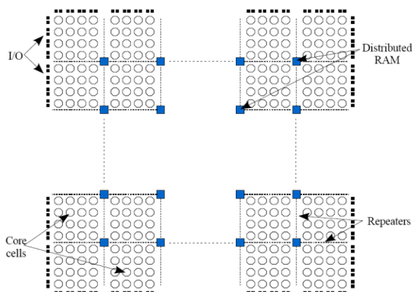
Figure 2-6. Core device overview
