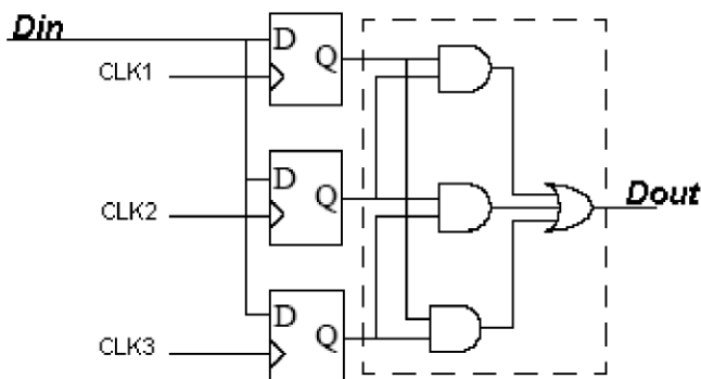
Figure 13-3. TMR structure
