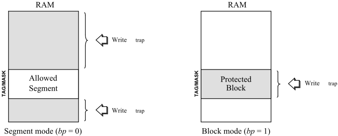
Figure 3-15. Tag/Mask Address Scheme Protection Overview
