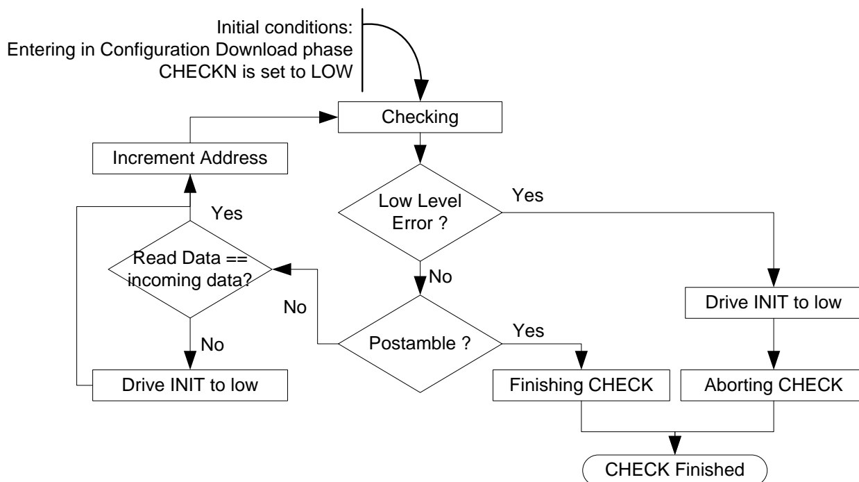
Figure 11-20. ATF697FF reconfigurable unit CHECK function workflow
