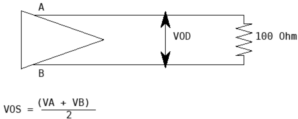
Figure 17-1. Test Termination Measurements
