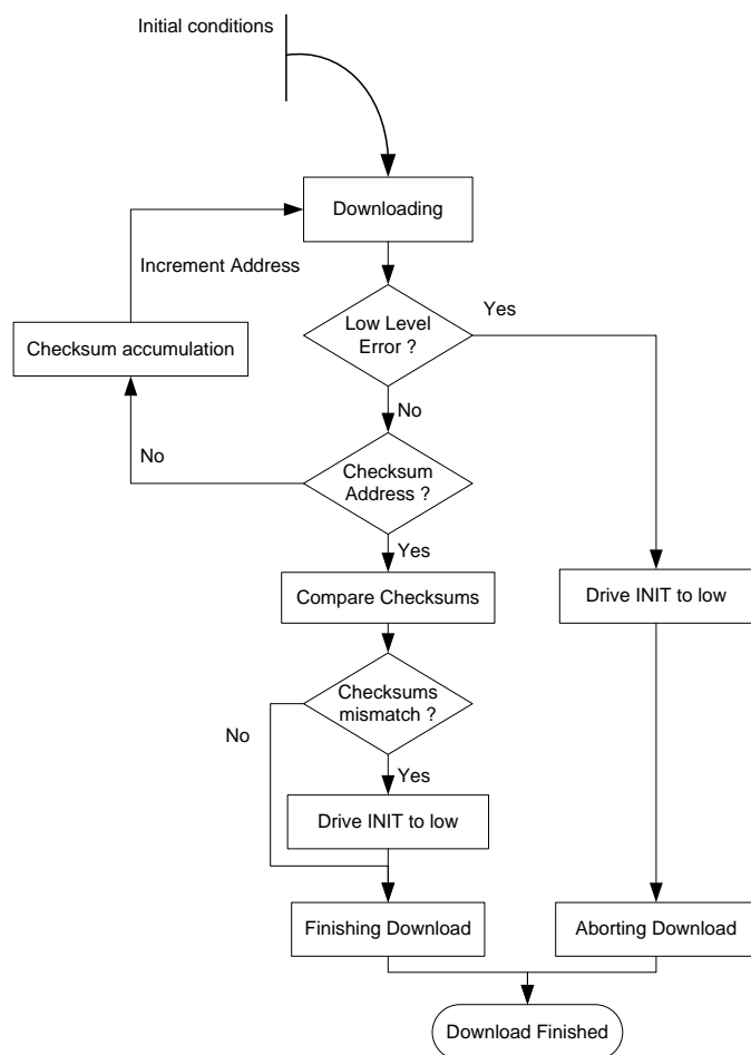
Figure 11-16. Management of configuration download link protection
