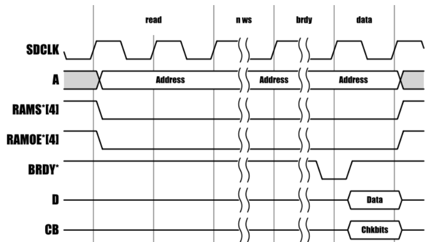
Figure 3-22. Asynchronous BRDY* -Controlled SRAM4 Read Access (MCFG1.abrdy=1)
