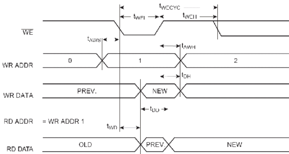
Figure 17-6. Dual-port Read
