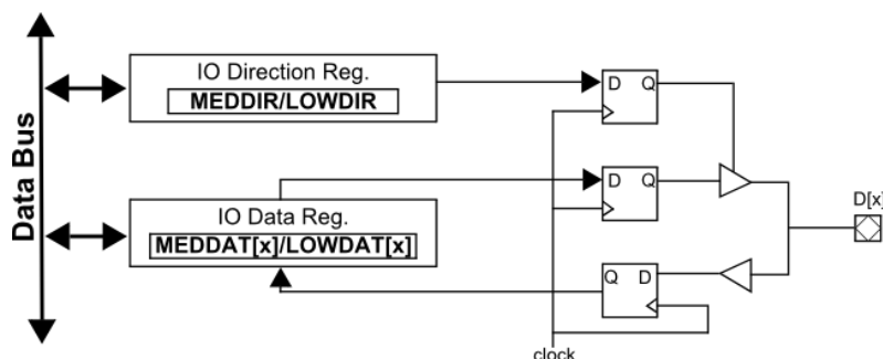
Figure 10-2. I/O Port Block Diagram D[15:0]
