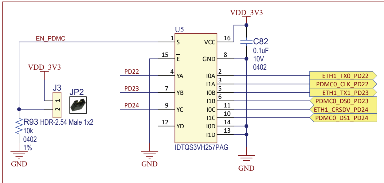
Figure 3-25. GPIO Distribution Schematic
