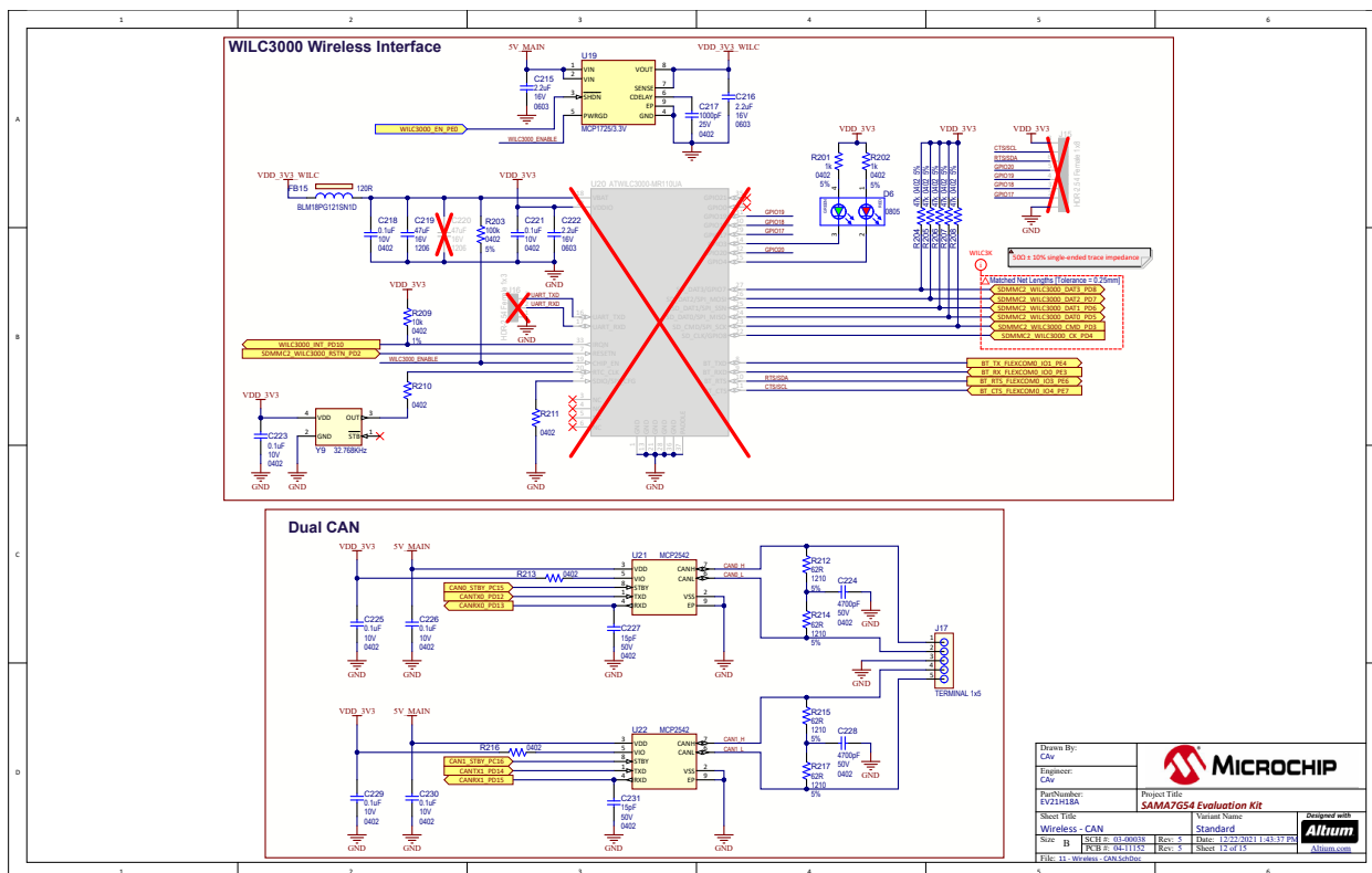
Figure 6-12. SAMA7G54-EK: Schematic Page 12
