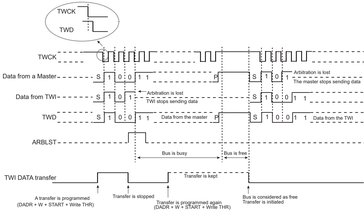
Figure 47-110. Arbitration Cases
