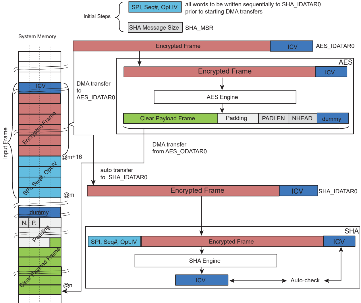
Figure 60-15. Decryption of an ESP IP Sec Frame without ESN
