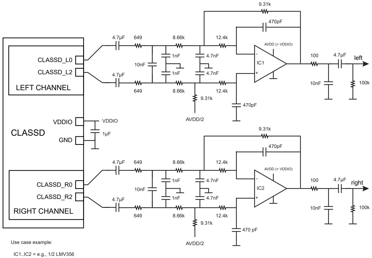
Figure 43-18. Use Case 3B: Stereo Audio DAC With Simple Passive Low-Pass Filter and Differential Outputs
