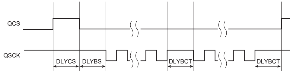
Figure 50-4. Programmable Delays
