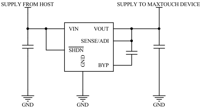
FIGURE 5-1: EXAMPLE LDO CIRCUIT
