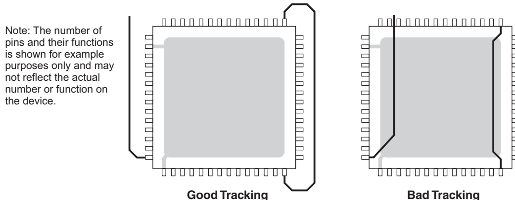
FIGURE 5-2: EXAMPLES OF GOOD AND BAD TRACKING
