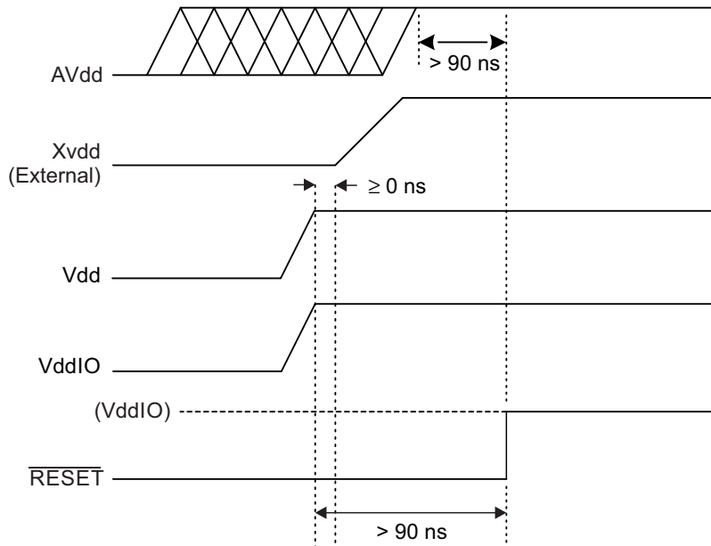
FIGURE 5-1: POWER SEQUENCING ON THE MXT1189TD-AT
