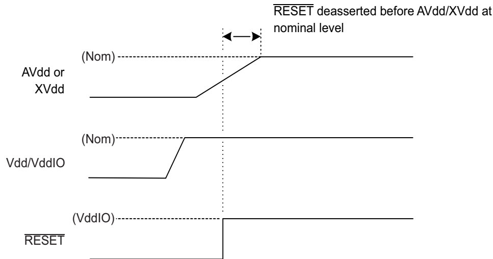
FIGURE 5-2: POWER SEQUENCING ON THE MXT1189TD-AT – LATE RISE ON AVDD OR XVDD
