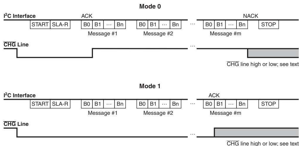
FIGURE 8-7: \overline{\text{CHG}} LINE MODES FOR I 2 C-COMPATIBLE TRANSFERS
