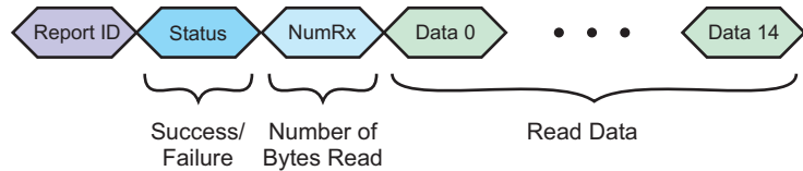
FIGURE 9-3: READ/WRITE MEMORY MAP – RESPONSE PACKET FORMAT
