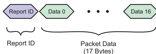
FIGURE 9-1: READ/WRITE MEMORY MAP – GENERIC PACKET FORMAT
