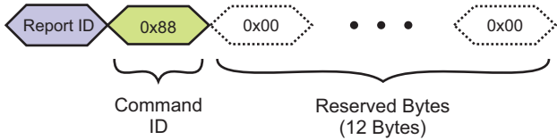
FIGURE 9-9: SEND AUTO-RETURN – COMMAND PACKET FORMAT
