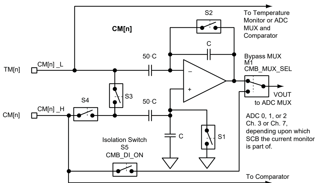
Figure 6-2 • Functional Block Diagram of Current Monitor
