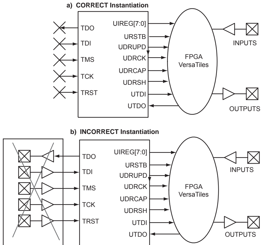
Figure 14-3 • Connectivity Method of UJTAG Macro
