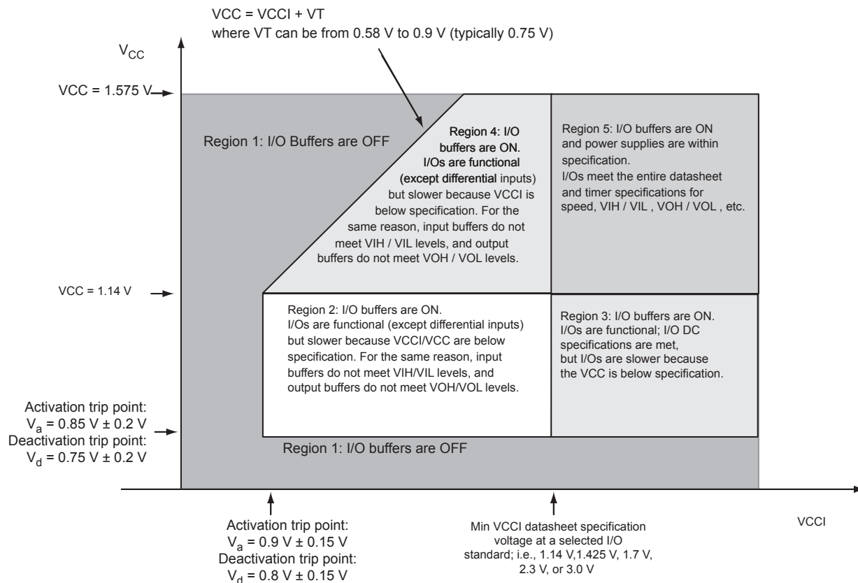
Figure 15-5 • I/O State as a Function of VCCI and VCC Voltage Levels for IGLOO V2, IGLOO nano V2, IGLOO PLUS V2, and ProASIC3L Devices Running at V_{CC} = 1.2\text{ V} \pm 0.06\text{ V}
