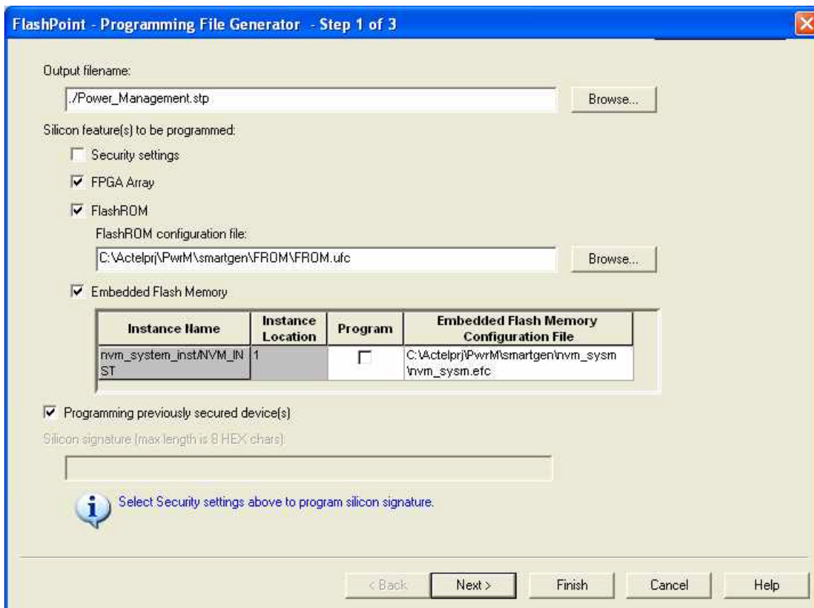
Figure 10-17 • Settings to Program a Device Secured with FlashLock and using AES Encryption
