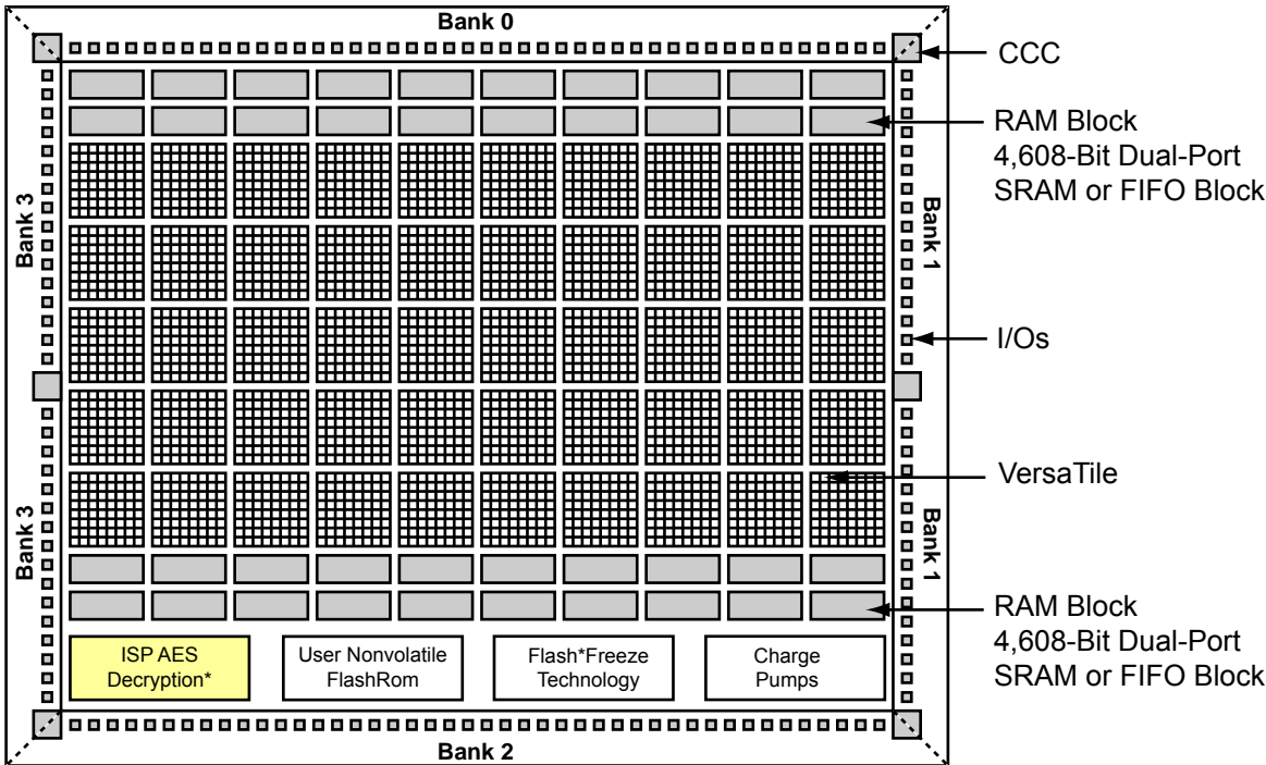
Figure 10-2 • Block Representation of the AES Decryption Core in IGLOO and ProASIC3 Devices
