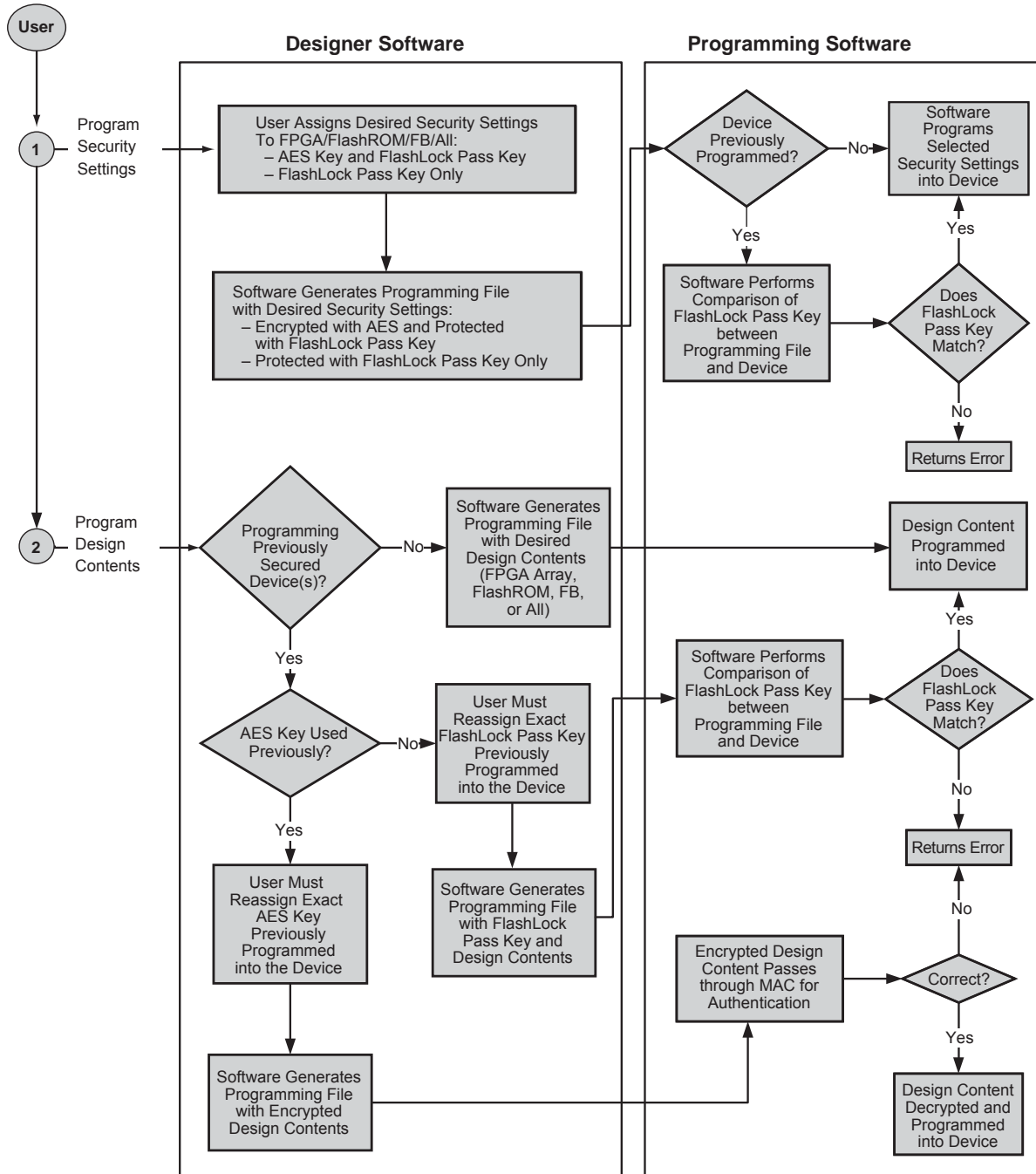
Figure 10-9 • Security Programming Flows
