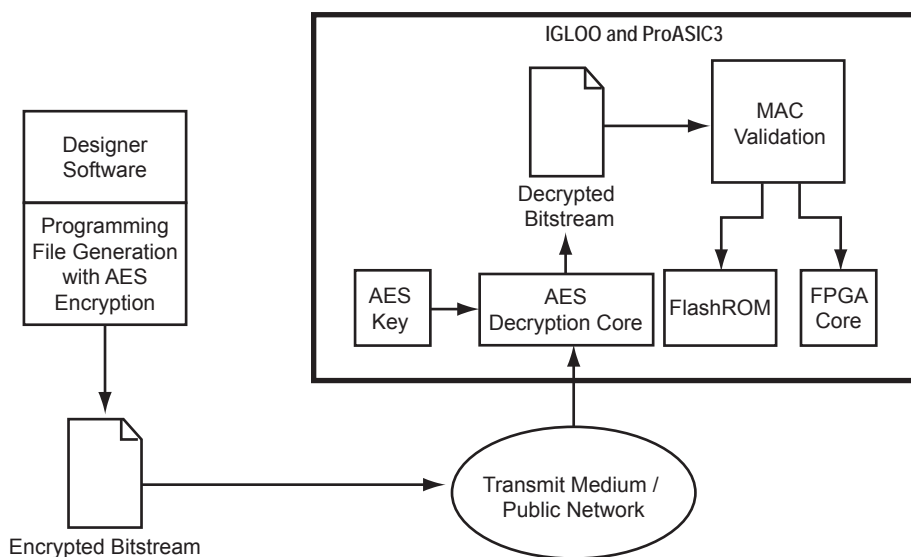
Figure 10-4 • Example Application Scenario Using AES in IGLOO and ProASIC3 Devices
