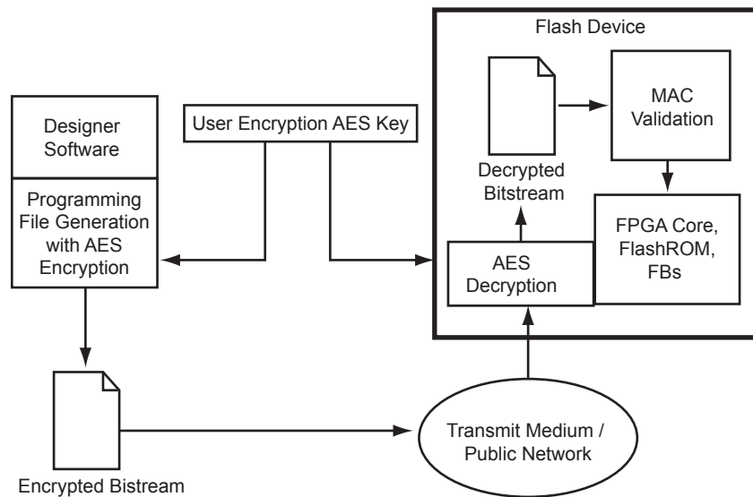
Figure 11-1 • AES-128 Security Features
