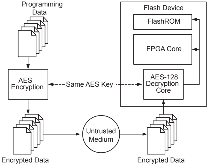
Figure 5-5 • Programming FlashROM Using AES
