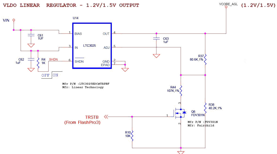
Figure 12-1 • Circuit Diagram
