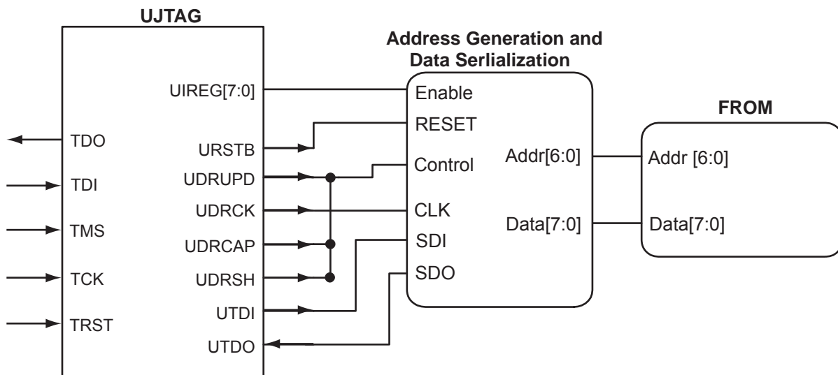
Figure 14-1 • Block Diagram of Using UJTAG to Read FlashROM Contents
