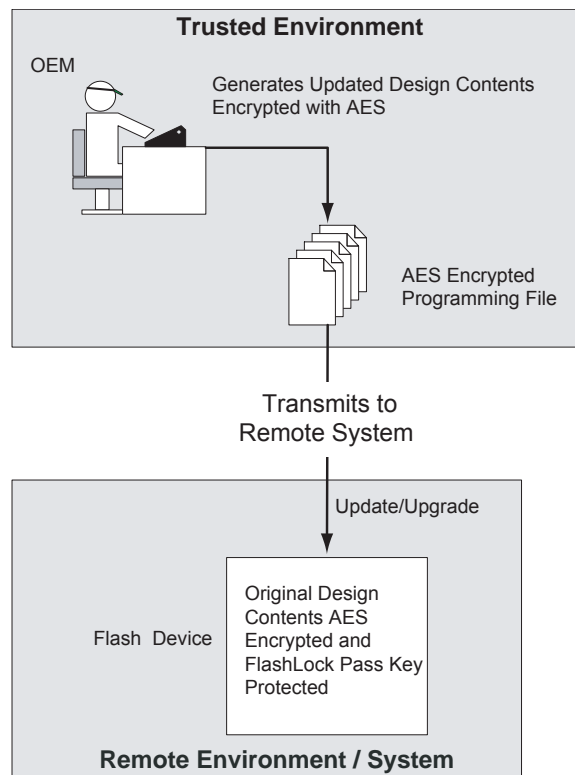
Figure 10-8 • Application 3: Nontrusted Environment—Field Updates/Upgrades
