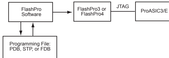
Figure 9-1 • FlashPro Programming Setup
