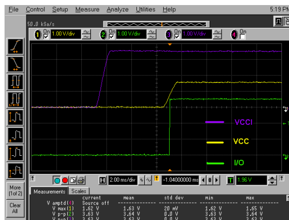
Figure 15-3 • I/O State when VCCI Is Powered before VCC
