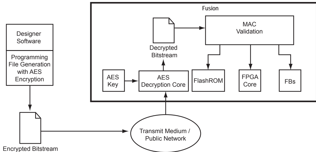
Figure 10-5 • Example Application Scenario Using AES in Fusion Devices
