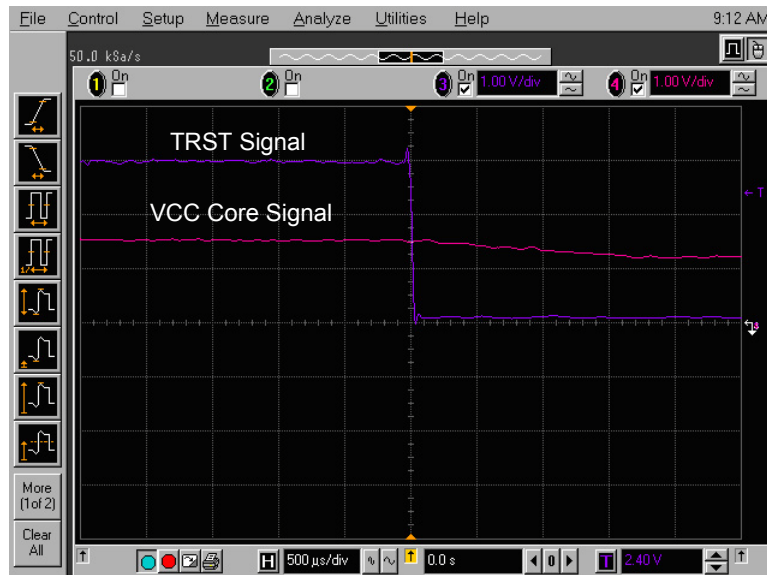
Figure 12-4 • TRST Toggled LOW
