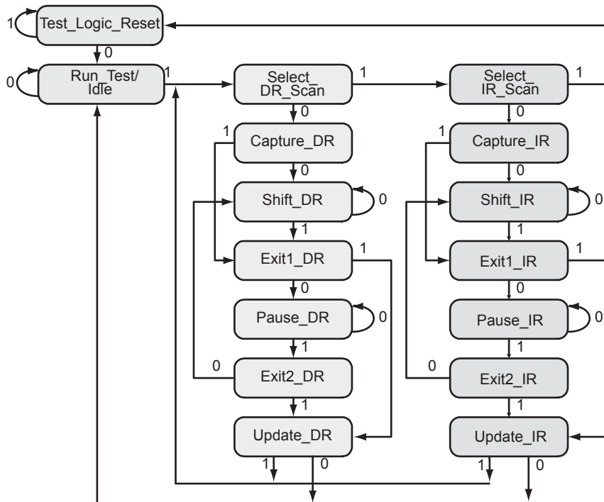
Figure 14-4 • TAP Controller State Diagram
