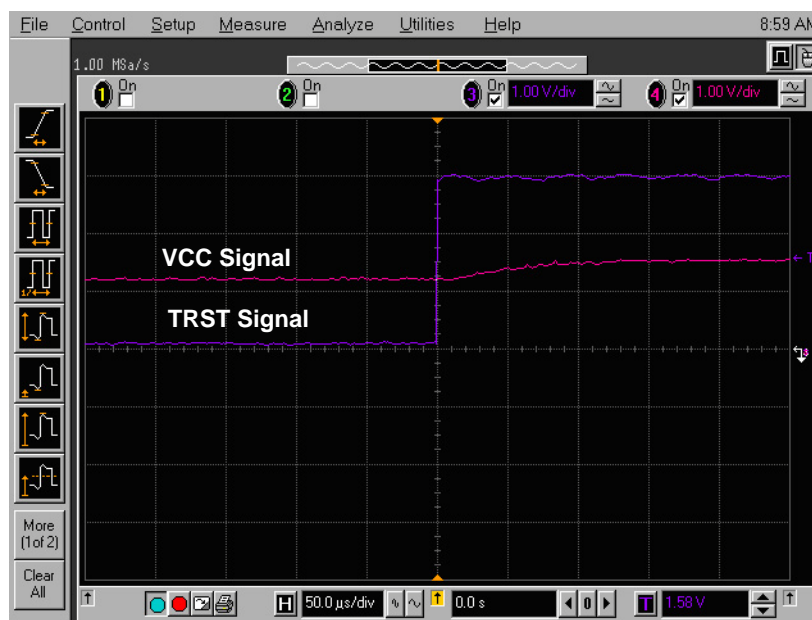
Figure 12-2 • Core Voltage on the IGLOO AGL125-QNG132 Device
