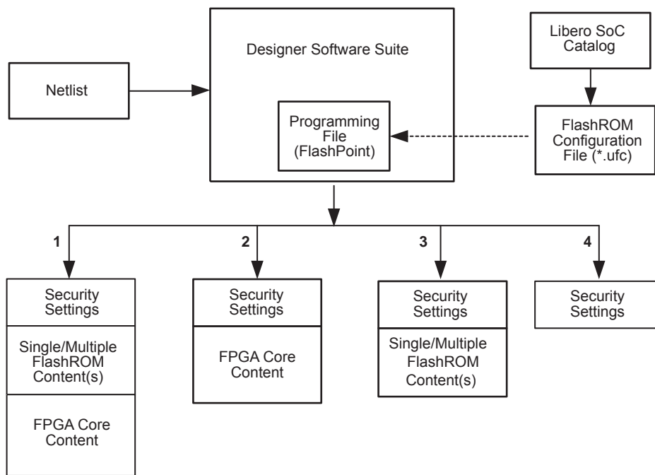
Figure 11-4 • Flexible Programming File Generation for Different Applications
