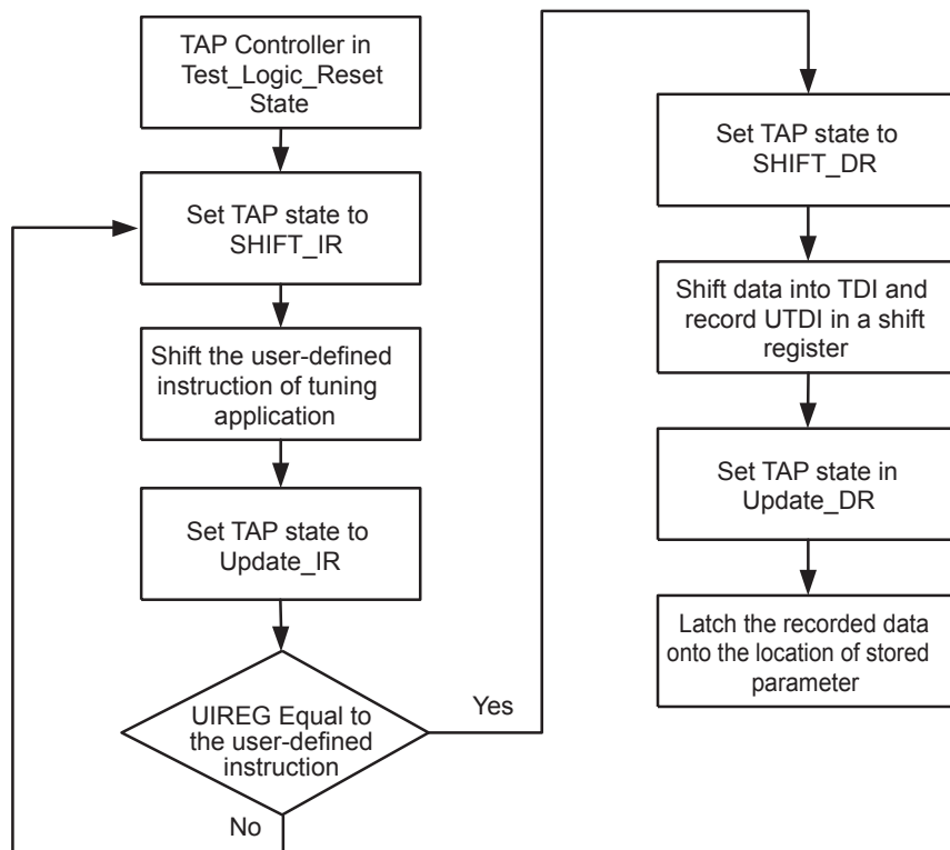
Figure 14-5 • Flow Chart Example of Fine-Tuning an Application Using UJTAG
