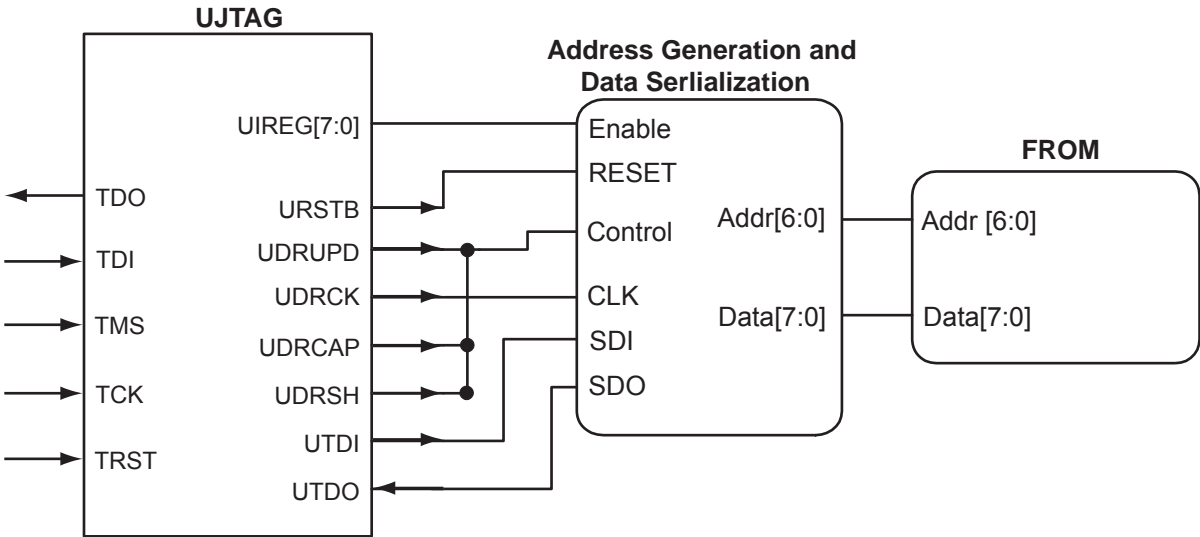
Figure 14-7 • Block Diagram of Using UJTAG to Read FlashROM Contents
