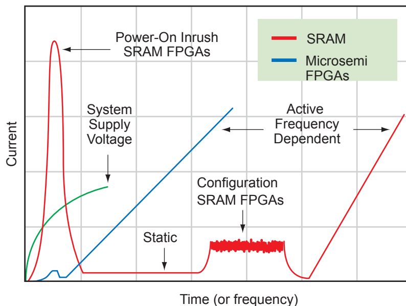
Figure 15-1 • Types of Power Consumption in SRAM FPGAs and Microsemi Nonvolatile FPGAs
