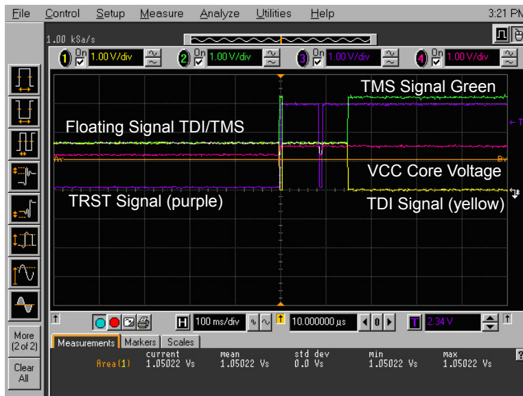
Figure 12-3 • Programming Algorithm
