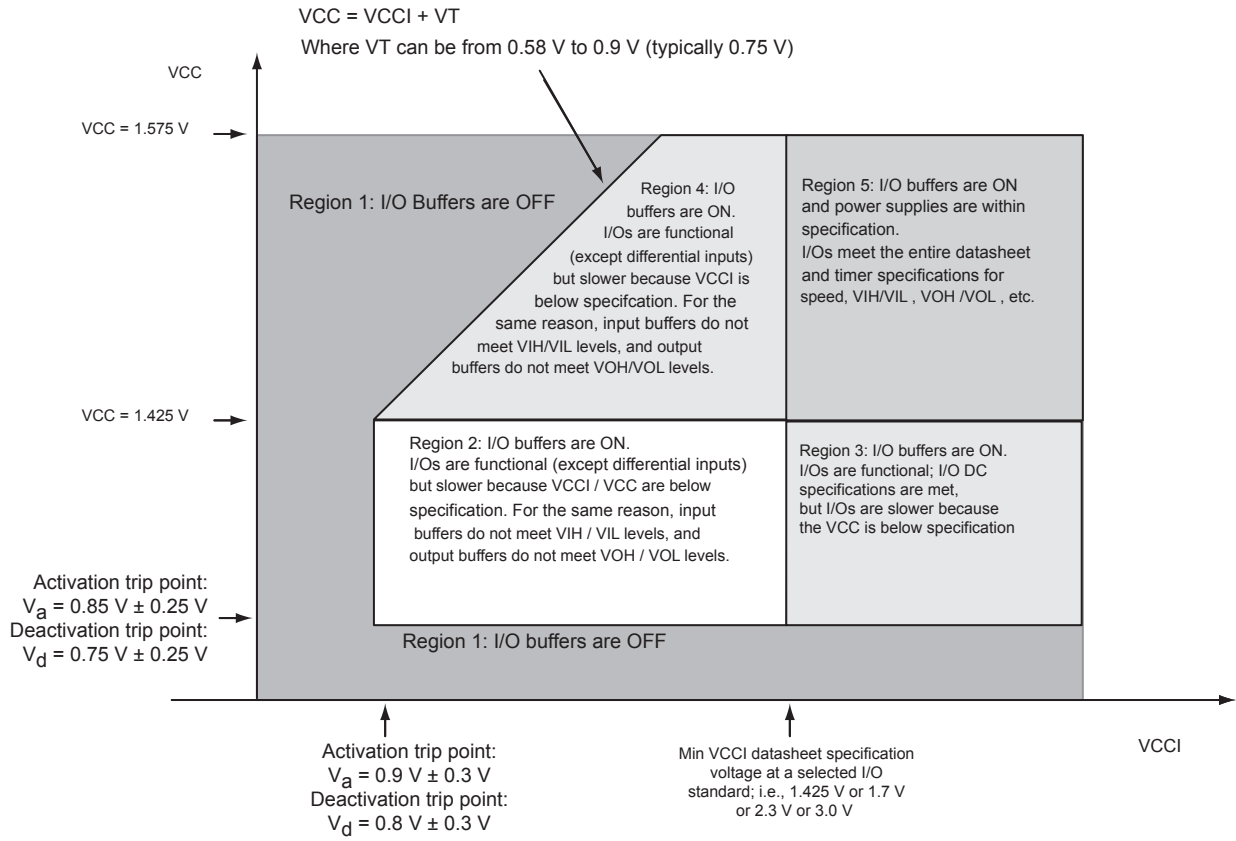
Figure 15-4 • I/O State as a Function of VCCI and VCC Voltage Levels for IGLOO V5, IGLOO nano V5, IGLOO PLUS V5, ProASIC3L, and ProASIC3 Devices Running at VCC = 1.5\text{ V} \pm 0.075\text{ V}
