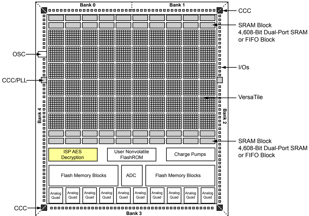
Figure 10-3 • Block Representation of the AES Decryption Core in a Fusion AFS600 FPGA
