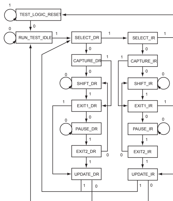
Figure 13-1 • TAP Controller State Machine
