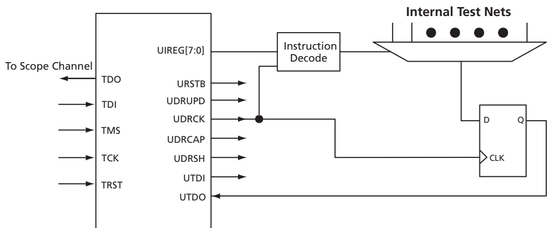
Figure 14-6 • UJTAG Usage Example in Test and Debug Applications
