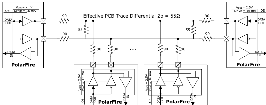
Figure 7-6. Bus-LVDSE System Diagram
