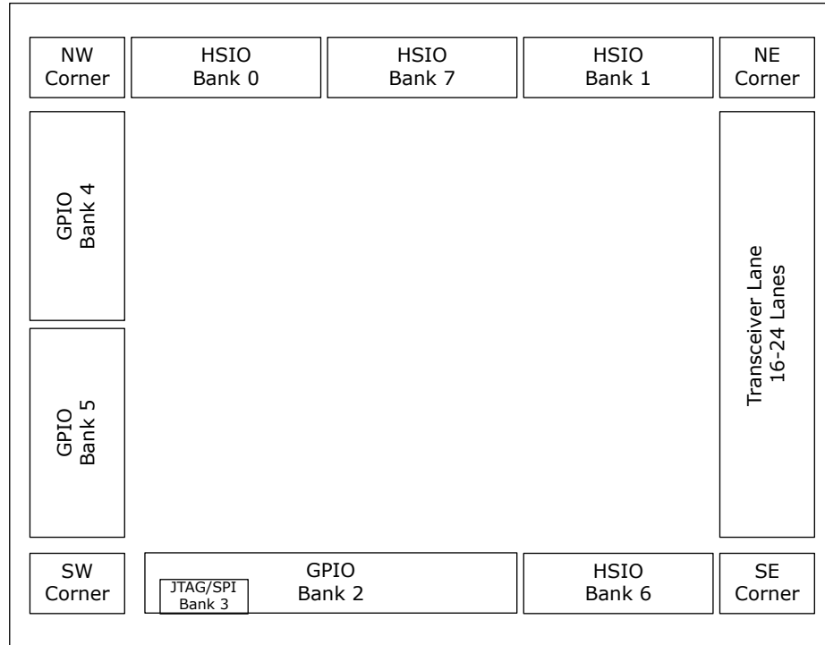
Figure 3-1. PolarFire FPGA MPF300T/MPF300XT/MPF500T and RT PolarFire FPGA RTPF500T I/O Banks (Top View)
