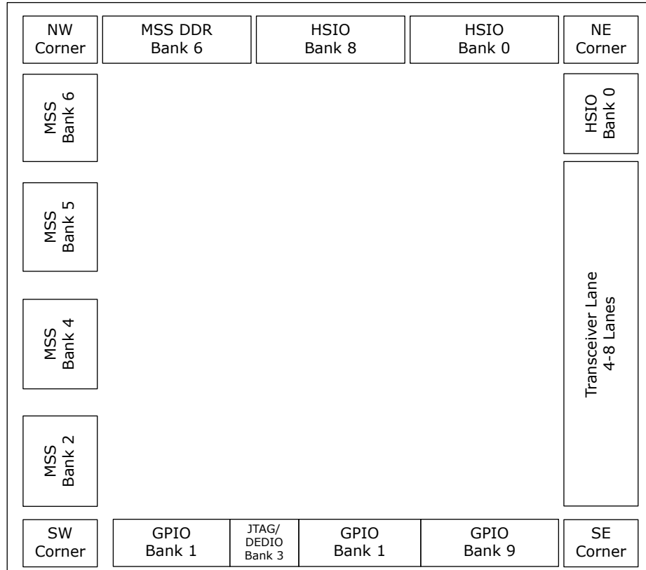
Figure 3-8. PolarFire SoC FPGA MPFS095 I/O Banks (Top View)
