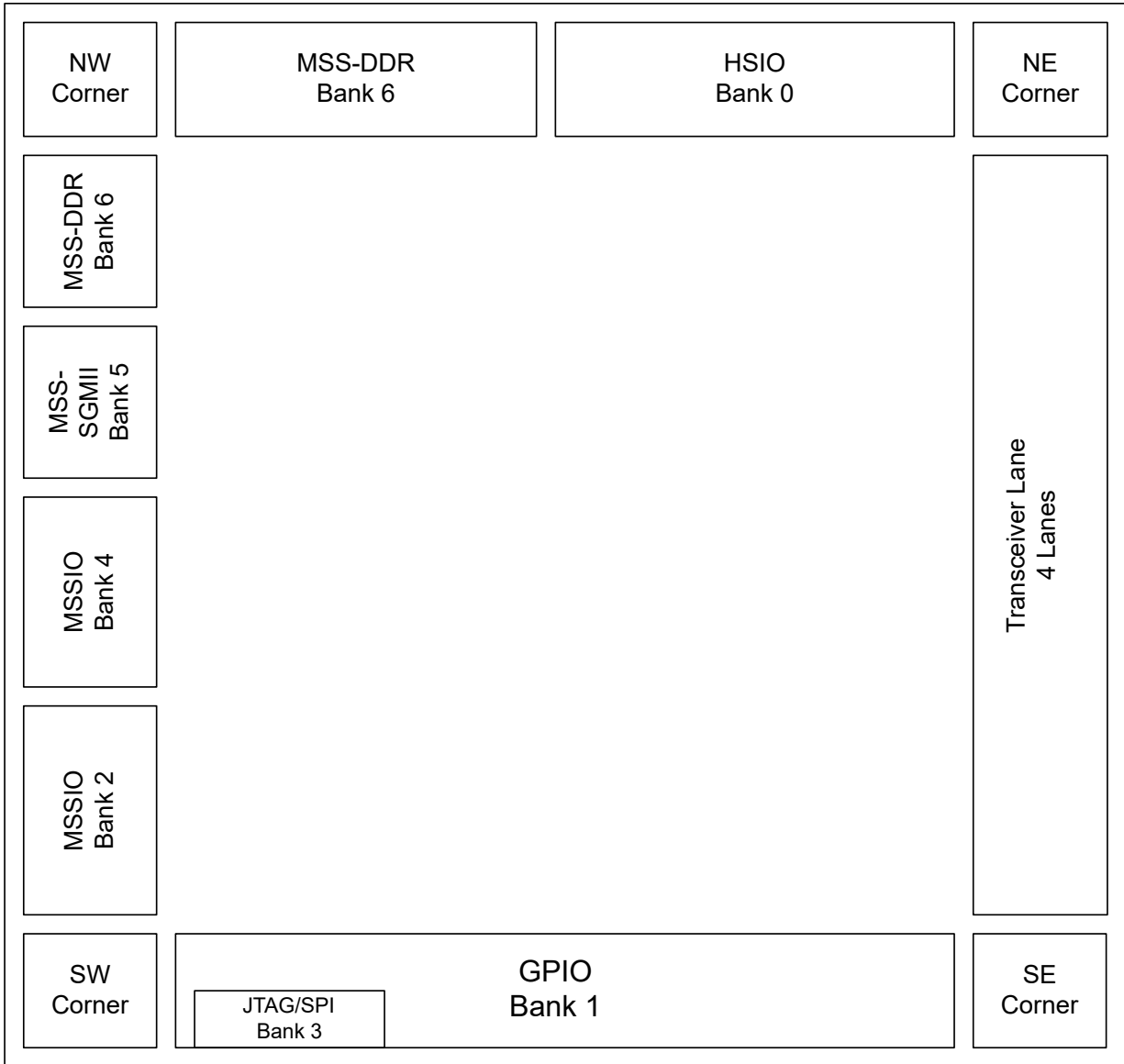
Figure 3-5. PolarFire SoC FPGA MPFS250–FCVG484 I/O Banks (Top View)
