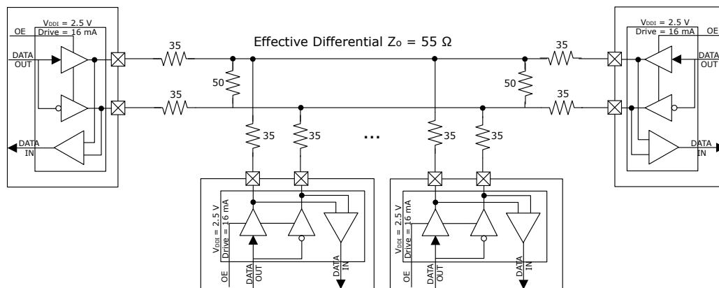
Figure 7-7. MLVDSE System Diagram
