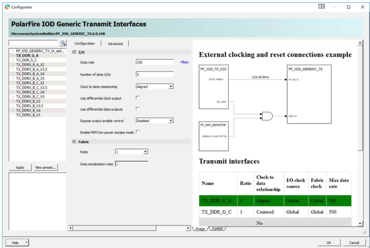
Figure 9-4. IOD Generic Transmit Interfaces—Configuration Tab
