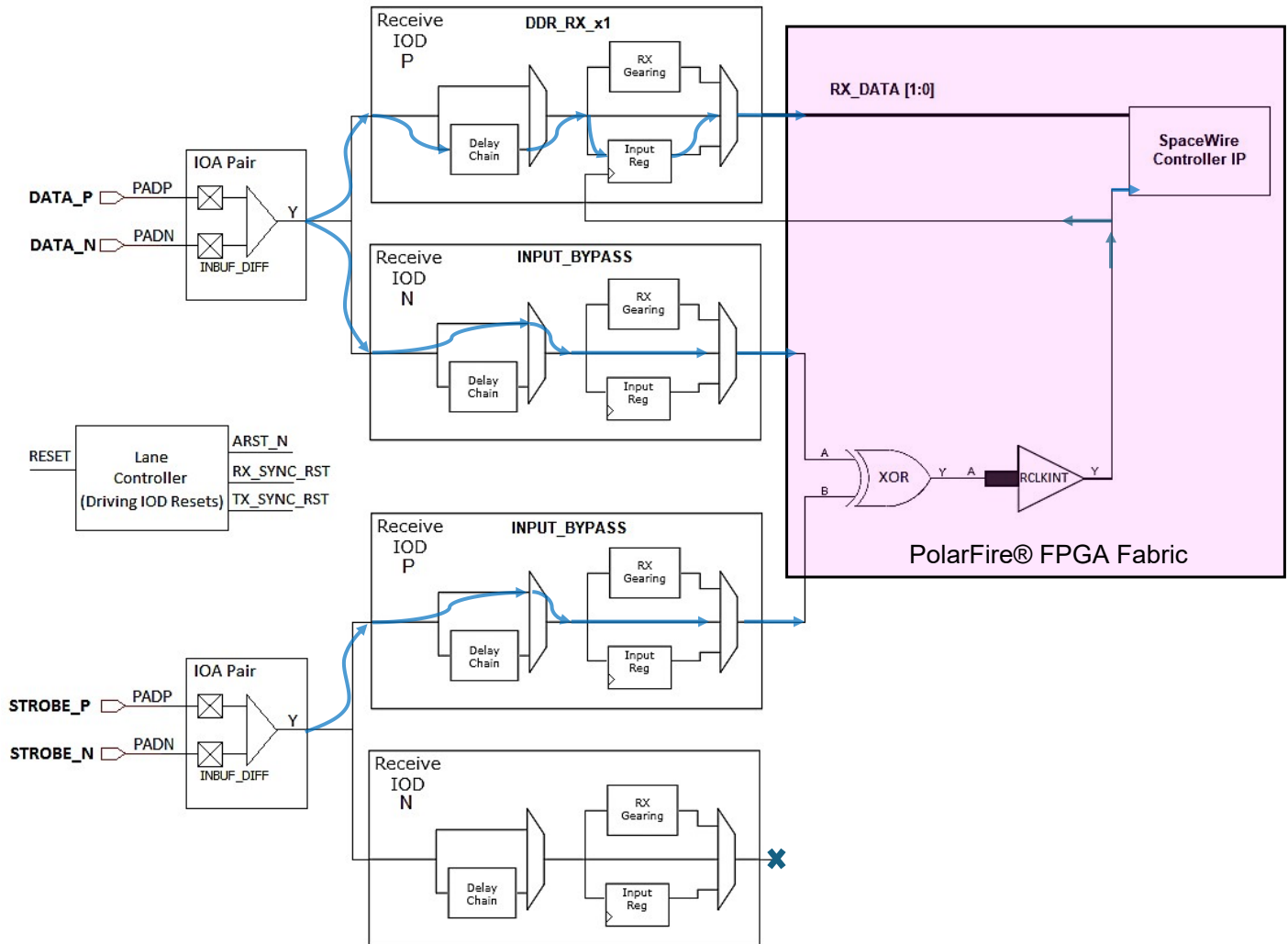
Figure 10-15. SpaceWire RX PHY Implementation in RT PolarFire and RT PolarFire SoC FPGA
