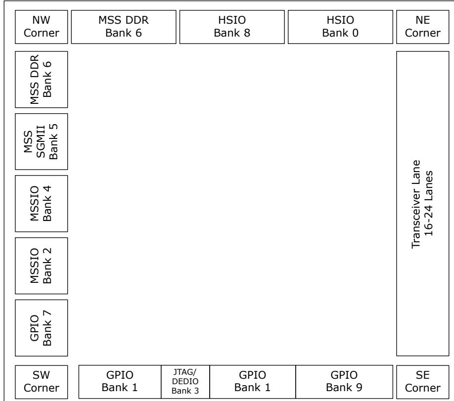
Figure 3-6. PolarFire SoC FPGA MPFS250/MPFS460 and RT PolarFire SoC FPGA RTPFS460 I/O Banks (Top View)
