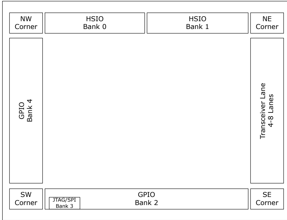
Figure 3-3. PolarFire FPGA MPF050/MPF100T Device I/O Banks (Top View)
