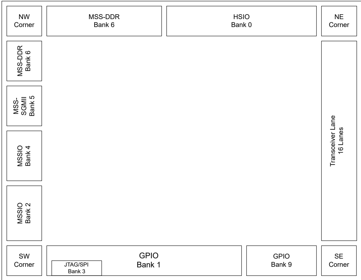
Figure 3-4. PolarFire SoC FPGA MPFS250–FCG1152 I/O Banks (Top View)
