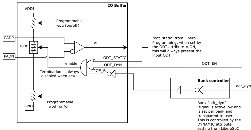
Figure 7-14. Dynamic ODT used for Fail-safe LVDS
