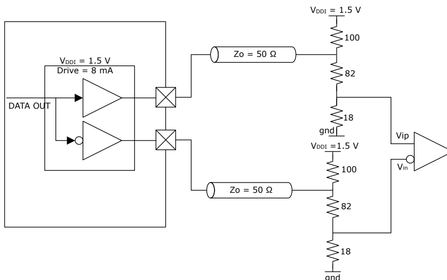
Figure 7-5. SLVSE System Diagram
