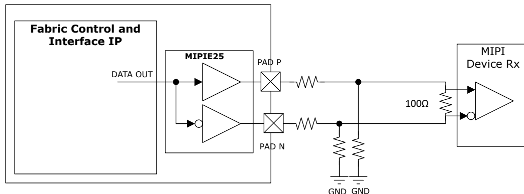
Figure 7-10. MIPI D-PHY Transmit Interface
