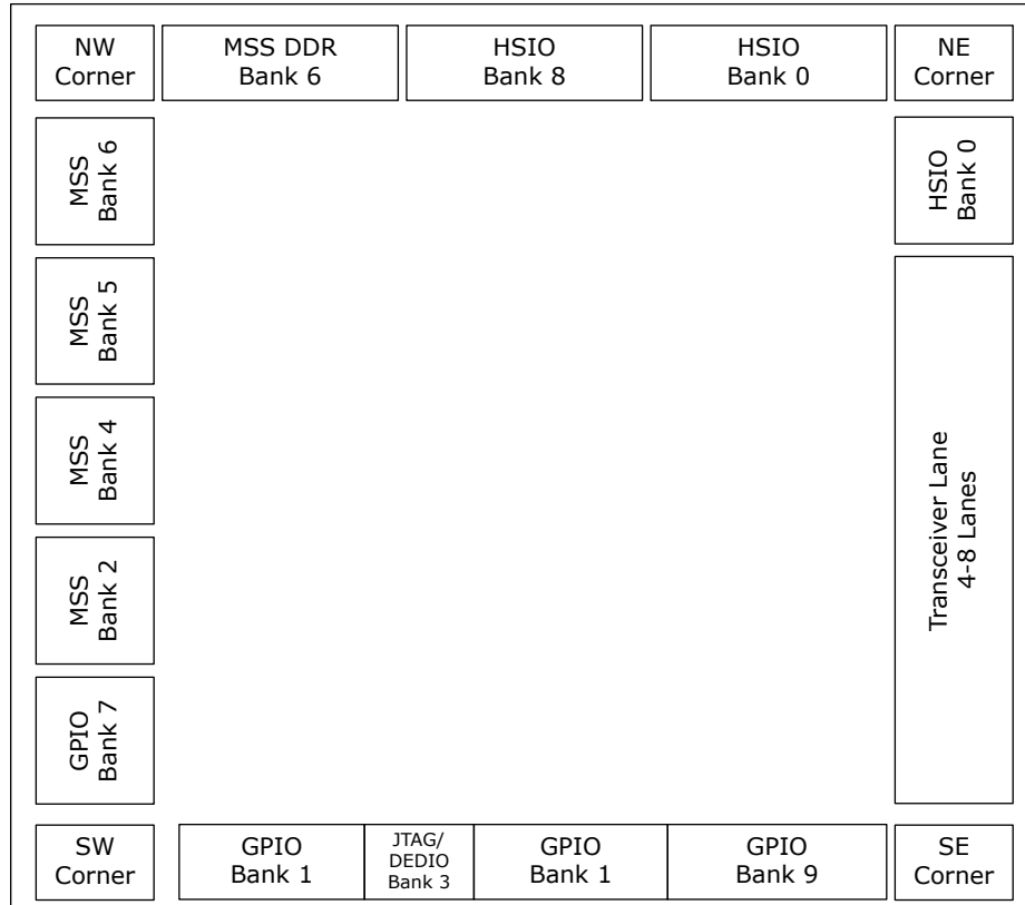
Figure 3-7. PolarFire SoC FPGA MPFS160 and RT PolarFire SoC FPGA RTPFS160 I/O Banks (Top View)
