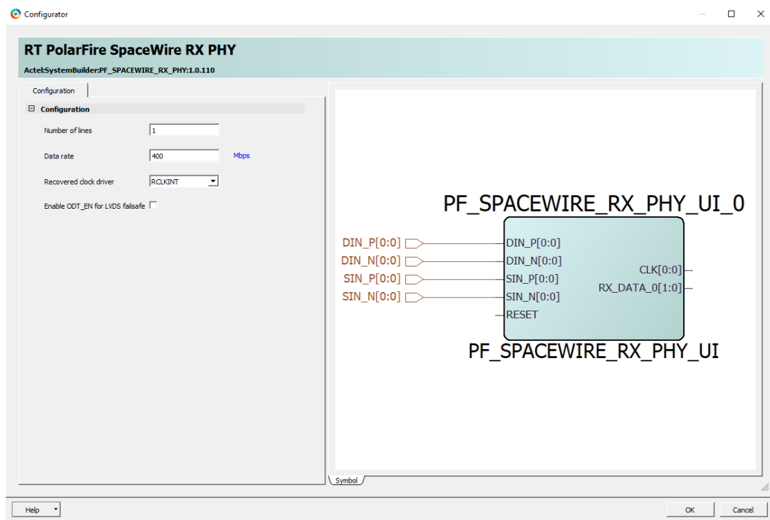
Figure 10-16. RT PolarFire and RT PolarFire SoC SpaceWire RX PHY
