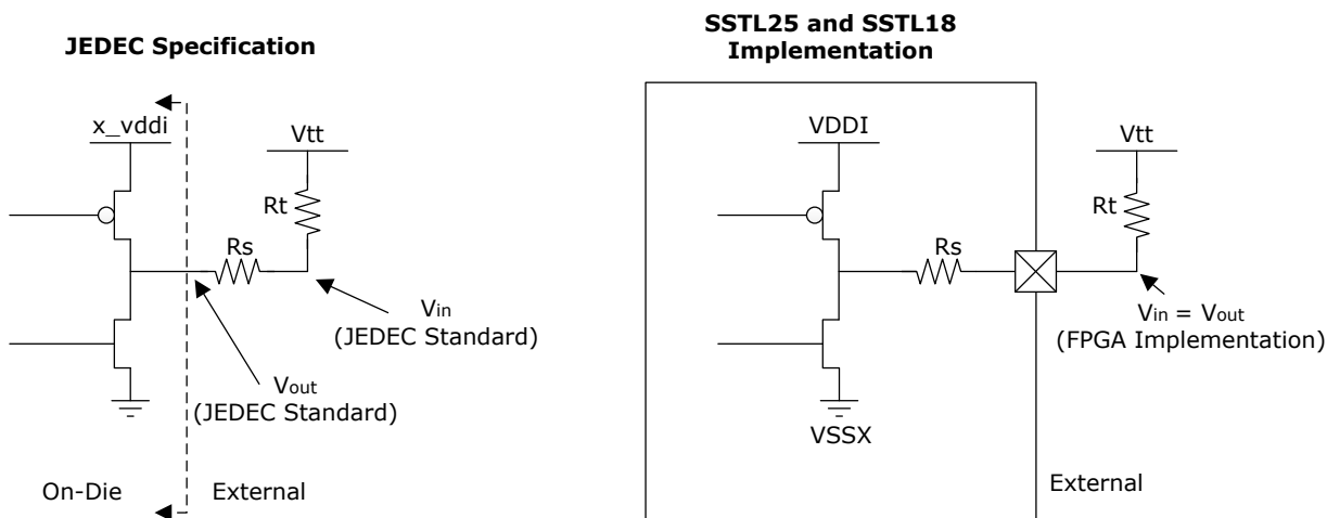
Figure 7-3. SSTL25 and SSTL18 Stub Resistor
