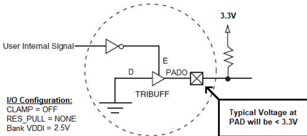
Figure 7-4. Open Drain GPIO Example
