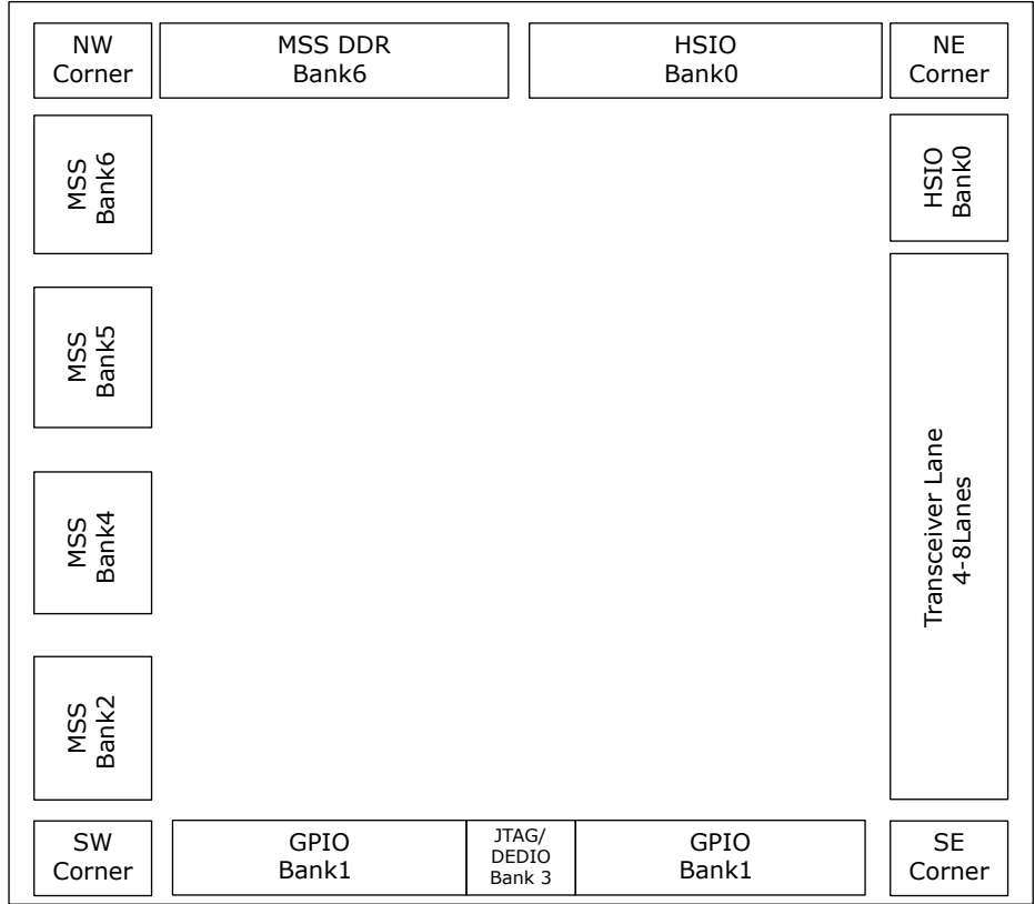
Figure 3-9. PolarFire SoC FPGA MPFS025 I/O Banks (Top View)
