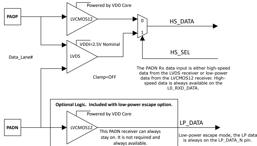
Figure 7-9. MIPI D-PHY Receiver
