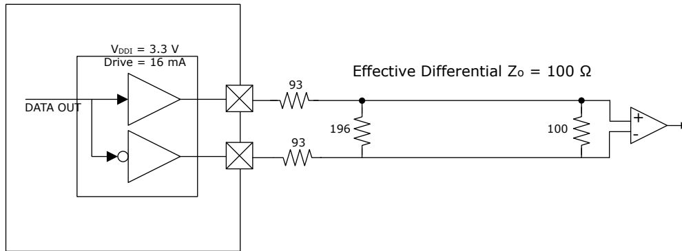
Figure 7-8. LVPECL System Diagram
