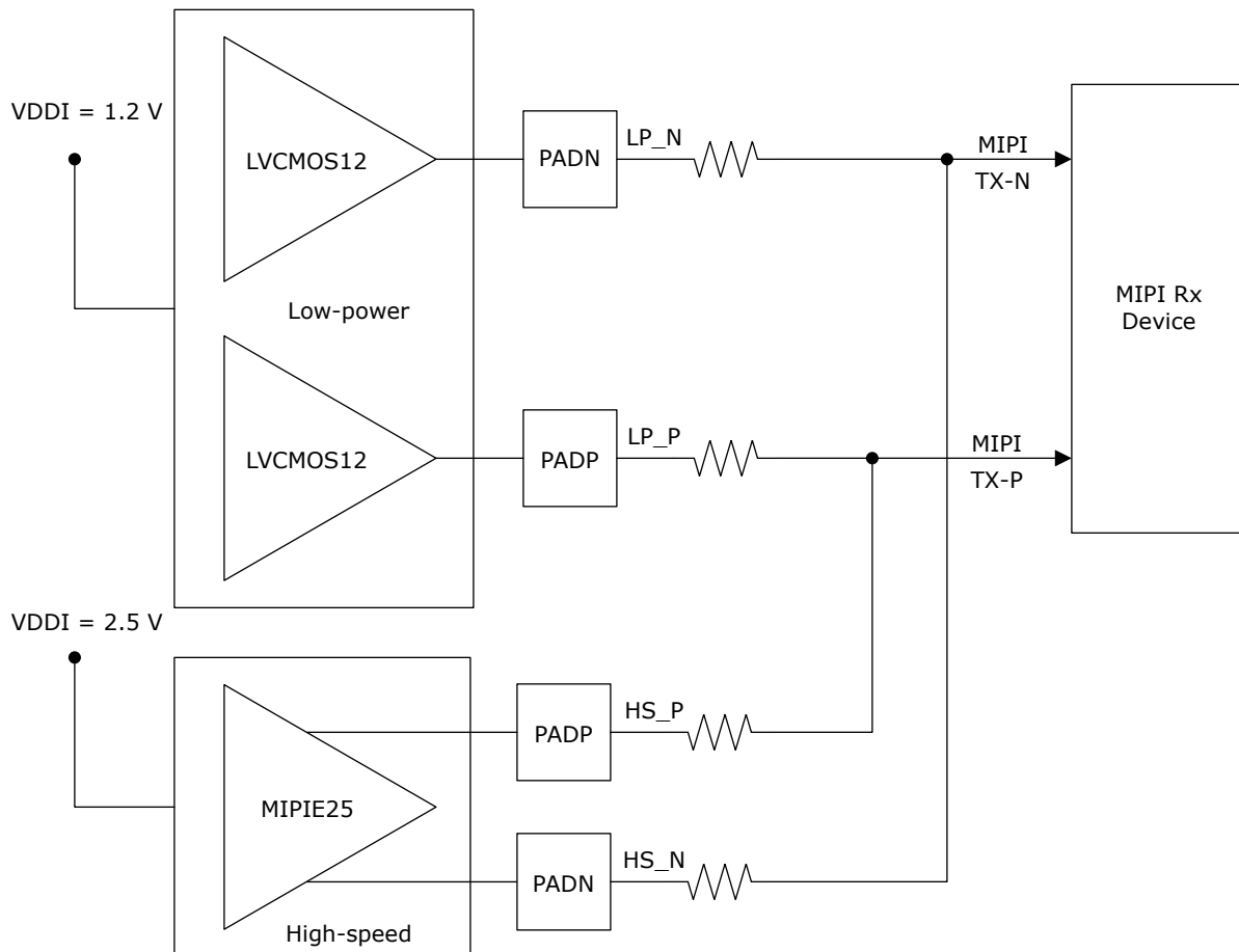
Figure 7-11. MIPI D-PHY Transmit Interface (High-Speed and Low-Power)
