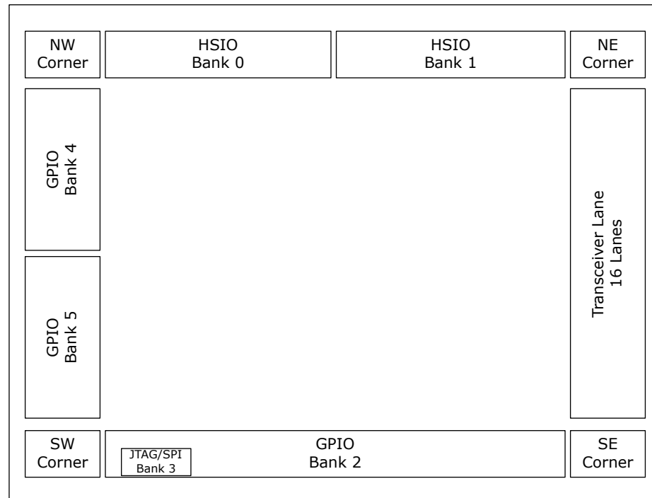
Figure 3-2. PolarFire FPGA MPF200T Device I/O Banks (Top View)
