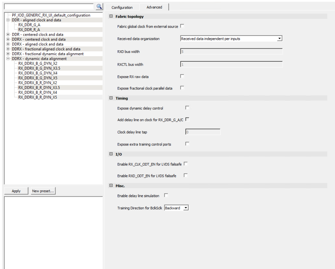
Figure 10-12. RX_DDRX_B_G_FA Interface—Advanced Tab
