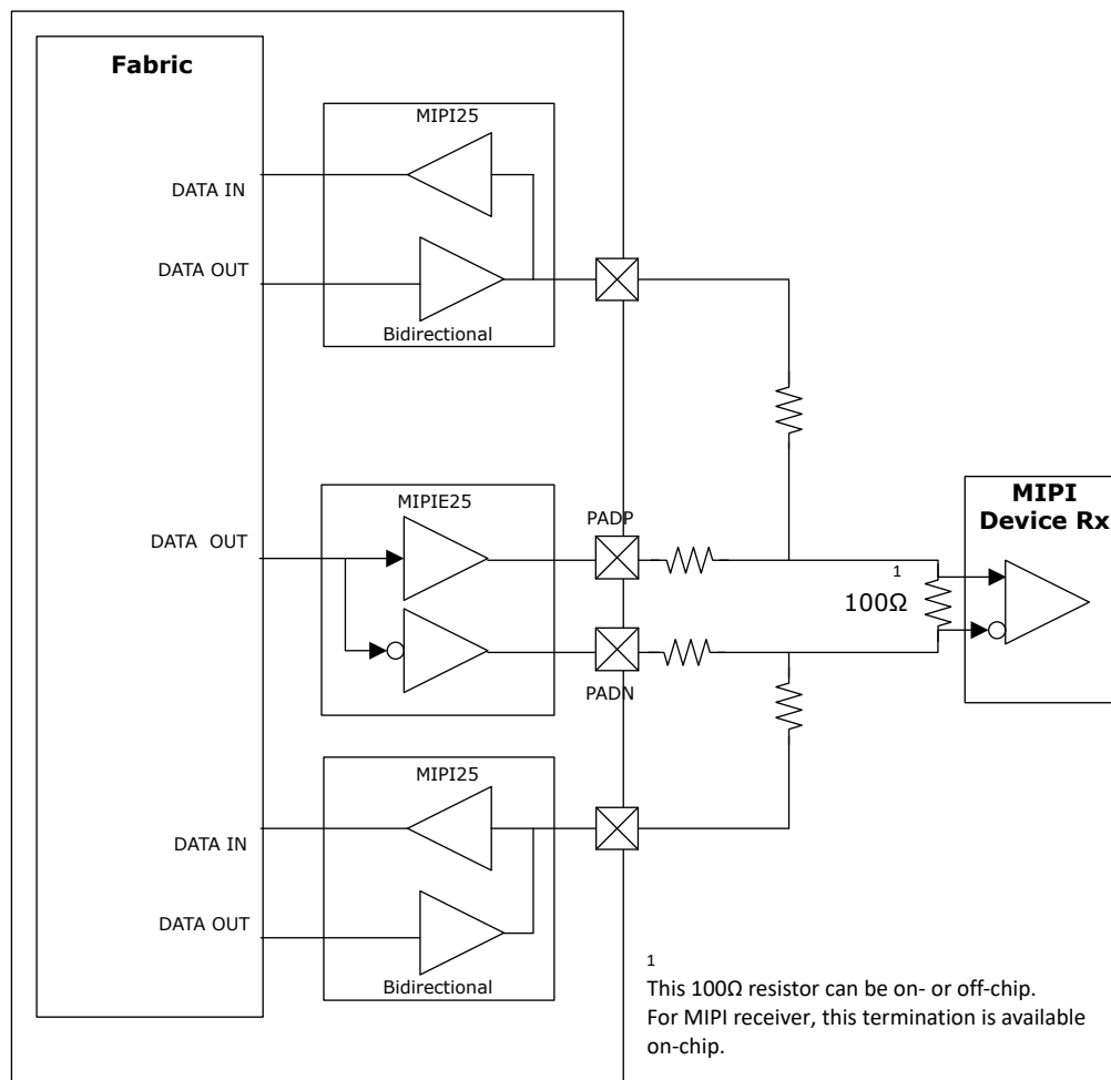
Figure 7-13. High-Speed Transmit With Bidirectional
