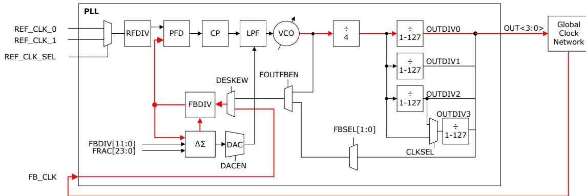
Figure 4-10. External Feedback Mode—Feedback through Global Clock Network
