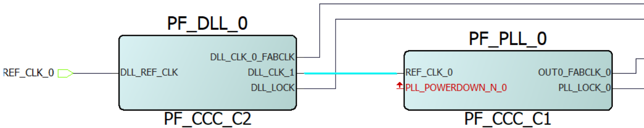
Figure 4-23. DLL Driving PLL
