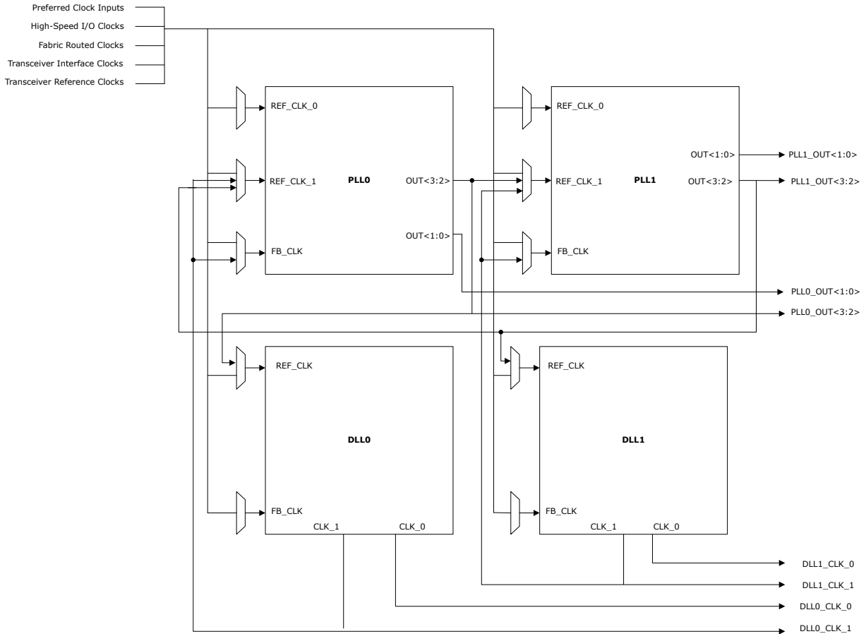
Figure 4-22. CCC Block Diagram
