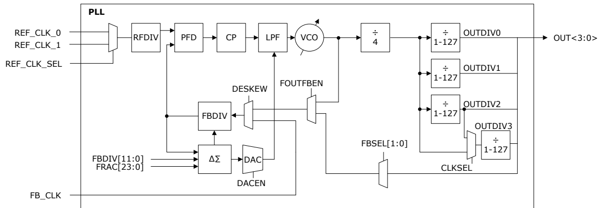
Figure 4-13. Frequency Synthesis
