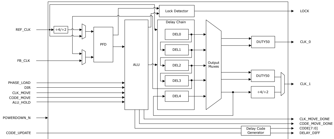
Figure 4-15. DLL Block Diagram
