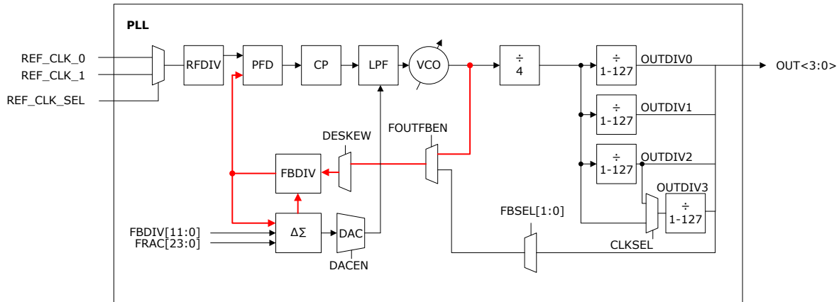
Figure 4-8. Internal Post-VCO Feedback Mode
