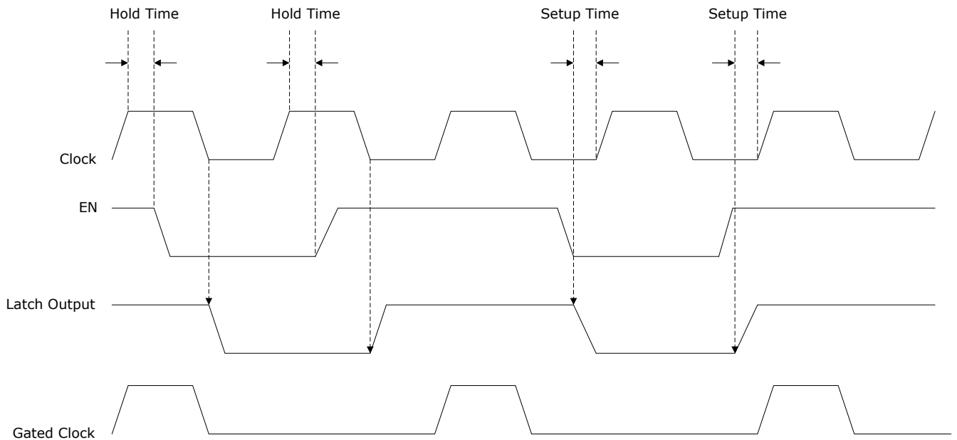
Figure 2-17. forms for the Clock Gating Circuitry
