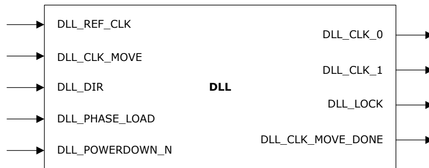
Figure 4-18. DLL Port List—Phase Generation Mode
