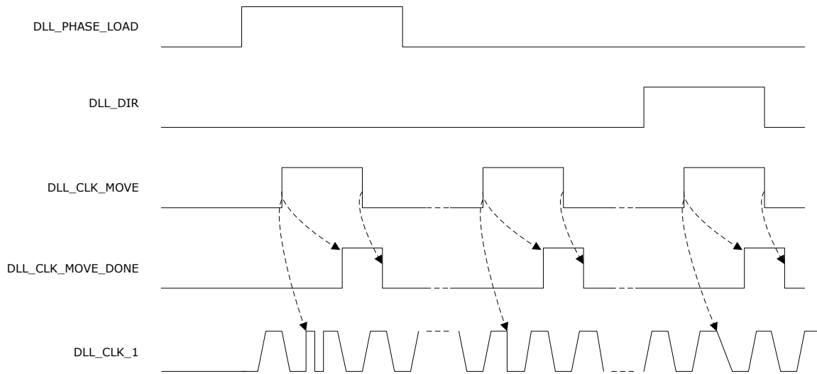
Figure 4-19. Phase Generation Mode—DLL_CLK_1 Dynamic Configuration
