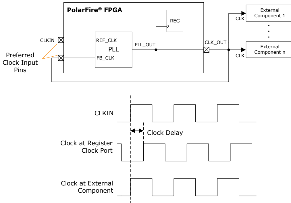
Figure 4-14. Zero-Delay Buffer—Phase Relationship Between Clocks
