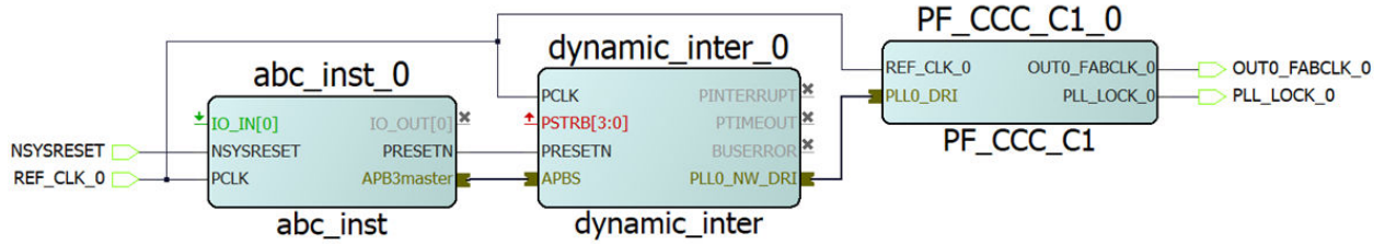
Figure 4-34. CCC Dynamic Configuration System
