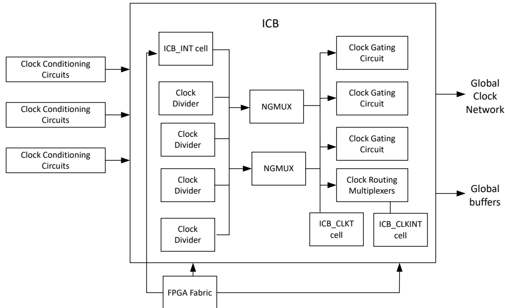
Figure 2-9. Interface Clock Block
