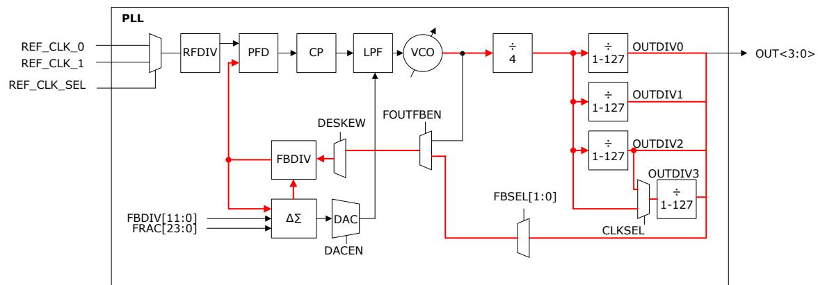
Figure 4-9. Internal Post-Divider Feedback Mode
