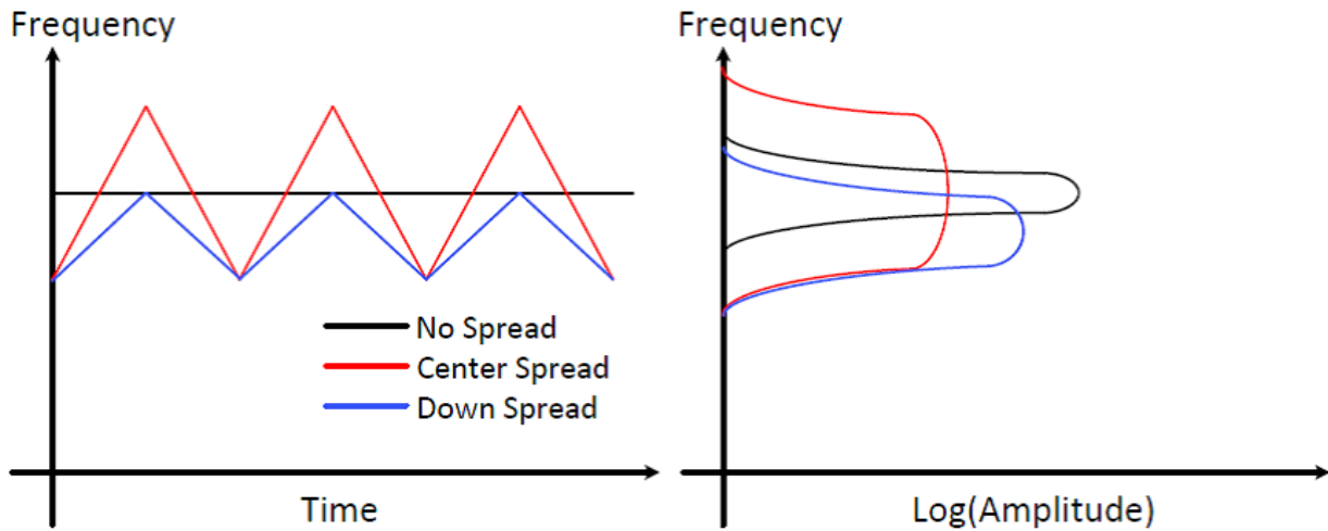
Figure 4-12. Spread Spectrum in Time and Frequency Domain Using Triangular-Modulated Waveform
