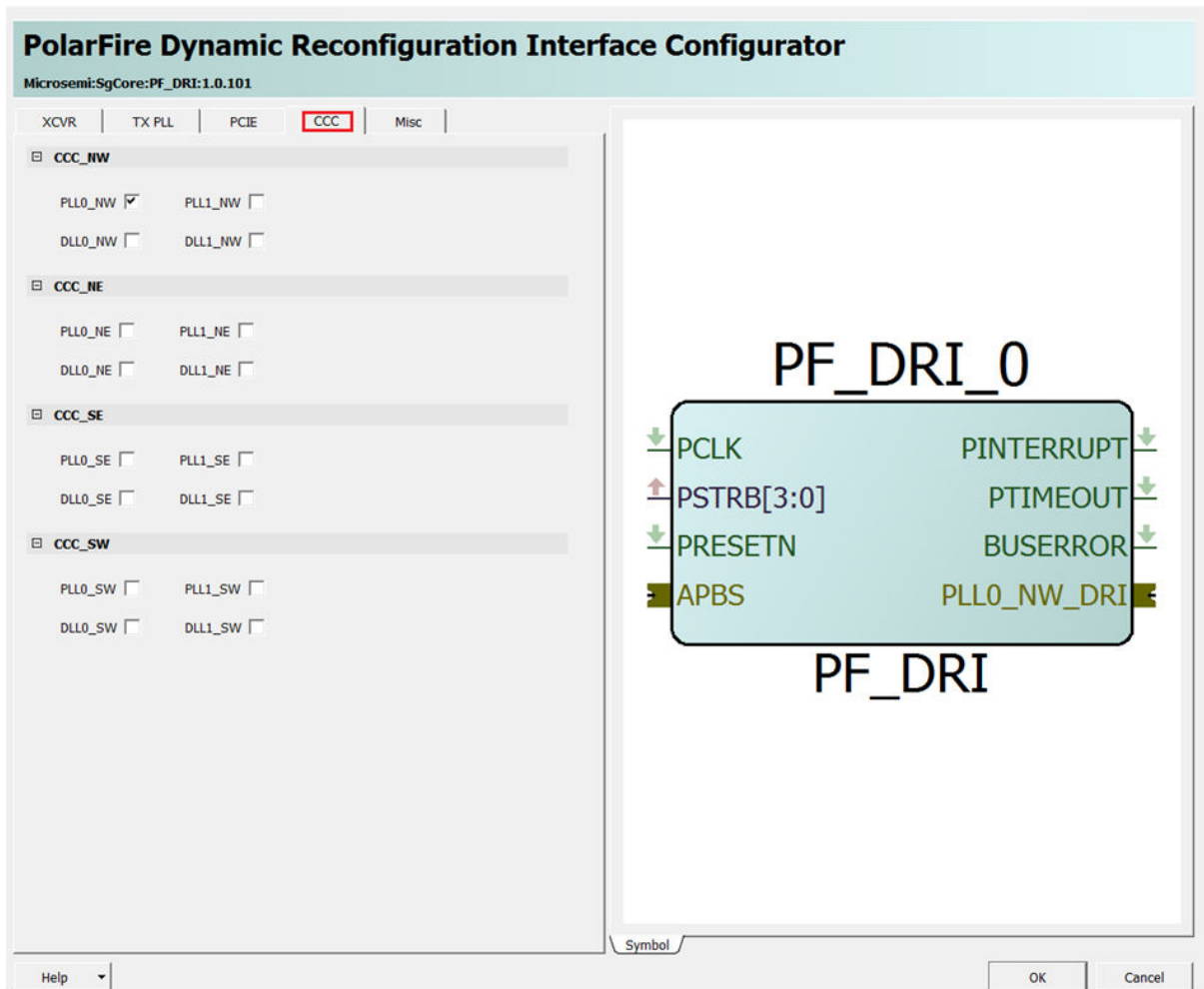
Figure 4-33. Dynamic Reconfiguration Interface Configurator
