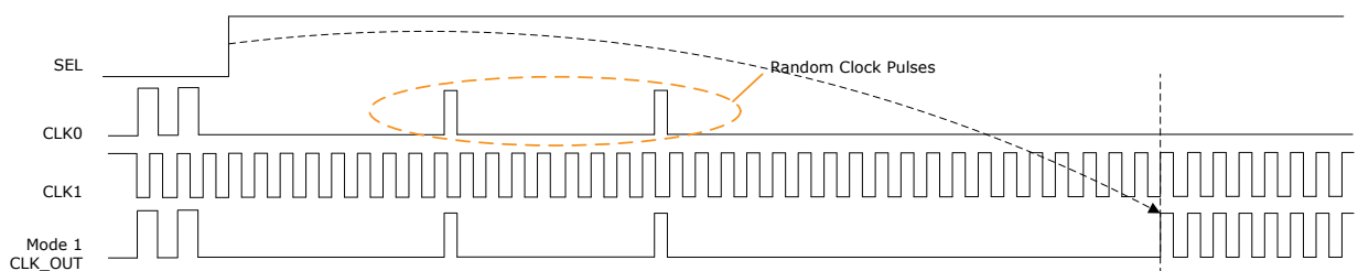
Figure 2-15. Mode 1: Clock Switching when Current Clock (CLK0) is Uncertain with Random Pulses
