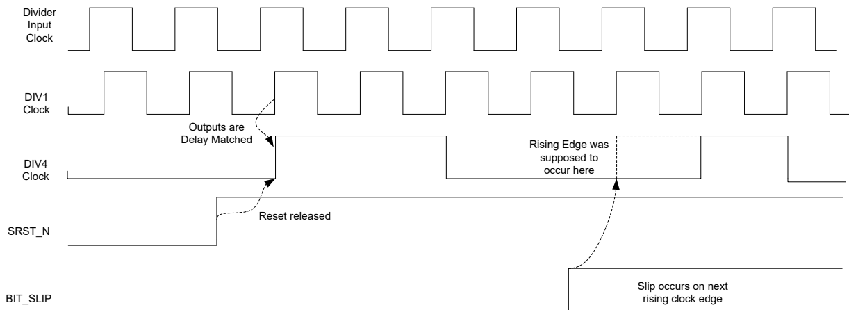
Figure 2-10. Using the Reset and Slip Operations for the ICB Dividers
