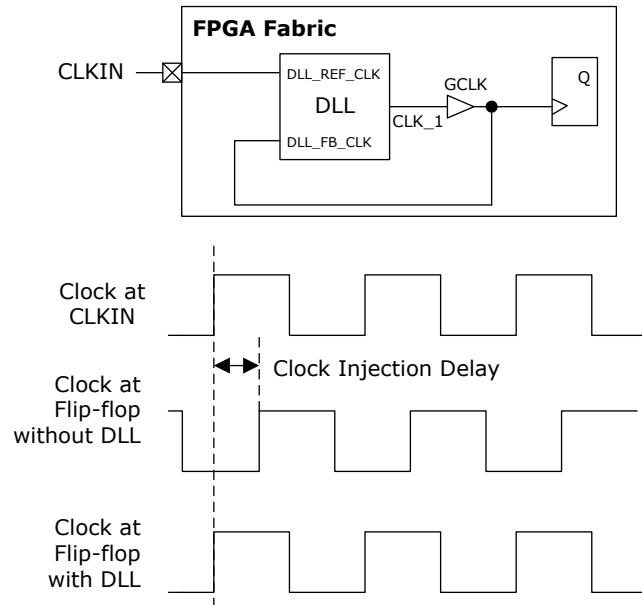
Figure 4-21. Clock Injection Delay Removal Mode
