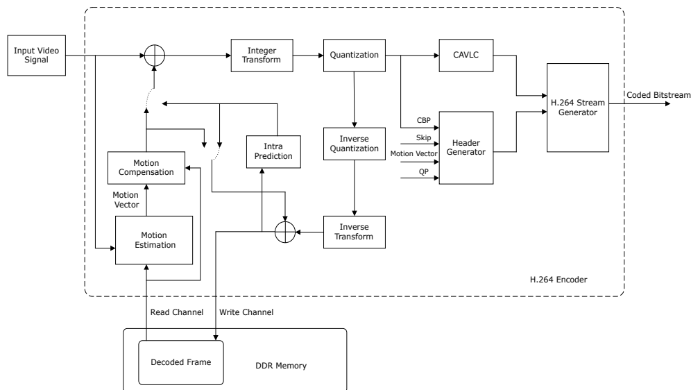
Figure 2-6. Slice Encoder Block Diagram
