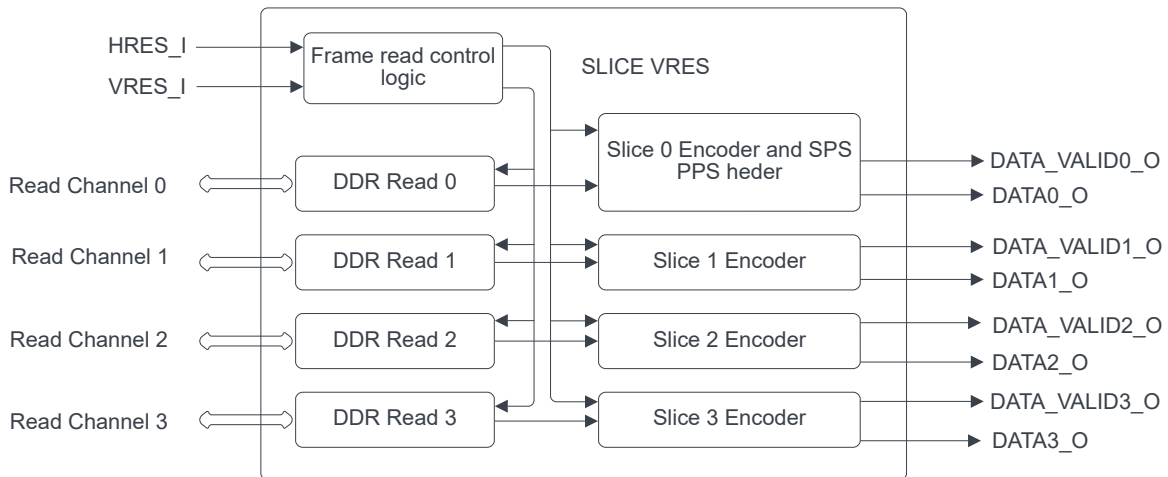
Figure 2-5. Block Diagram
