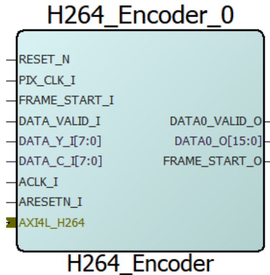
Figure 2-2. H.264 Encoder Block Diagram (P_Frame = 1, 4K = 0)
