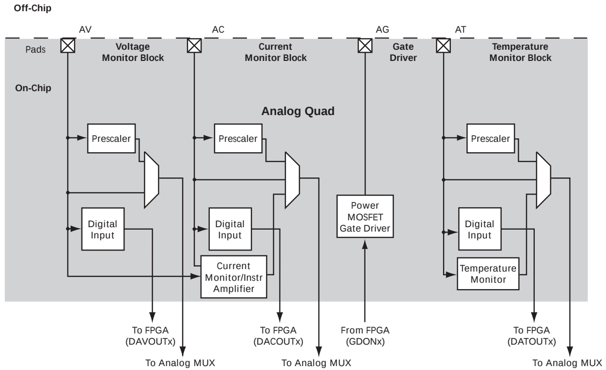
Figure 1: Analog Quad
