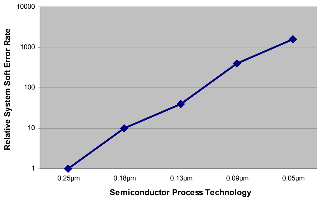
Figure 4: Soft Error Rates as a Function of IC Process Technology 4
