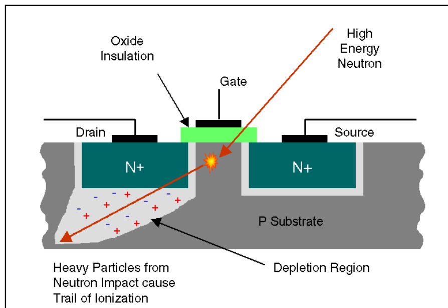
Figure 3: Interaction of a High-Energy Neutron and a Silicon Integrated Circuit
