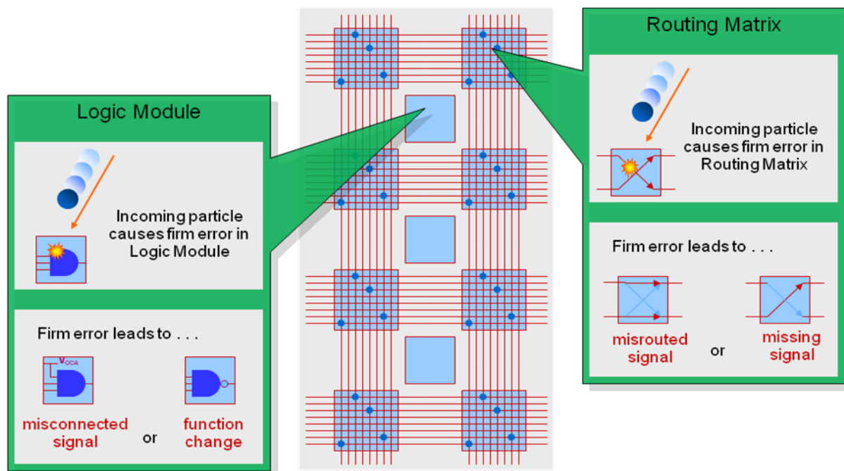
Figure 7: Firm-Error Effect on an SRAM FPGA
