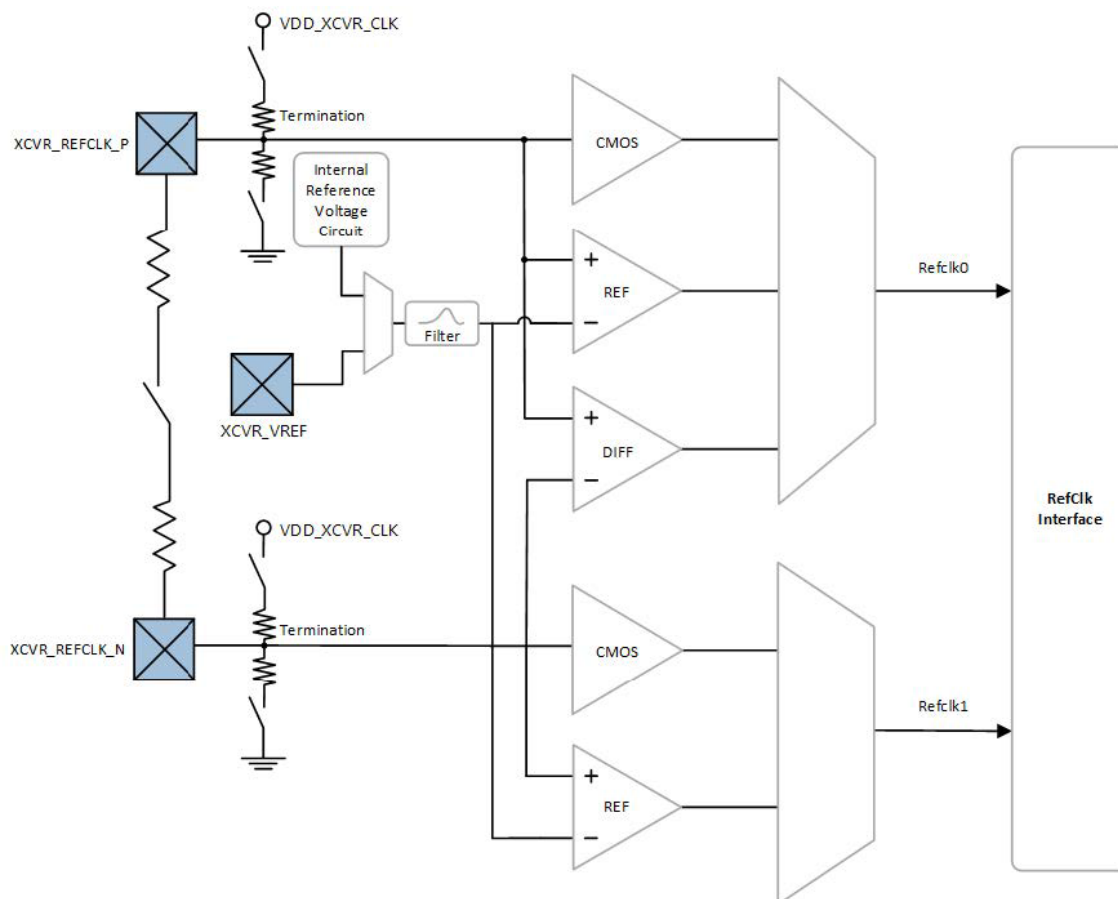
Figure 7-2. Reference Clock
