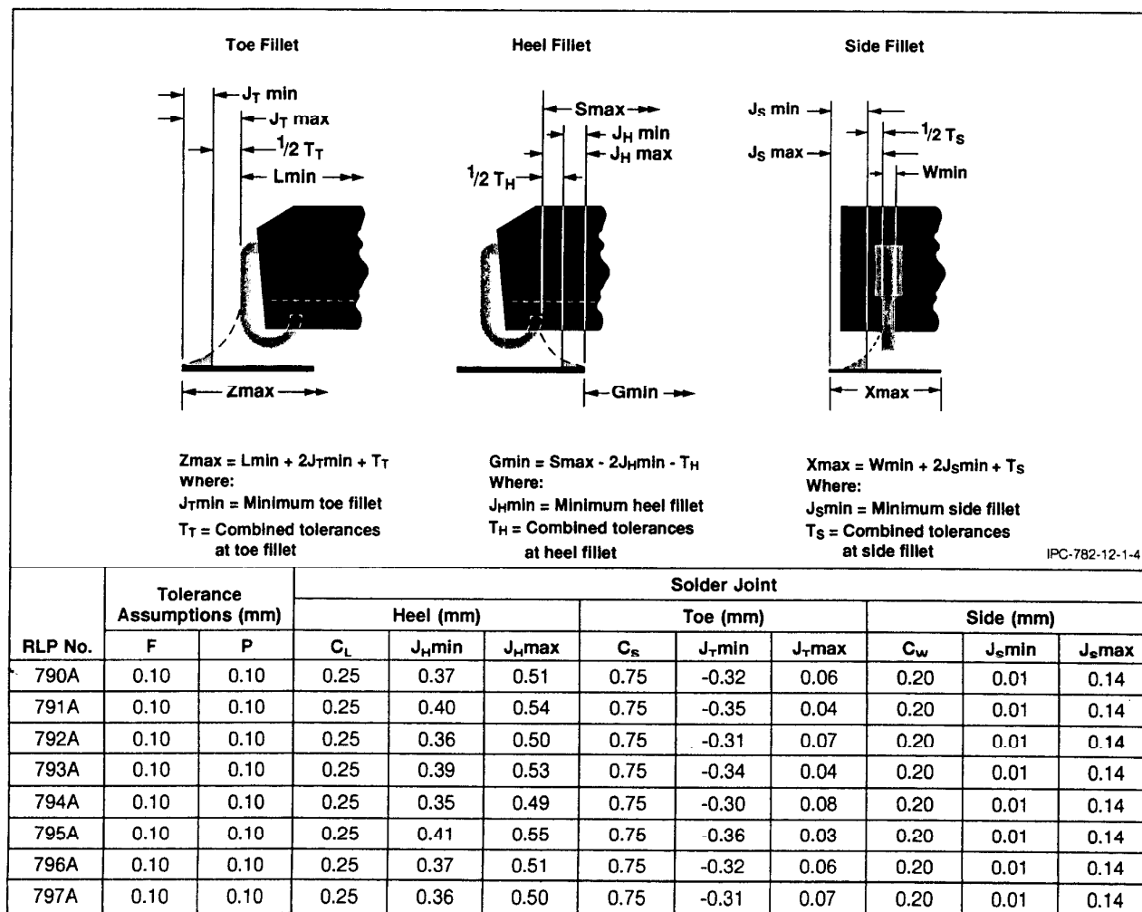
Figure 4 Tolerance and solder joint analysis
