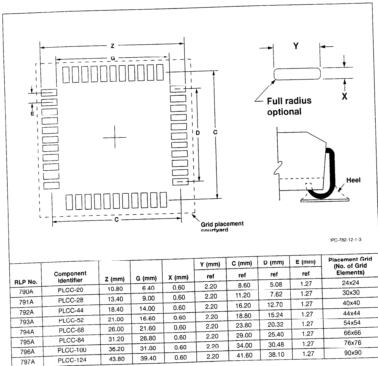
Figure 3 PLCC (Square) land pattern dimensions
