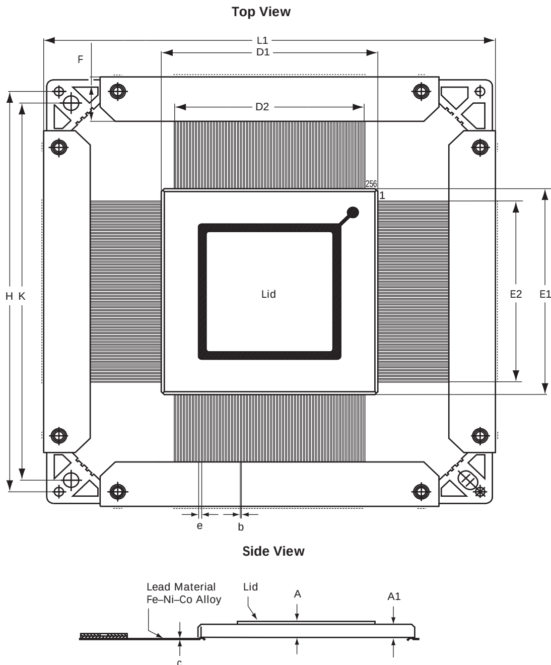
Figure 14 • CQ256—Cavity Down without Heat Sink
