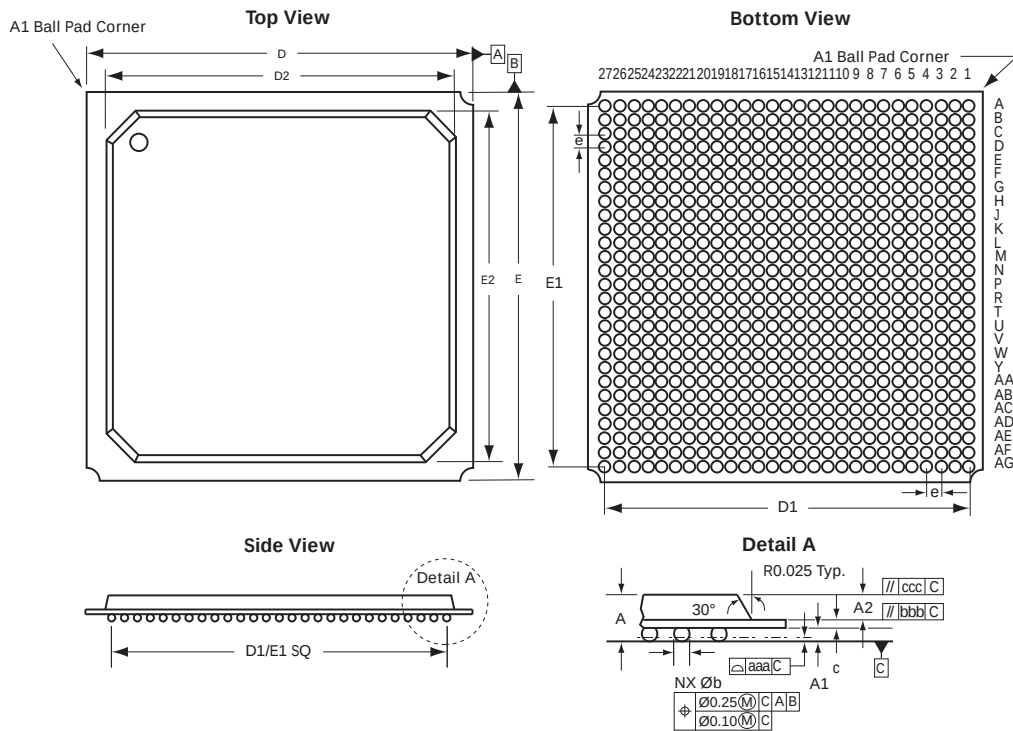
Figure 41 • Package Outline of BG729
