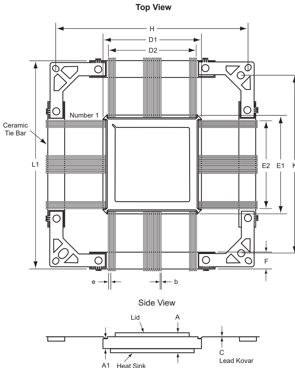
Figure 13 • CQ208 and CQ256—Cavity Up with Heat Sink
