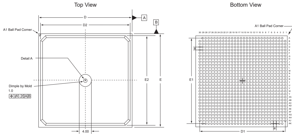
Figure 52 • Package Outline of FG896 Larger Mold Cap Size
