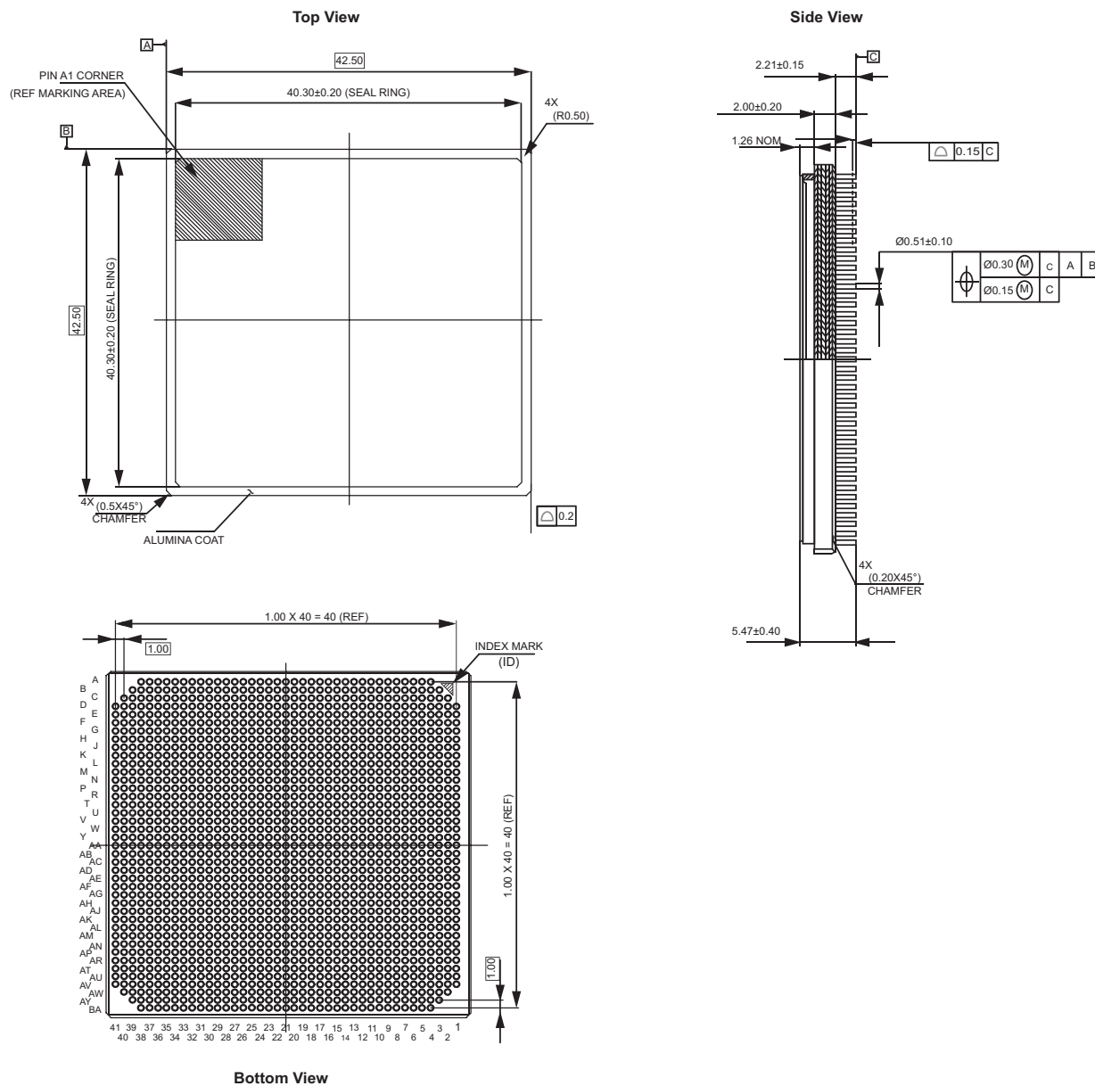
Figure 24 • Package Outline of CG1657
