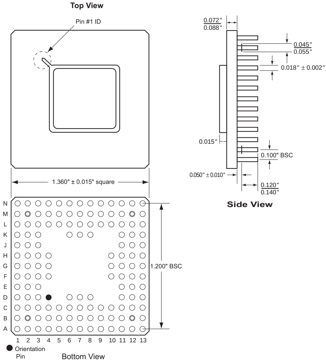
Figure 3 • Package Outline of PG132
