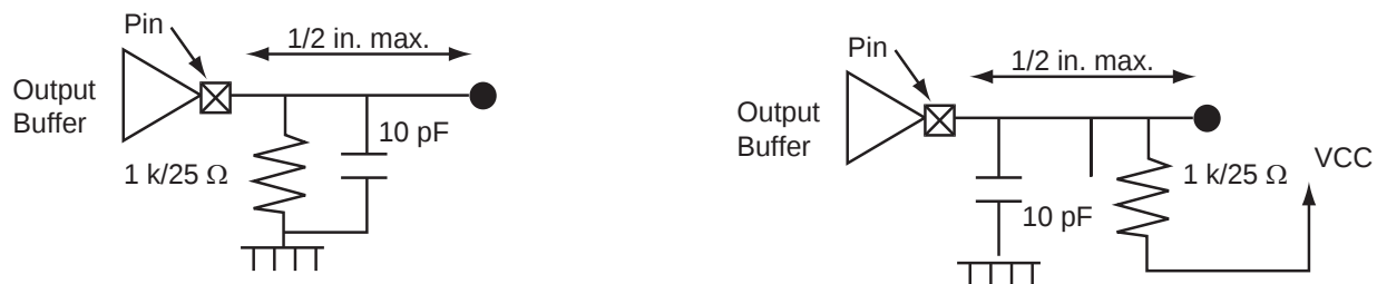
Figure 2-10 • 3.3 V PCI Output Loading
