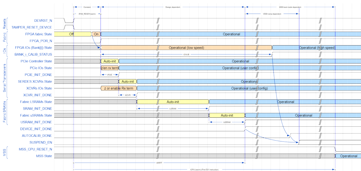
Figure 4-14. Warm Reset Timing (RTPFS460ZT and RTPFS160ZT)
