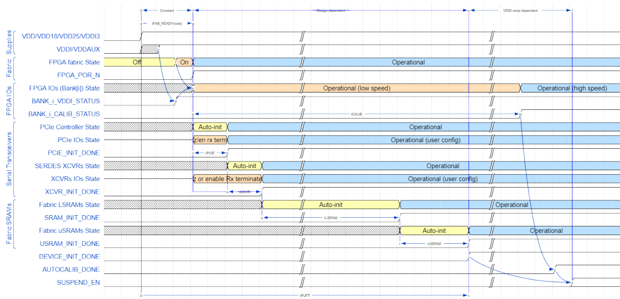
Figure 4-13. Cold Reset Timing (RTPF500T and RTPF500ZT)
