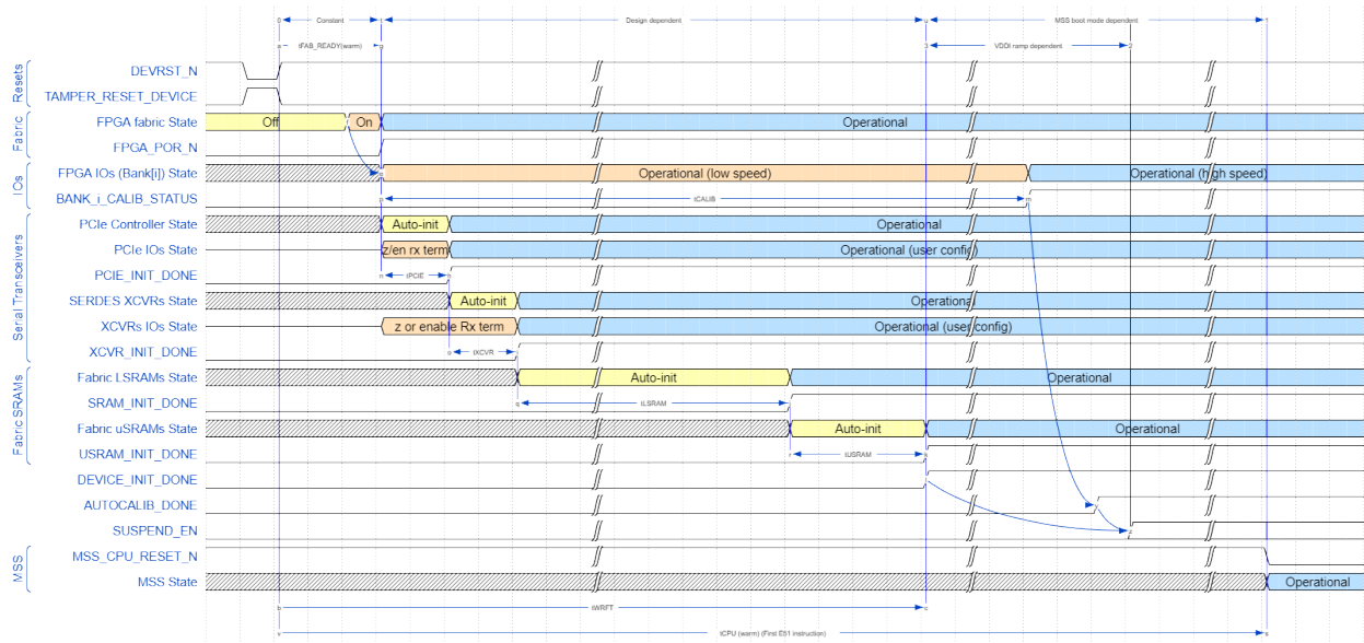
Figure 4-15. Warm Reset Timing (RTPF500T and RTPF500ZT)
