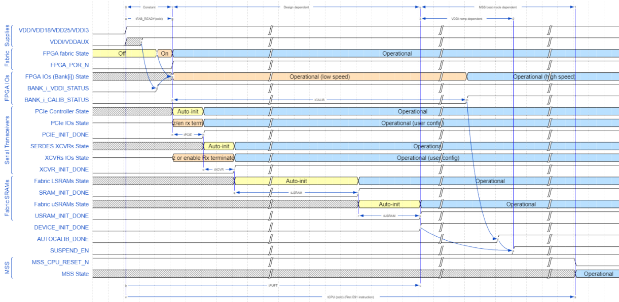
Figure 4-12. Cold Reset Timing (RTPFS460ZT and RTPFS160ZT)
