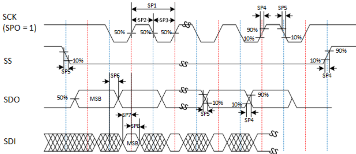
Figure 4-16. SPI Timing for a Single Frame Transfer in Motorola Mode (SPH = 1)
