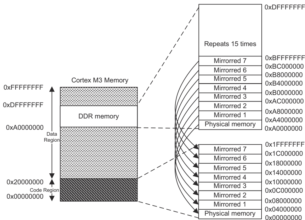
Figure 8 • Cortex M3 Processor Memory Map After Remapping DDR
