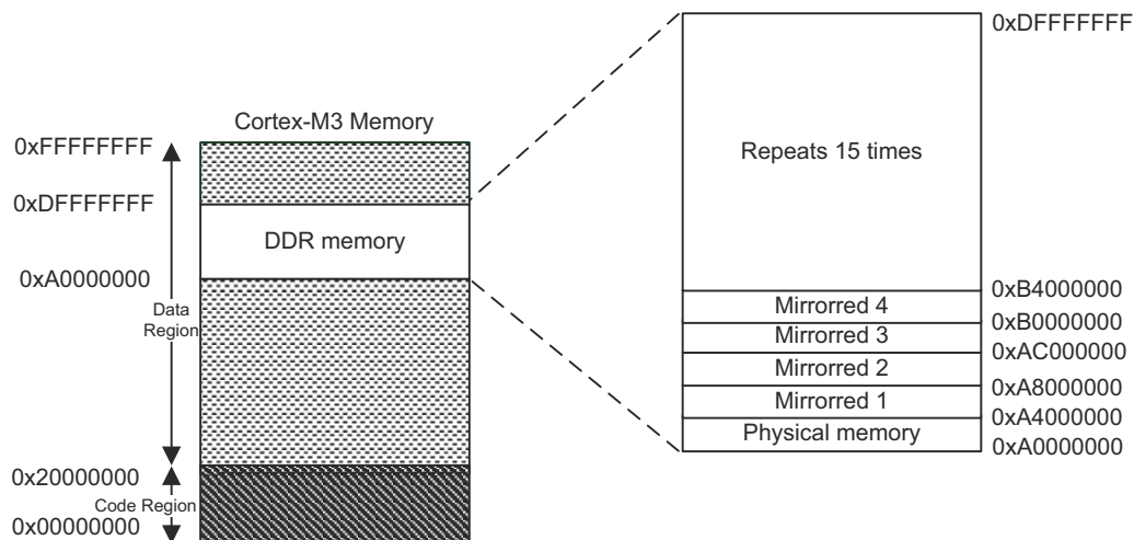
Figure 7 • Mirroring of DDR
