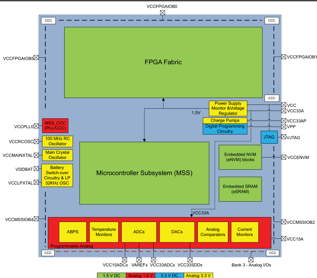
Figure 1 • SmartFusion Power System
