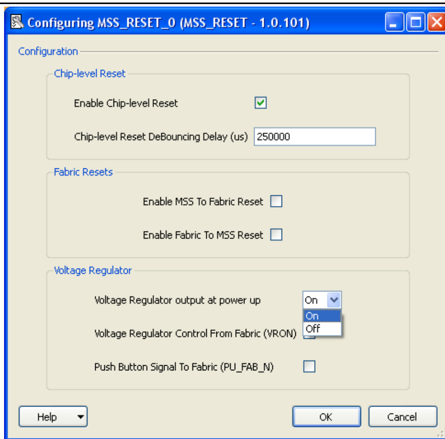
Figure 2 • Voltage Regulator Output Configuration
