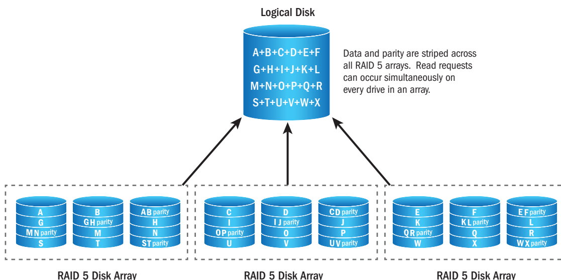
Figure 7-9. RAID 50 Array – 3 Legs
