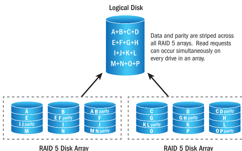
Figure 7-8. RAID 50 Array – 2 Legs
