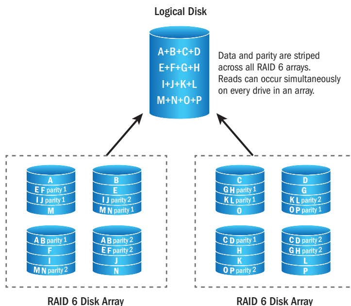
Figure 7-10. RAID 60 Array – 2 Legs
