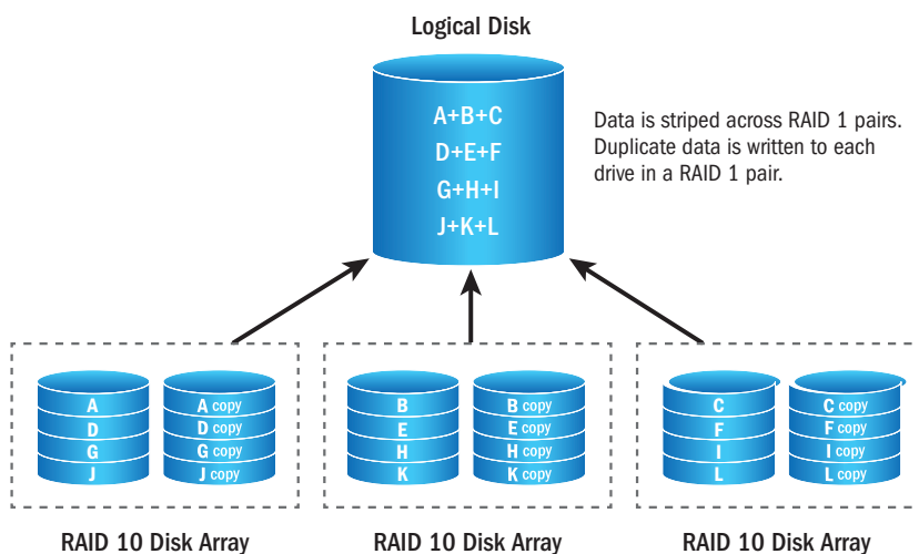
Figure 7-7. RAID 10 Array – 3 Legs
