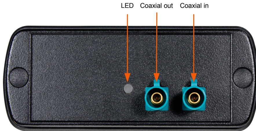
Figure 3.1 Coaxial Electrical Panel
