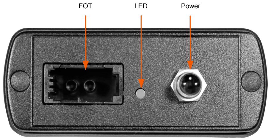
Figure 3.2 Optical Panel
