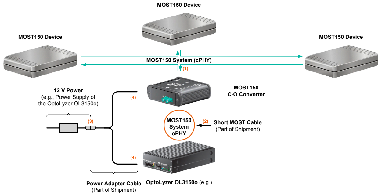
Figure 5.1 Typical Use Case: Connection Diagram
