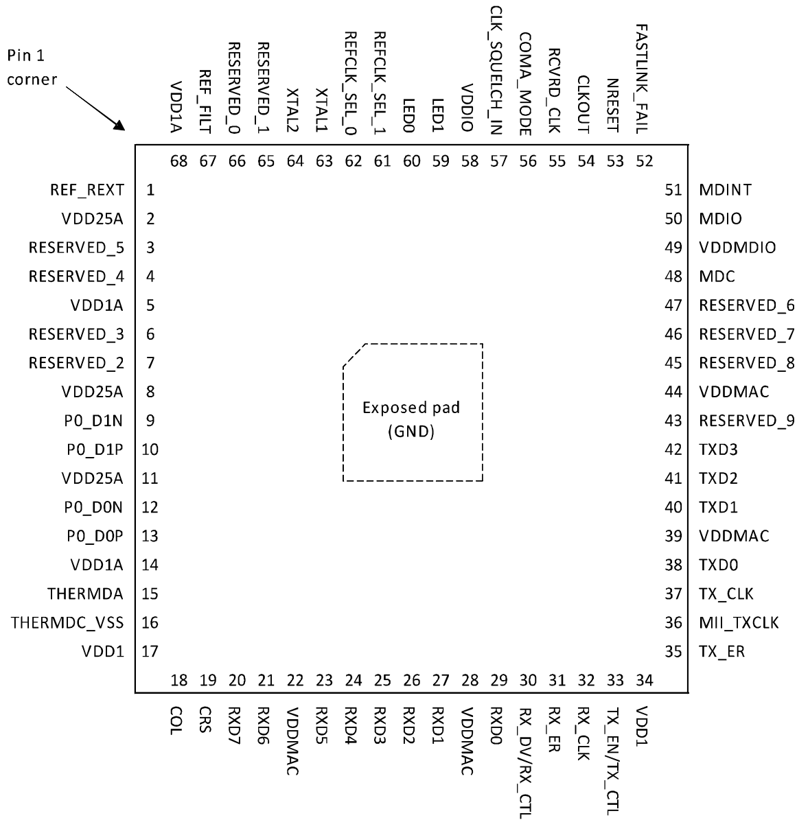
FIGURE 3-1: PIN DIAGRAM
