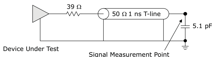
FIGURE 6-2: TEST CIRCUIT FOR RECOVERED CLOCK OUTPUTS SIGNAL
