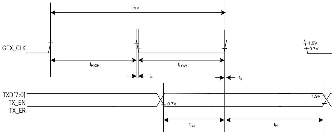
FIGURE 6-4: GMII TRANSMIT TIMING
