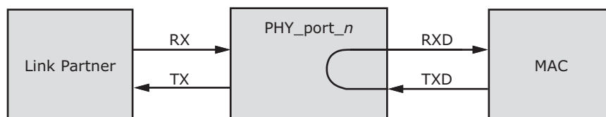
FIGURE 3-18: NEAR-END LOOPBACK DIAGRAM
