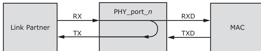
FIGURE 3-17: FAR-END LOOPBACK DIAGRAM
