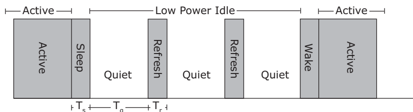
FIGURE 3-7: LOW POWER IDLE OPERATION
