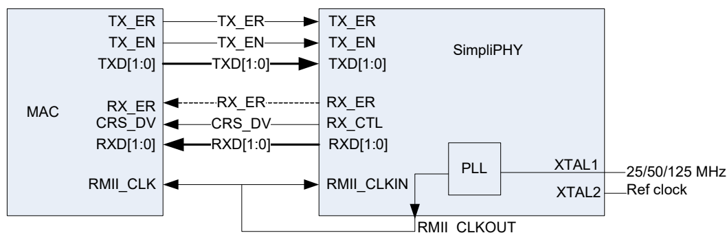
FIGURE 3-5: MODE 2
