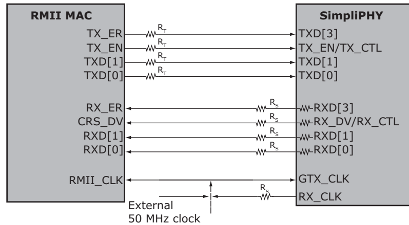
FIGURE 3-3: RMII MAC INTERFACE
