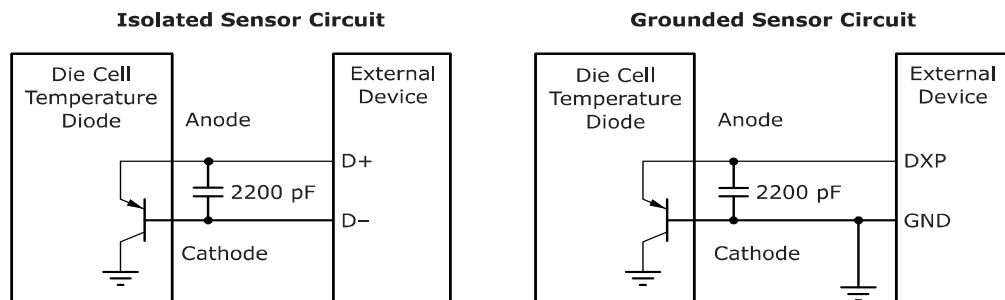
FIGURE 6-1: THERMAL DIODE
