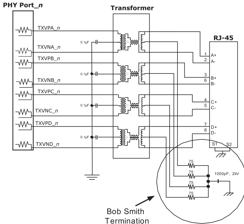
FIGURE 3-6: CAT5 MEDIA INTERFACE
