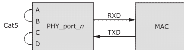
FIGURE 3-19: CONNECTOR LOOPBACK DIAGRAM
