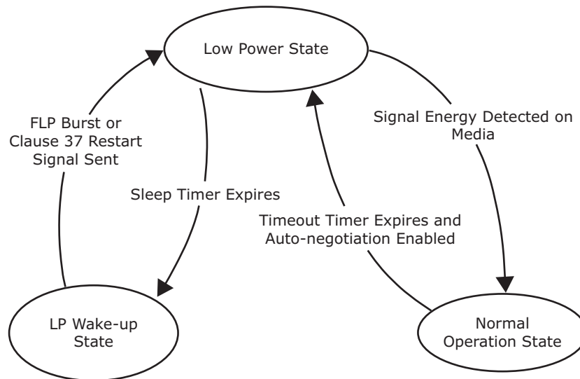
FIGURE 3-11: ACTIPHY STATE DIAGRAM
