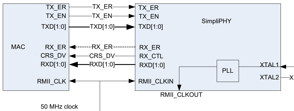
FIGURE 3-4: MODE 1
