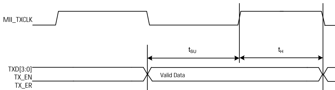
FIGURE 6-7: MII RECEIVE TIMING
