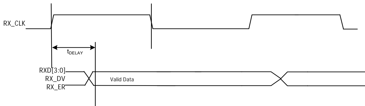
FIGURE 6-6: MII RECEIVE TIMING
