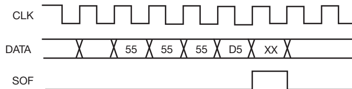
FIGURE 3-16: SOF INDICATION
