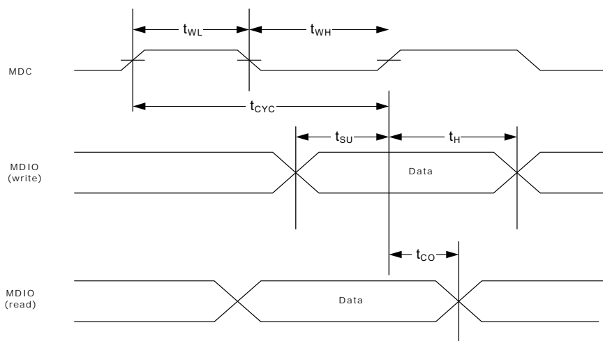
FIGURE 6-12: SERIAL MANAGEMENT INTERFACE TIMING
