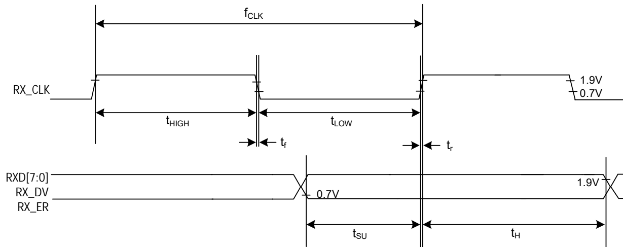
FIGURE 6-5: GMII RECEIVE TIMING
