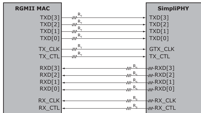
FIGURE 3-1: RGMII MAC INTERFACE
