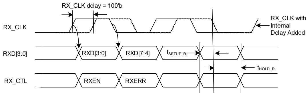
FIGURE 6-10: COMPENSATED OUTPUT RGMII TIMING
