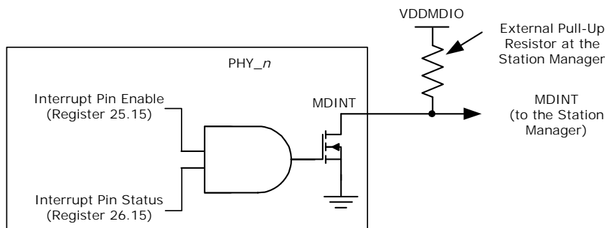
FIGURE 3-14: MDINT CONFIGURED AS AN OPEN-DRAIN (ACTIVE-LOW) PIN
