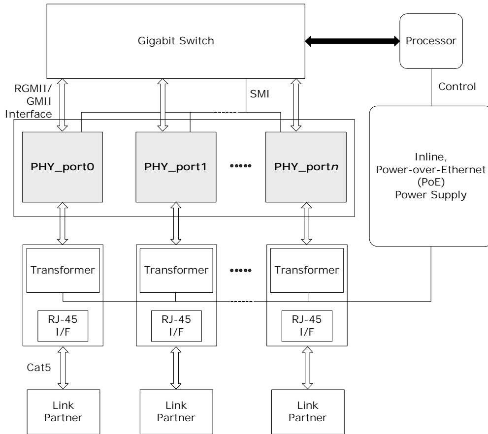
FIGURE 3-10: INLINE-POWERED ETHERNET SWITCH DIAGRAM
