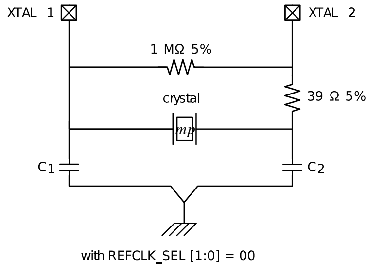
FIGURE 3-8: XTAL REFERENCE CLOCK
