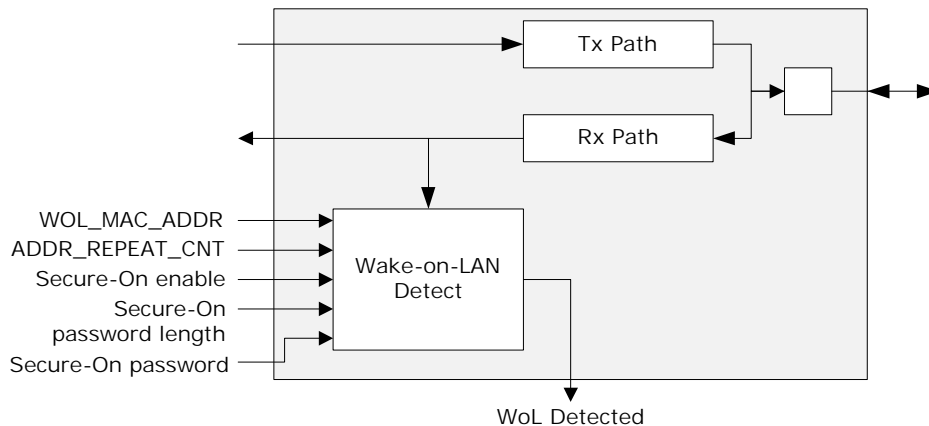
FIGURE 3-15: WAKE-ON-LAN FUNCTIONALITY
