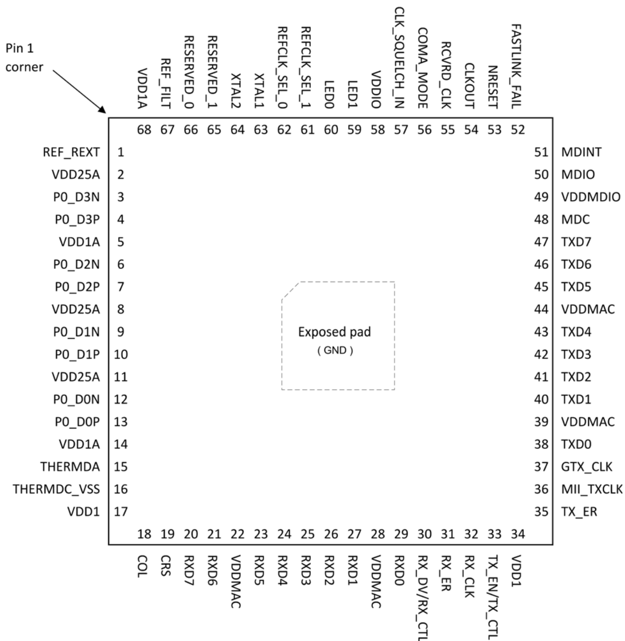
FIGURE 1-1: PIN DIAGRAM
