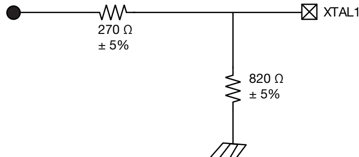
FIGURE 3-9: EXTERNAL 3.3V REFERENCE CLOCK
