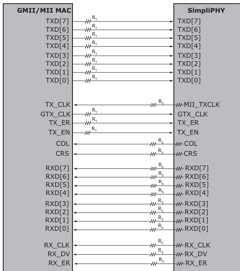
FIGURE 3-2: GMII/MII MAC INTERFACE
