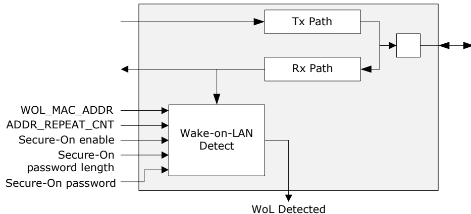
FIGURE 5-15: WAKE-ON-LAN FUNCTIONALITY
