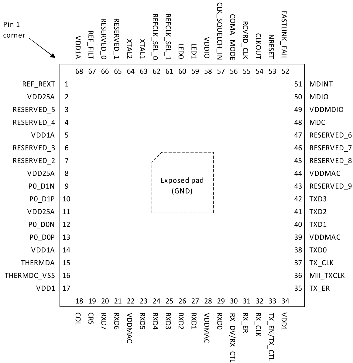
FIGURE 3-1: PIN DIAGRAM
