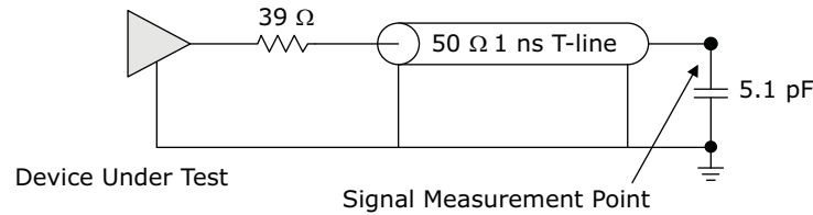
FIGURE 7-2: TEST CIRCUIT FOR RECOVERED CLOCK OUTPUTS SIGNAL
