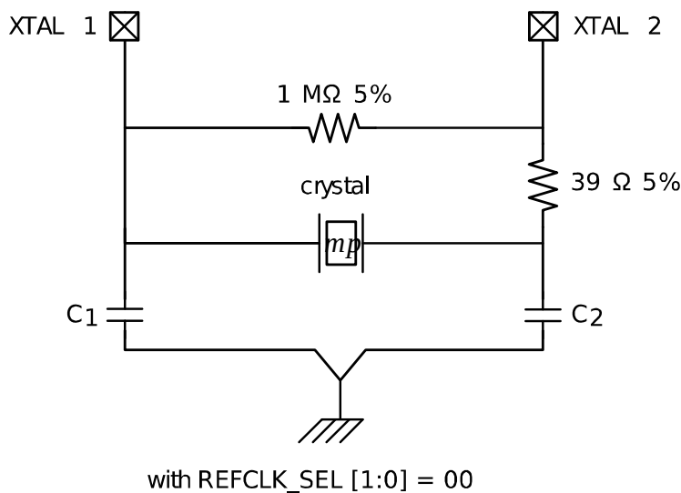
FIGURE 4-8: XTAL REFERENCE CLOCK
