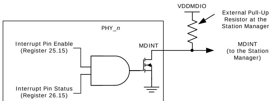
FIGURE 4-14: MDINT CONFIGURED AS AN OPEN-DRAIN (ACTIVE-LOW) PIN
