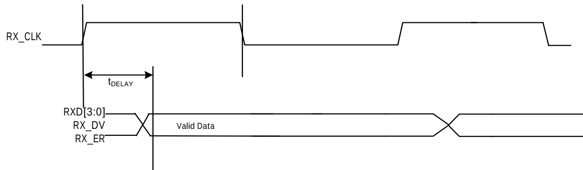
FIGURE 7-4: MII RECEIVE TIMING
