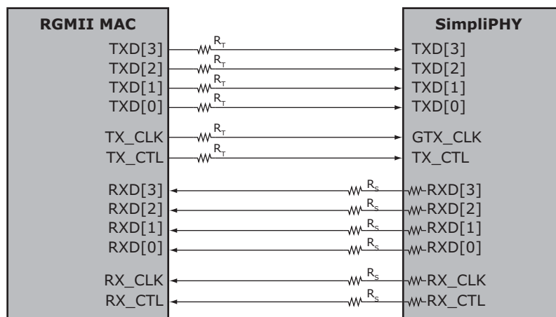
FIGURE 4-1: RGMII MAC INTERFACE
