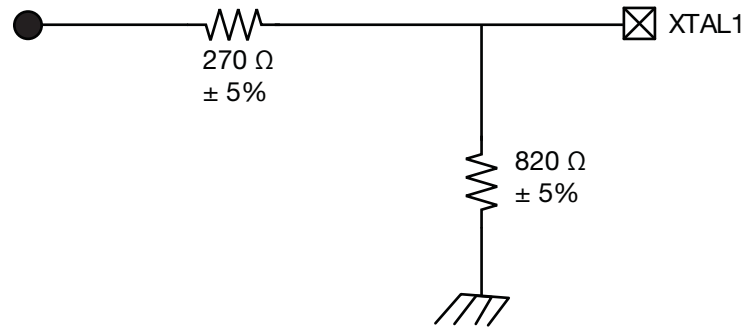
FIGURE 4-9: EXTERNAL 3.3V REFERENCE CLOCK
