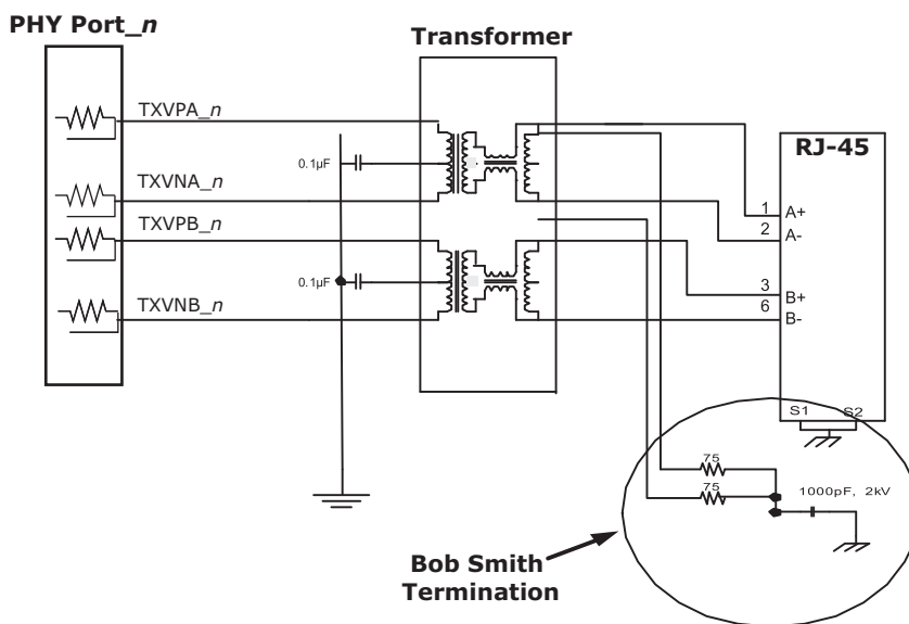
FIGURE 4-6: CAT5 MEDIA INTERFACE
