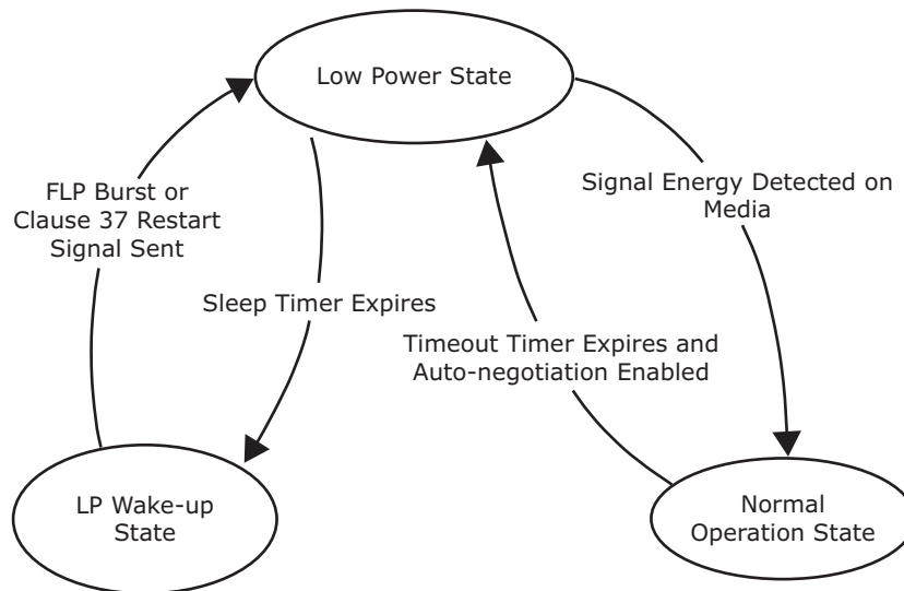
FIGURE 4-11: ACTIPHY STATE DIAGRAM
