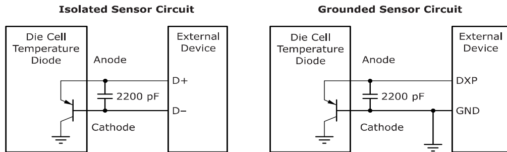
FIGURE 7-1: THERMAL DIODE
