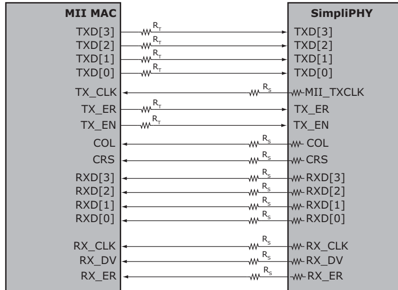
FIGURE 4-2: MII MAC INTERFACE
