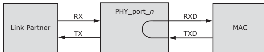
FIGURE 4-18: NEAR-END LOOPBACK DIAGRAM
