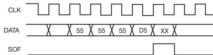
FIGURE 4-16: SOF INDICATION
