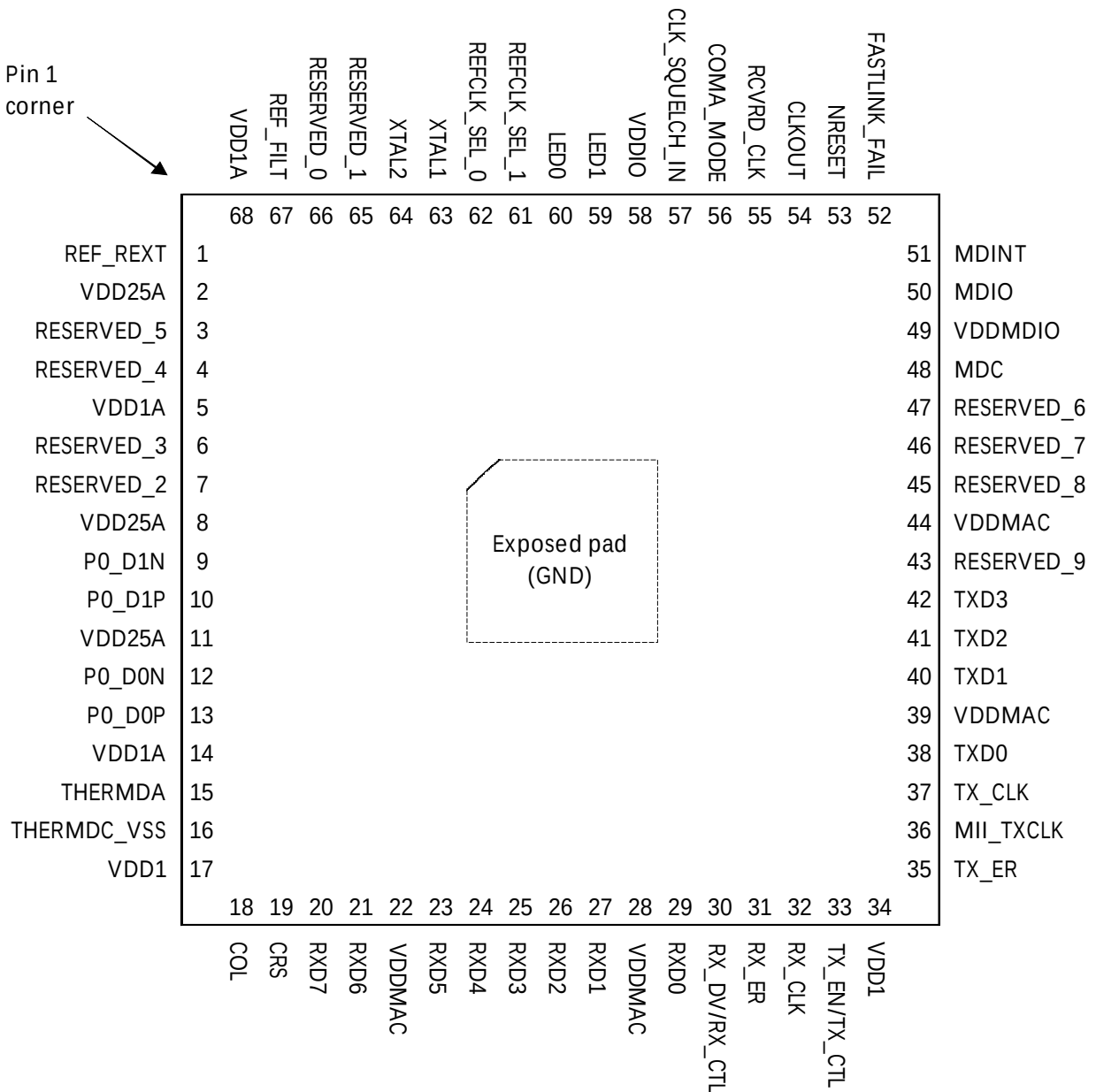
FIGURE 2-1: PIN DIAGRAM
