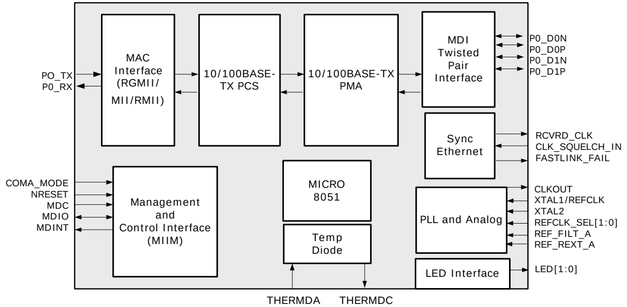
FIGURE 1-1: BLOCK DIAGRAM
