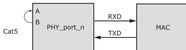
FIGURE 4-19: CONNECTOR LOOPBACK DIAGRAM
