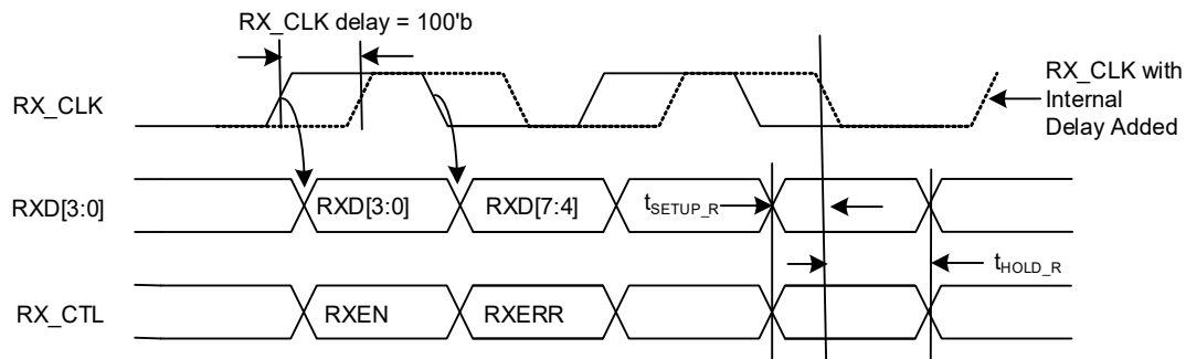
FIGURE 7-8: COMPENSATED OUTPUT RGMII TIMING
