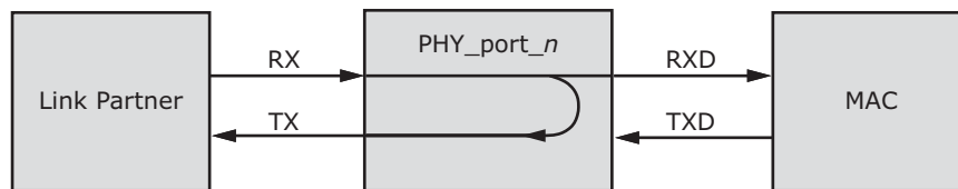
FIGURE 4-17: FAR-END LOOPBACK DIAGRAM
