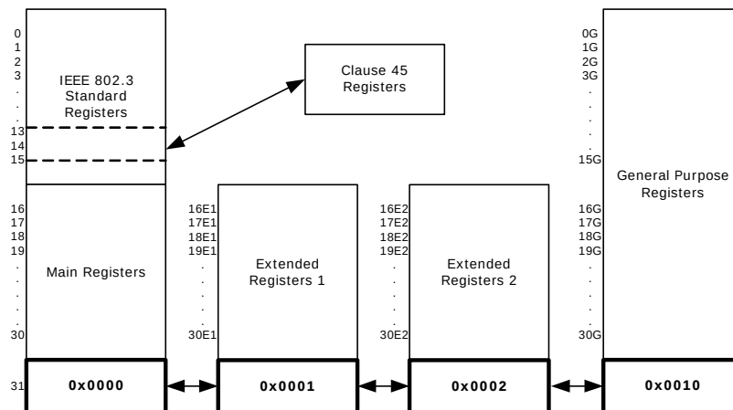
FIGURE 5-1: REGISTER SPACE DIAGRAM
