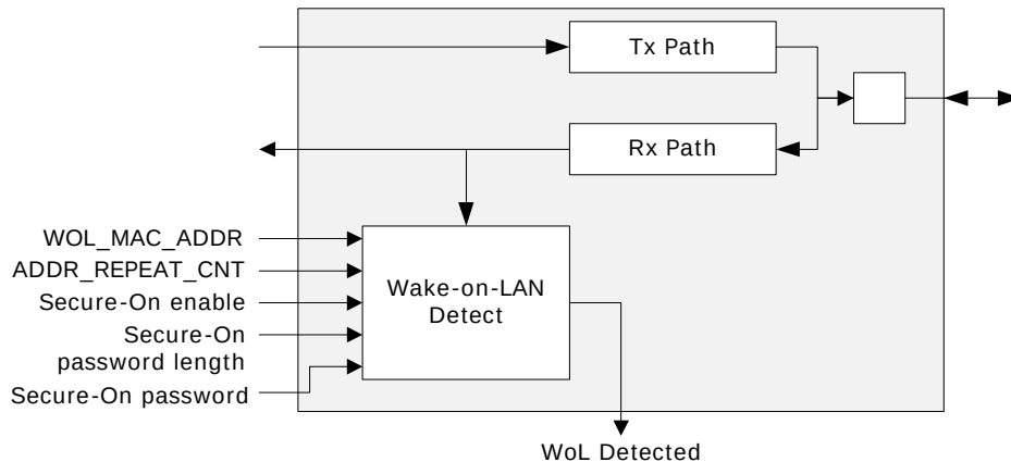
FIGURE 4-15: WAKE-ON-LAN FUNCTIONALITY
