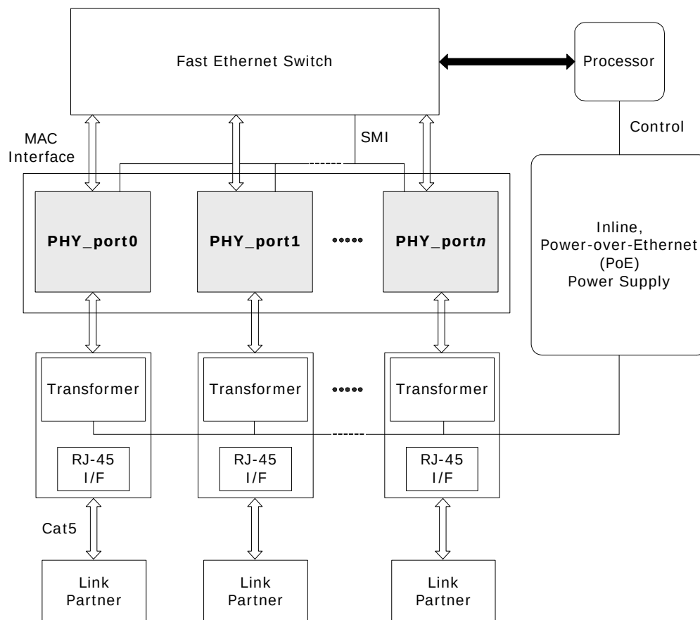
FIGURE 4-10: INLINE-POWERED ETHERNET SWITCH DIAGRAM
