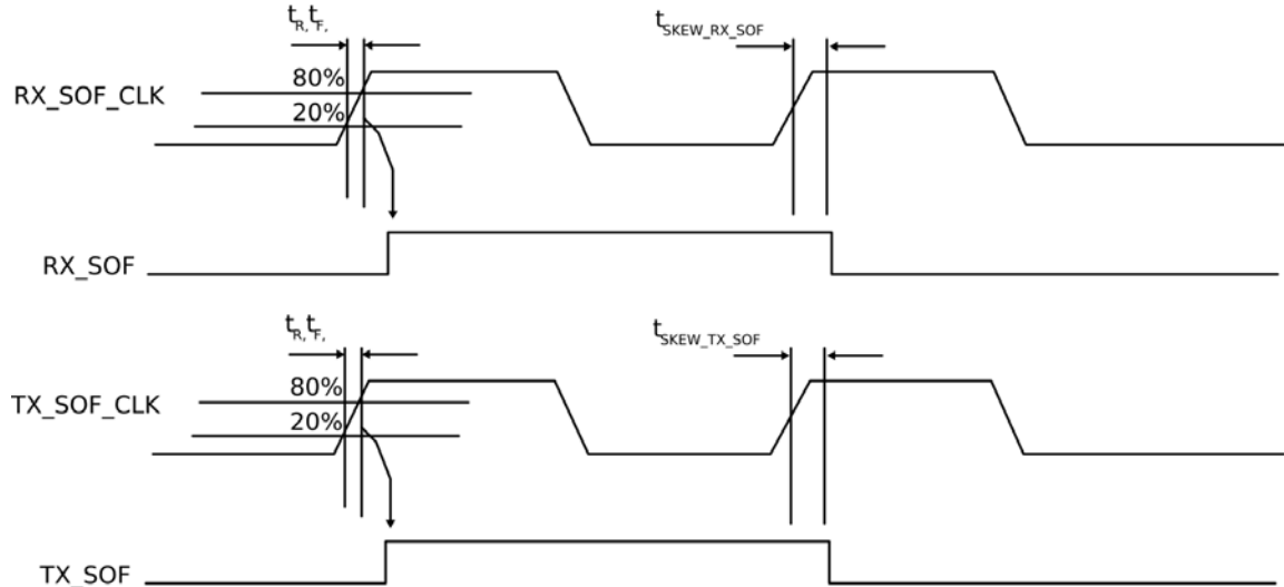
FIGURE 7-9: SOF INDICATION TIMING
