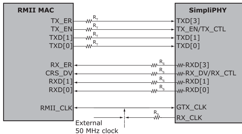
FIGURE 4-3: RMII MAC INTERFACE
