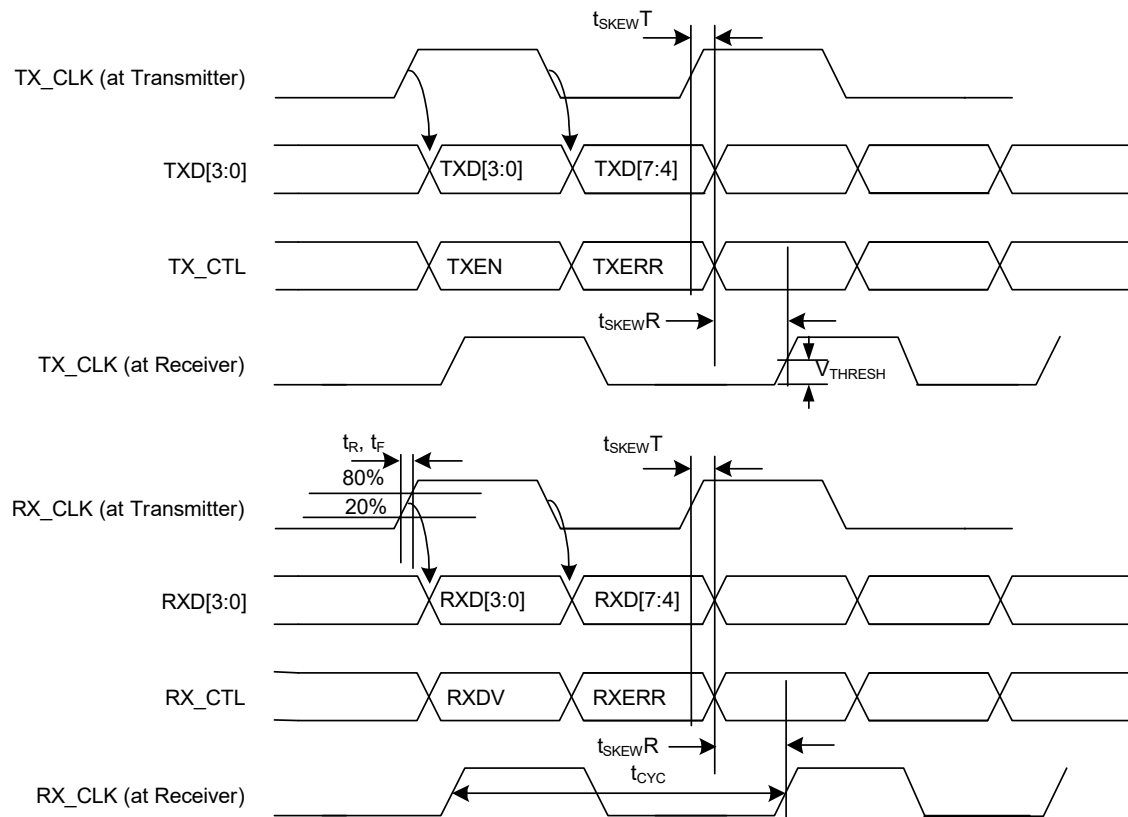
FIGURE 7-6: UNCOMPENSATED RGMII TIMING
