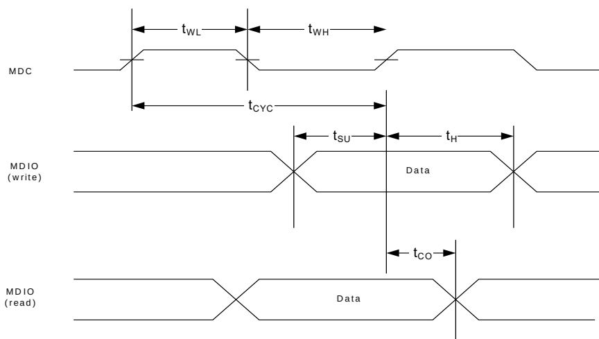
FIGURE 7-10: SERIAL MANAGEMENT INTERFACE TIMING
